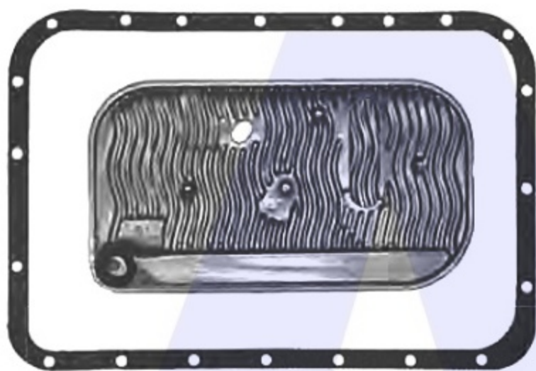
ALLISON AT-540 Pan Gasket AT545.GAS01 Filter AT545.FIL01
