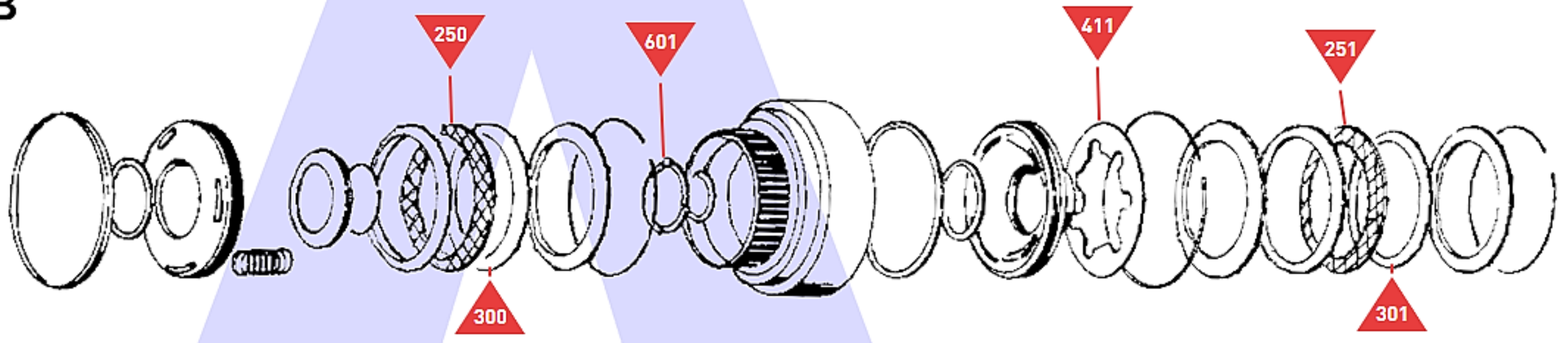
Direct/Reverse Clutch and Forward Clutch Assembly
