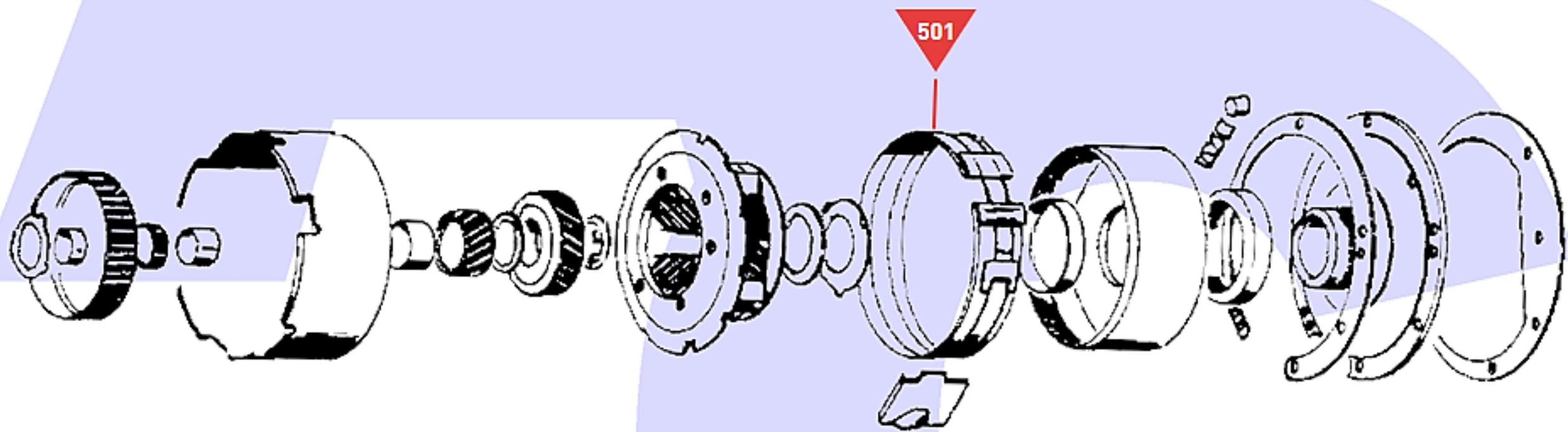
Planetary Assembly, Reverse/Low Band and Low One Way Clutch
