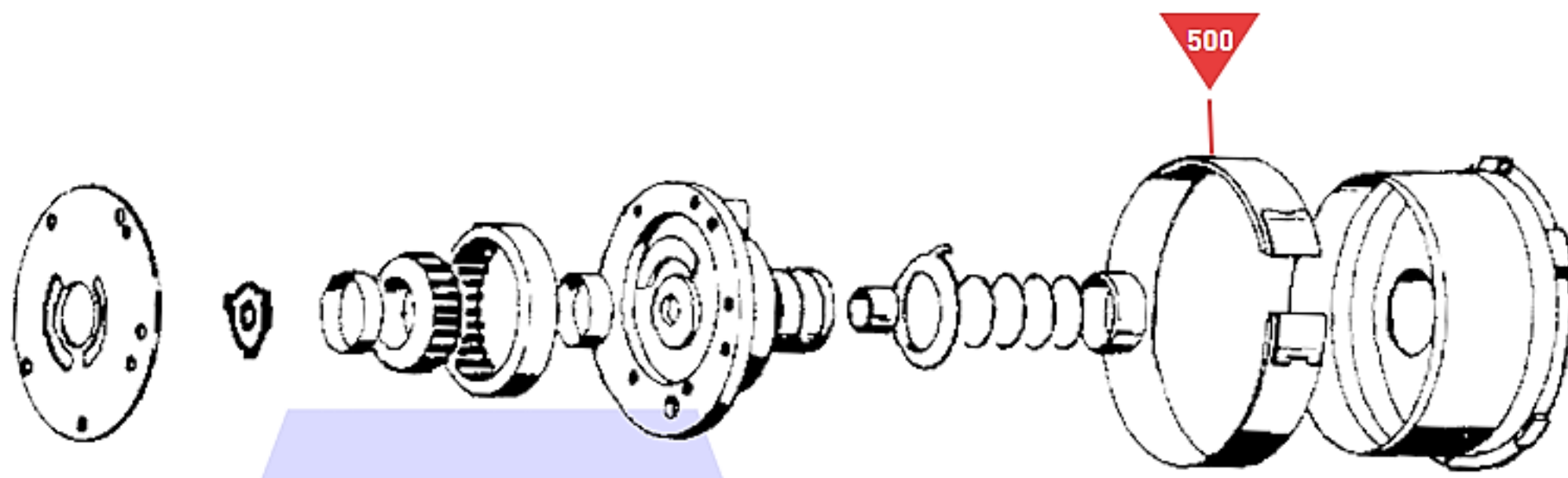
Oil Pump, Intermediate Band and Direct/Reverse Drum
