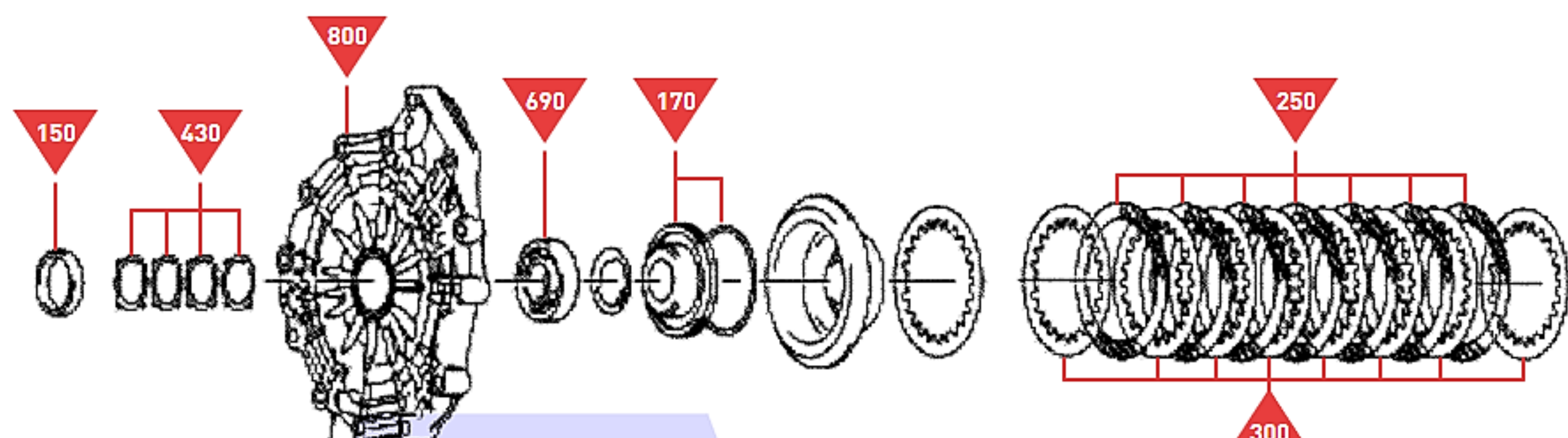
Front Cover & Forward Clutch
