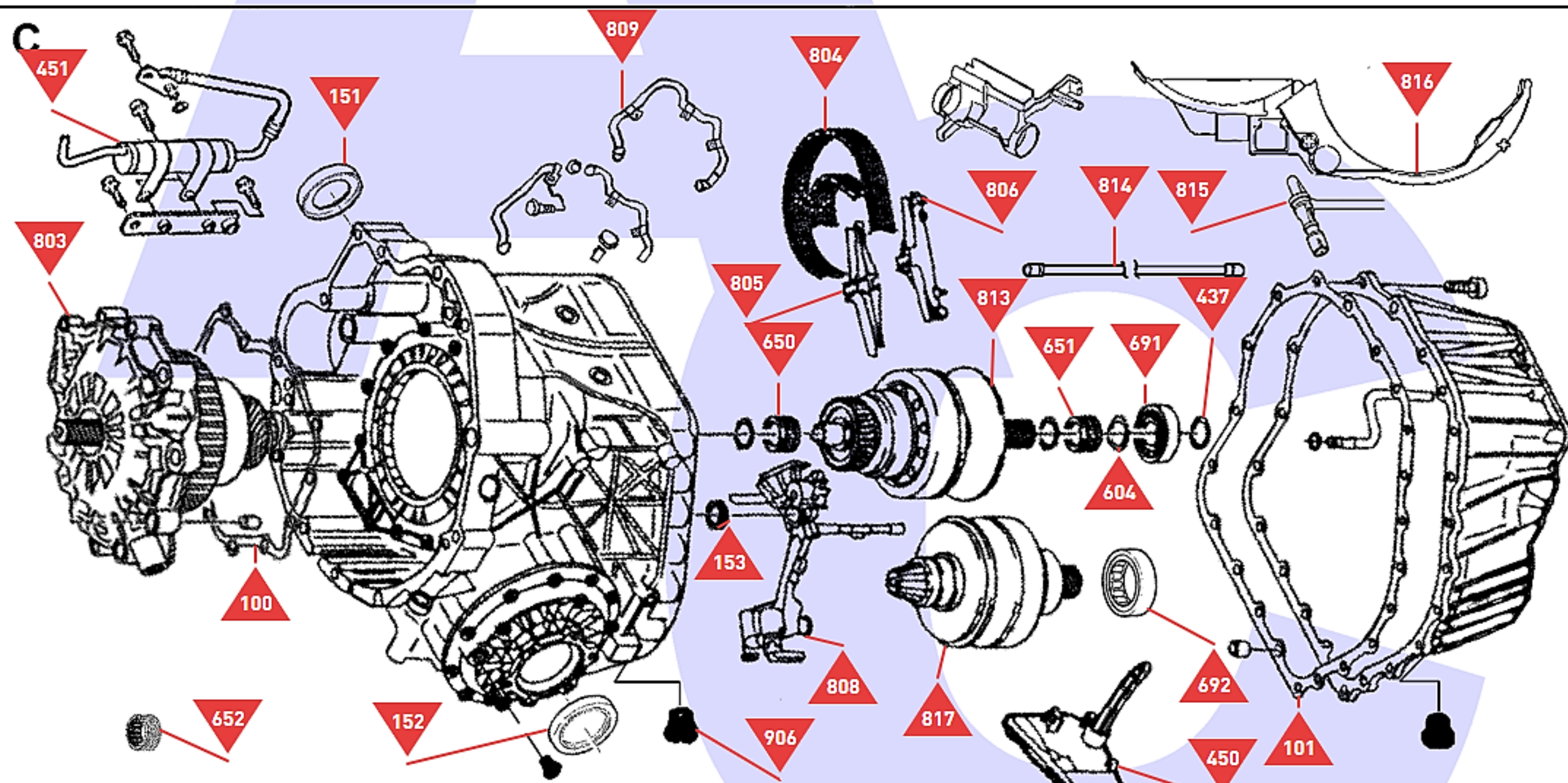
Main Case & Internal Components
