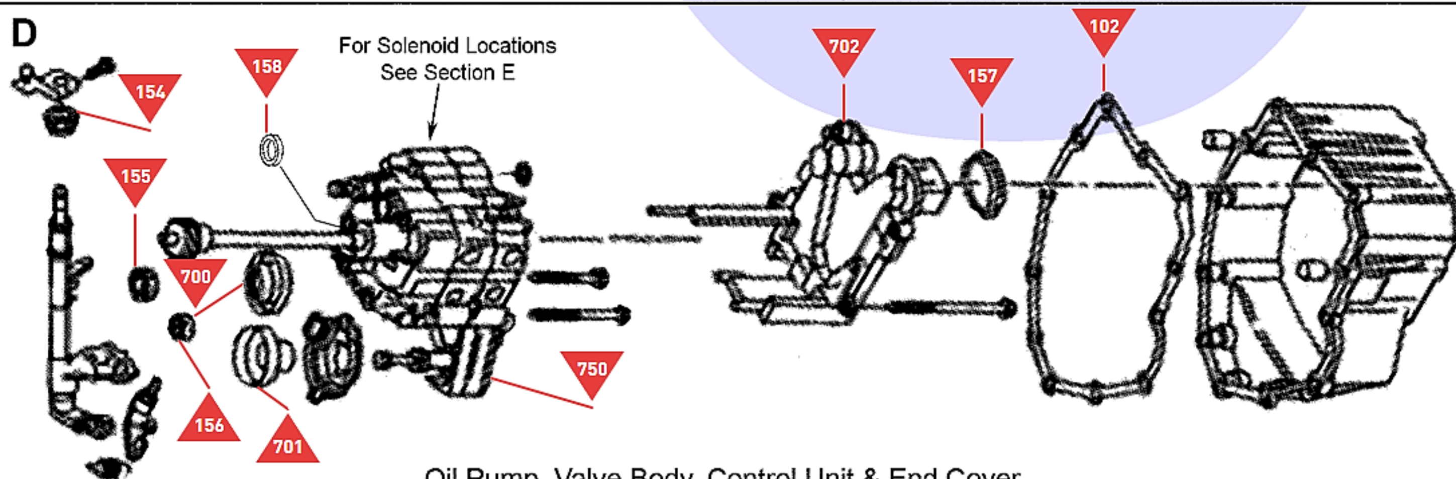
Oil Pump, Valve Body, Control Unit & End Cover
