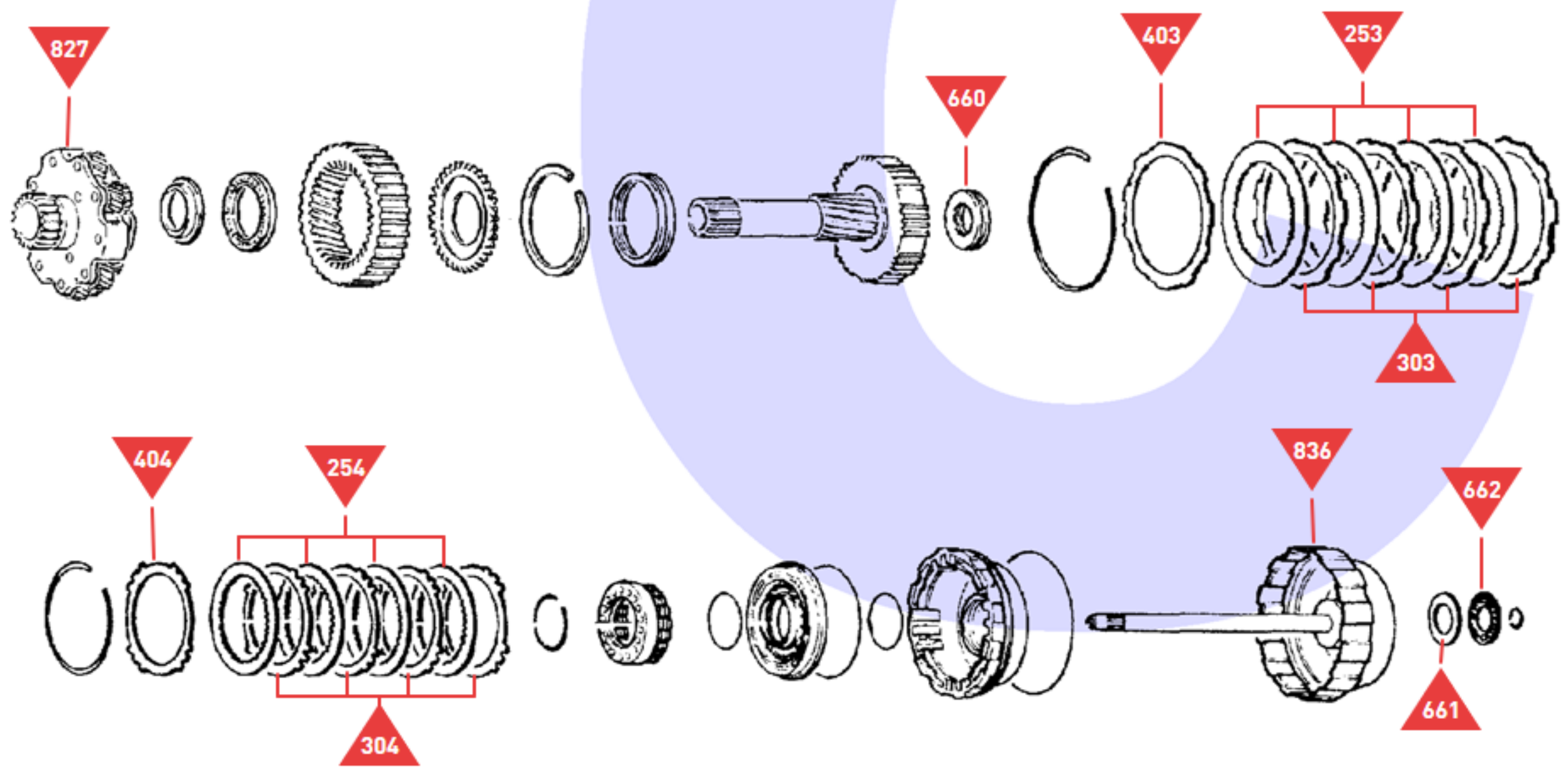
'P1' Planetary, 'C1' & 'C2' Clutches
