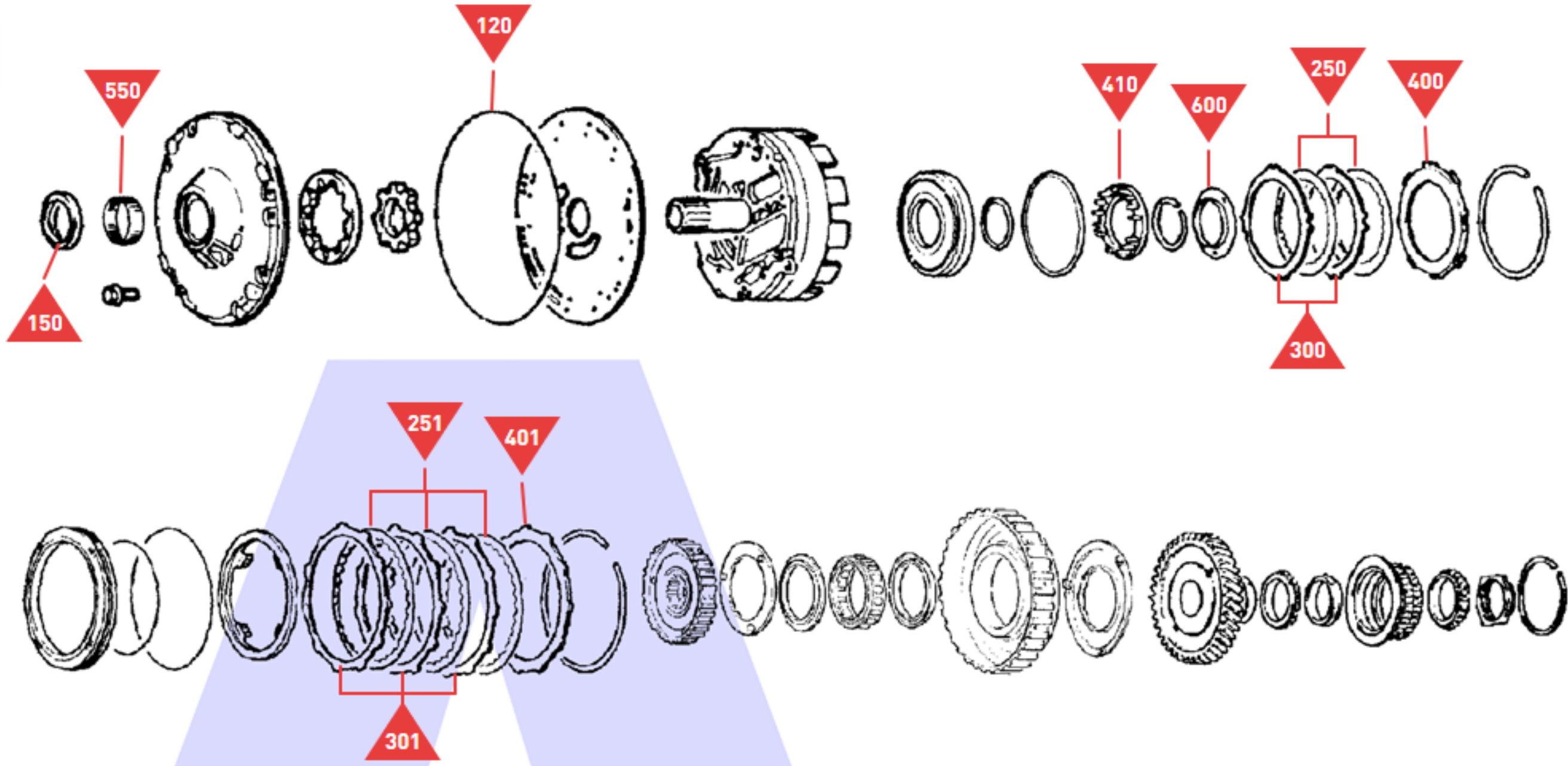
Pump, 'B1' & 'B2' Brakes, Intermediate Drive Gear
