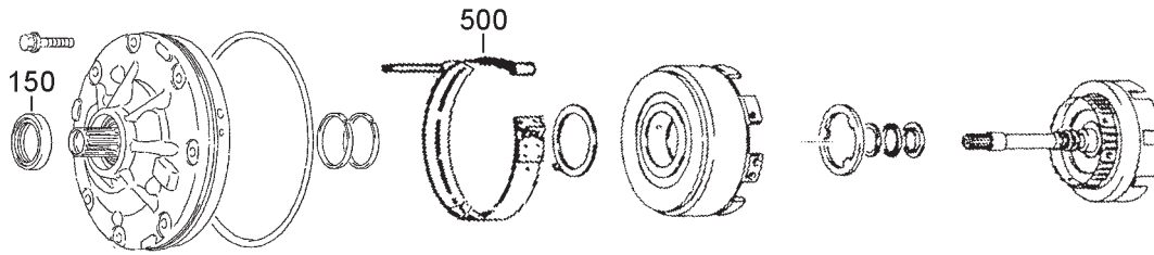
Oil Pump, Brake Band, Direct and Forward Clutches
