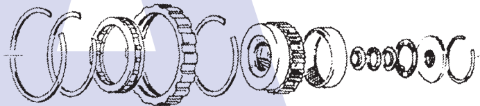
One Way Clutch and Rear Planetary
