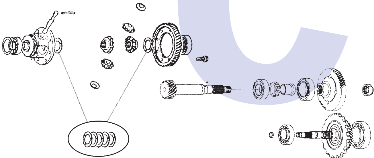
Differential, Transfer Gears and Output
