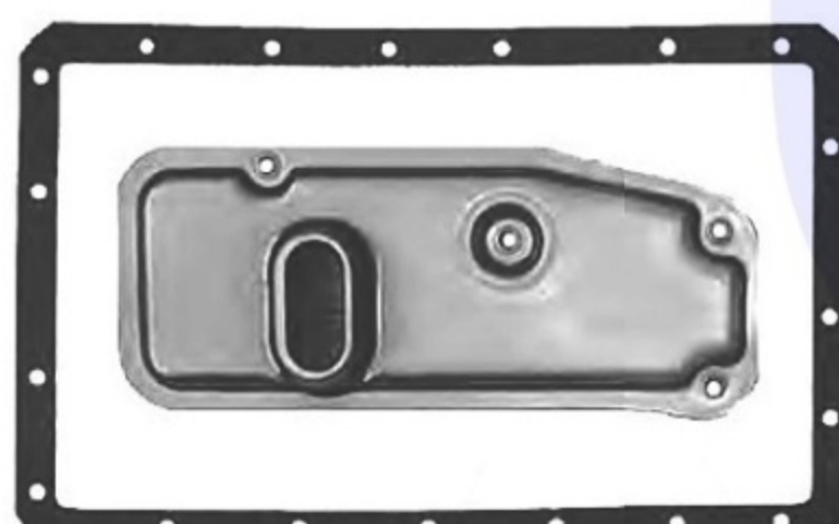
AISIN WARNER A343F Pan Gasket A340.GAS01 Filter A343.FIL03 Filter has 25mm Pick Up & 2 Valve Body Feed Holes
