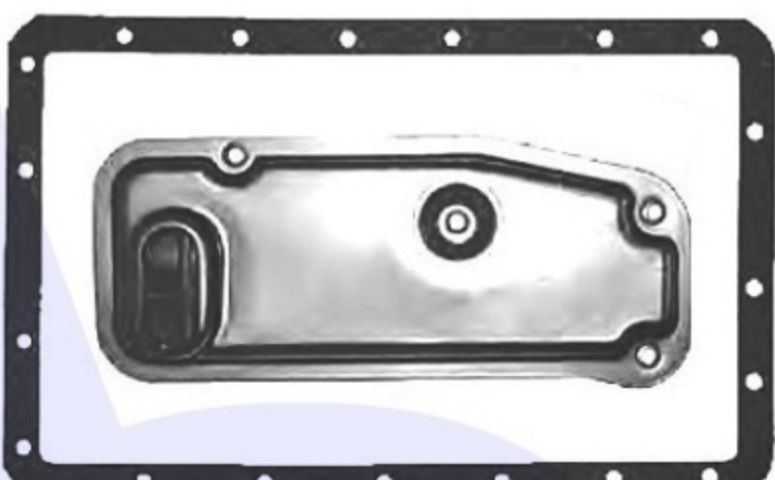
AISIN WARNER A343E, A343F 19mm Pick Up Pan Gasket A340.GAS01 Filter A343.FIL01 Filter has 19mm Pick Up
