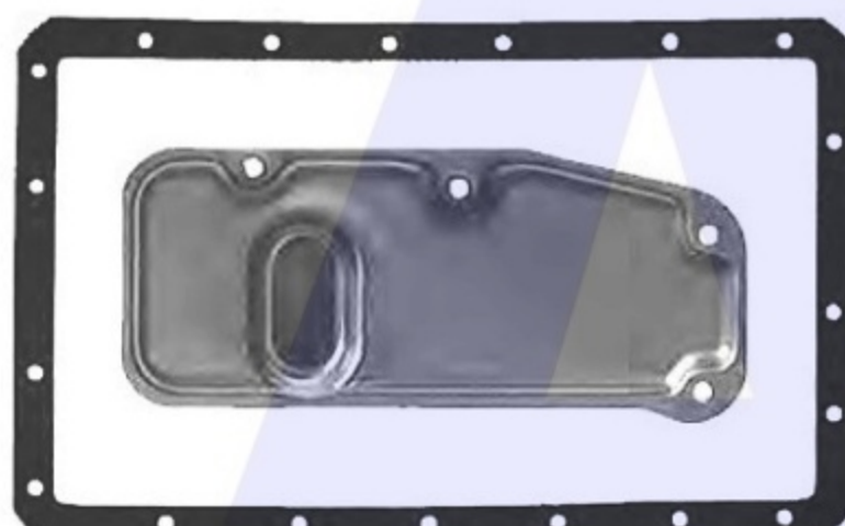
AISIN WARNER A340E, A343F Pan Gasket A340.GAS01 Filter A343.FIL02 Filter has 25mm Pick Up & 3 Valve body Feed Holes
