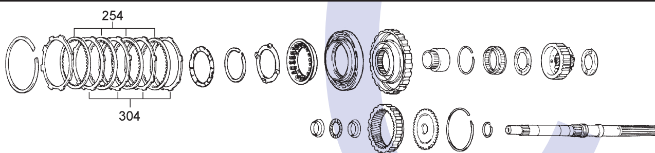
Intermediate Brake & Rear Planetary Set
