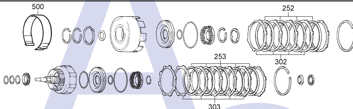
Direct & Forward Clutch Assemblies
