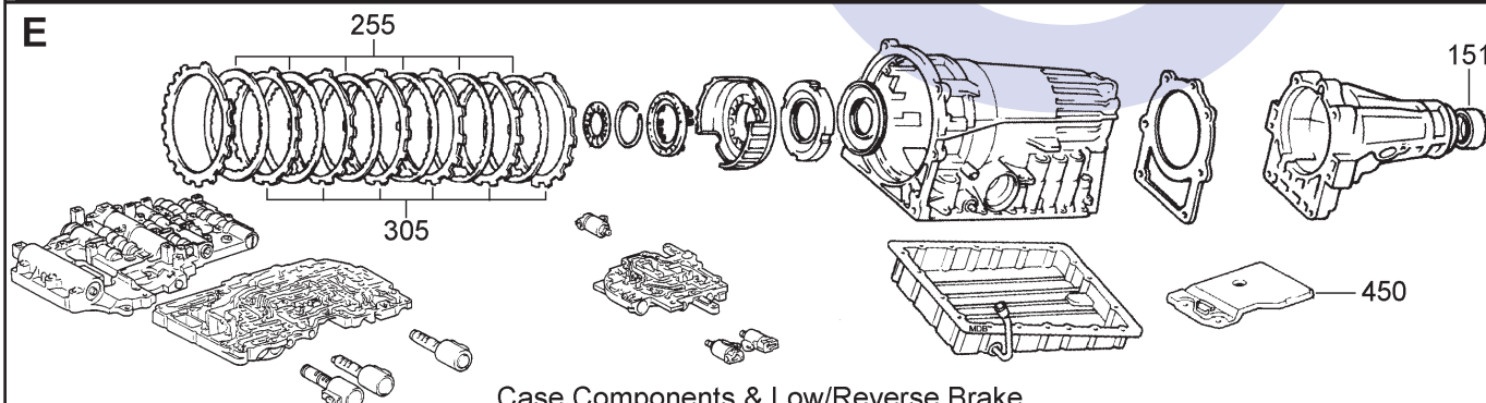
Case Components & Low/Reverse Brake
