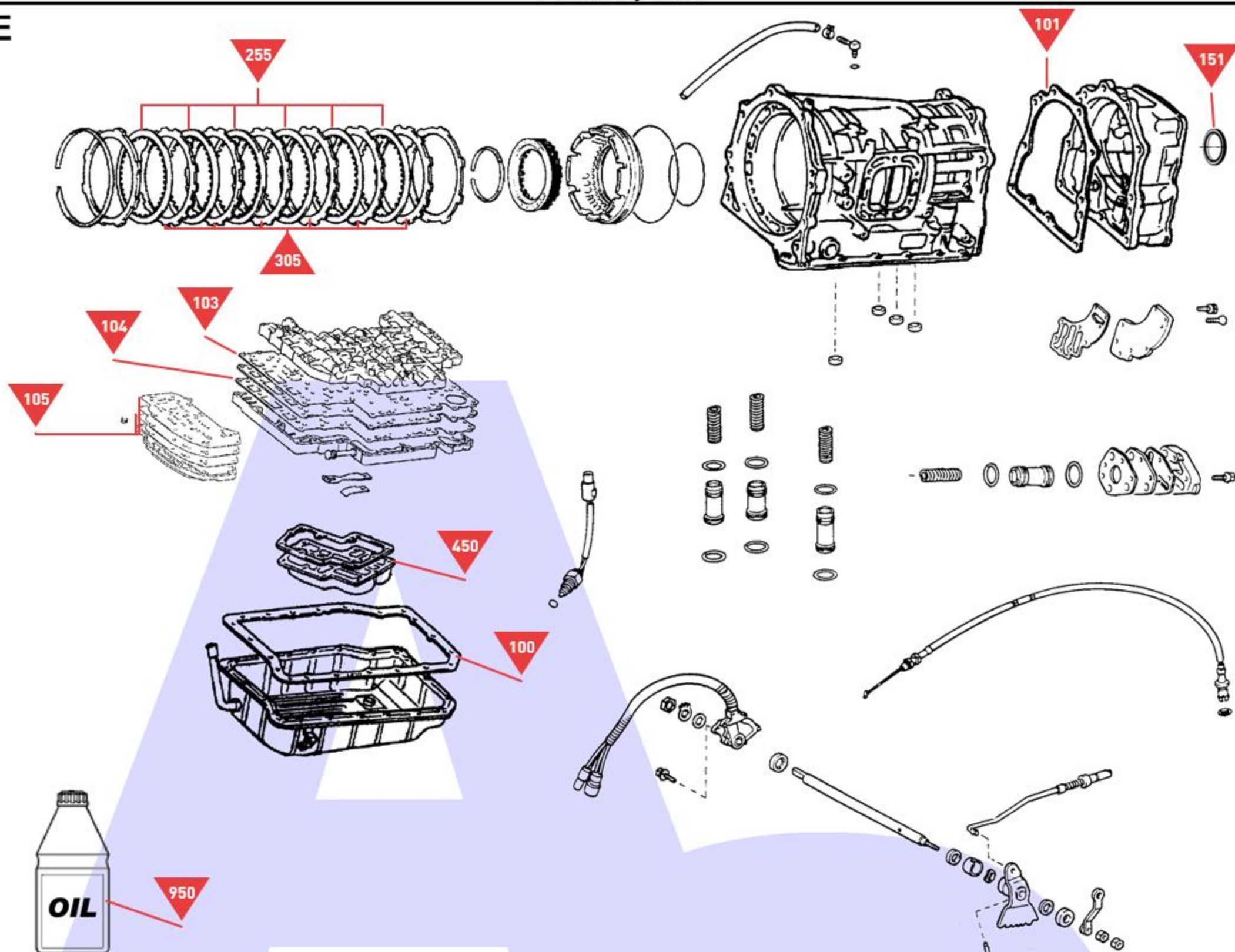
Low & Reverse Brake, Casings, Valve Body Etc.
