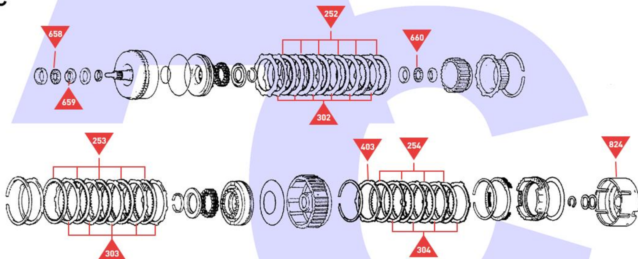
Forward, Direct & Intermediate Clutches
