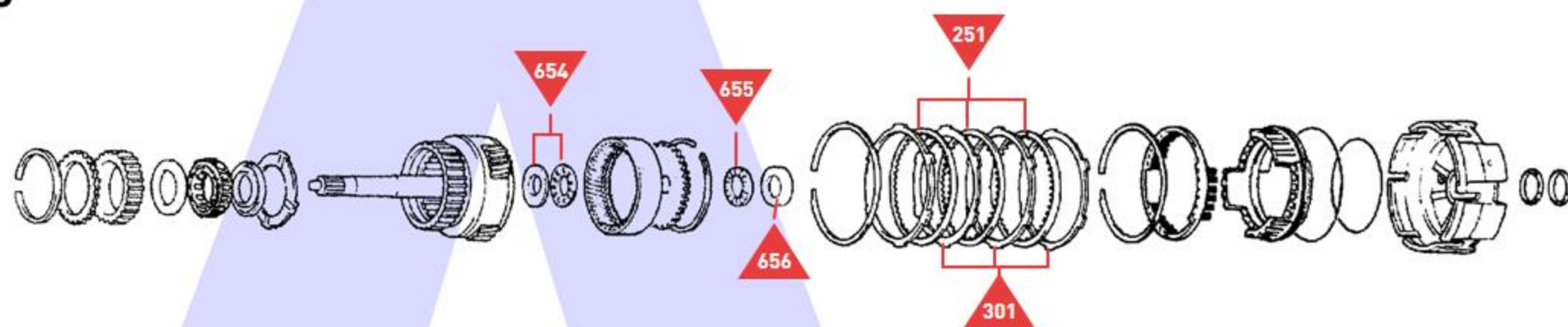
Overdrive Planet & Overdrive Brake
