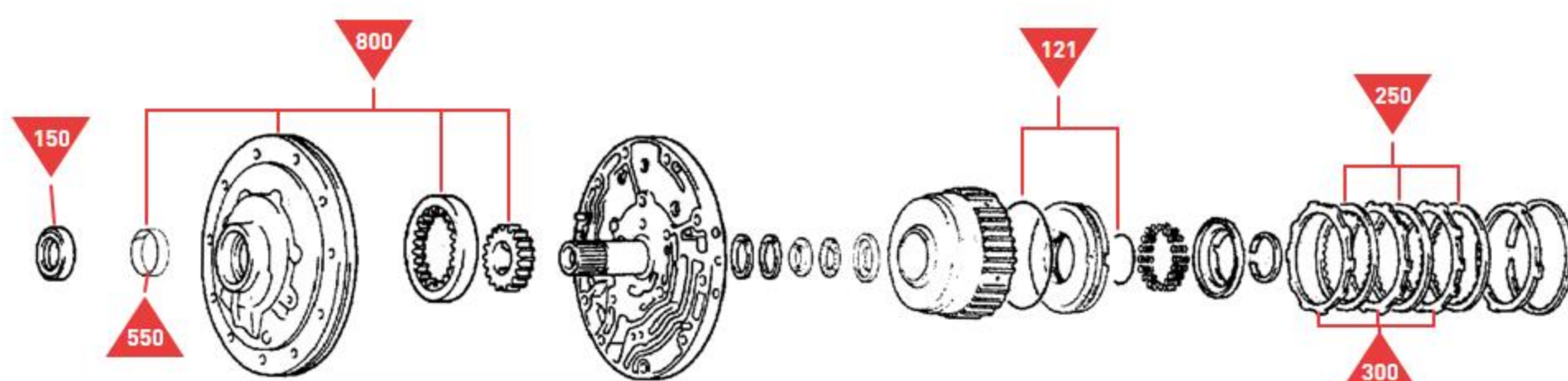
Oil Pump & Overdrive Direct Clutch
