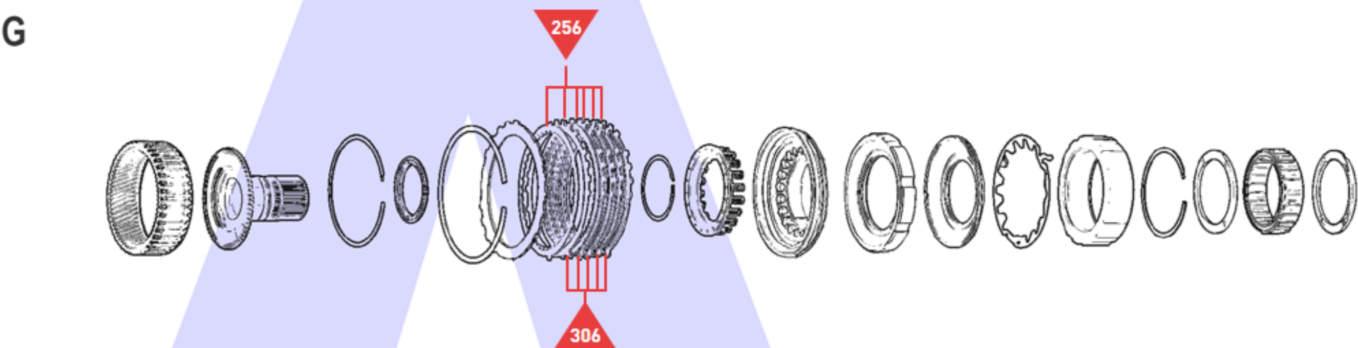
Low/Reverse Brake
