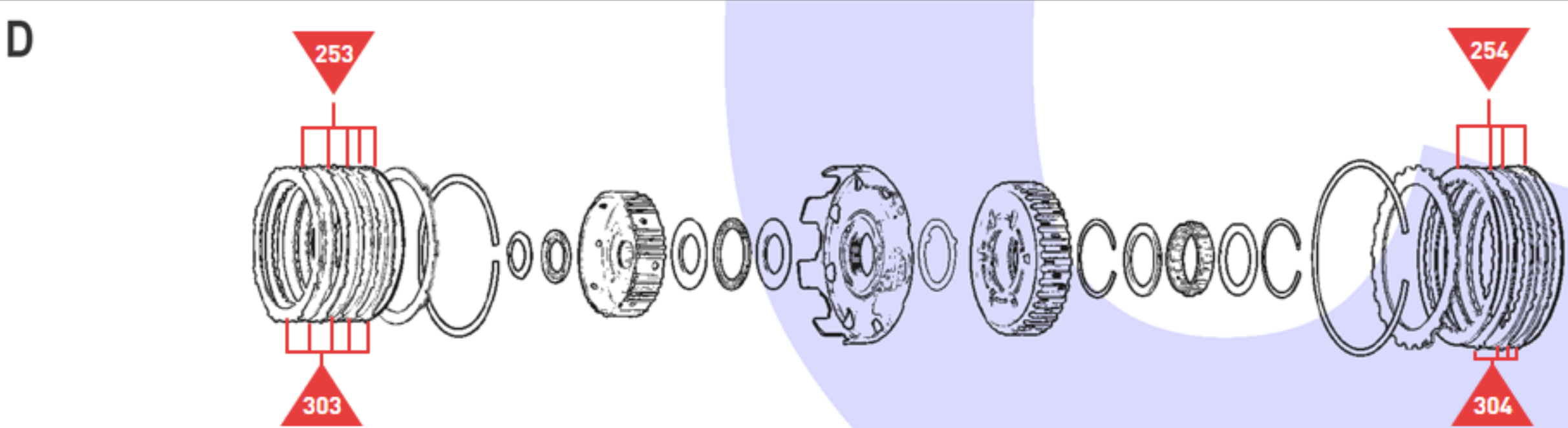
Forward Clutch
