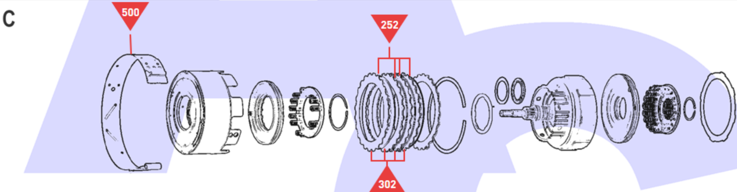
Direct Clutch
