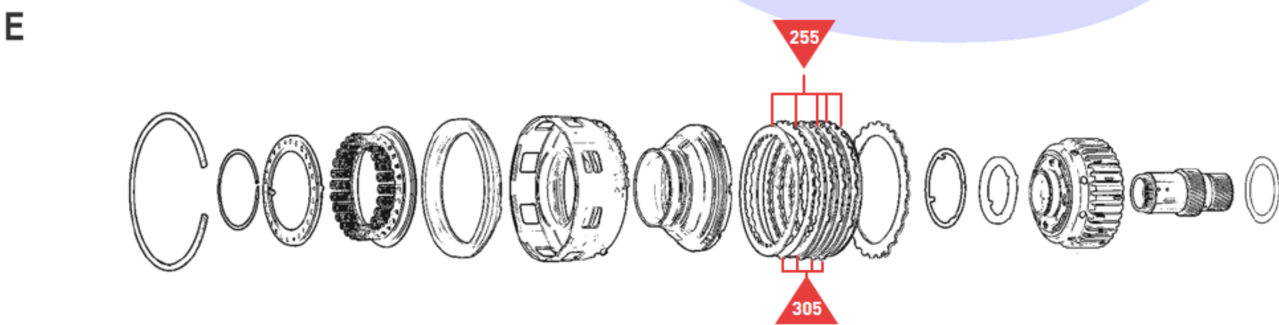
Third Brake
