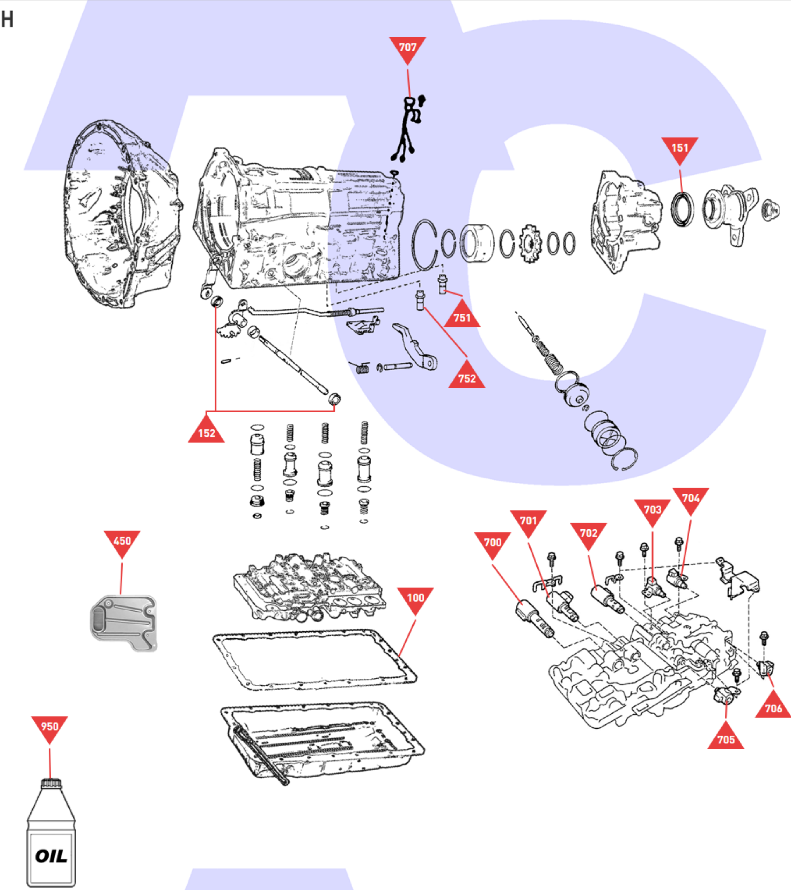
Low/Reverse Brake
