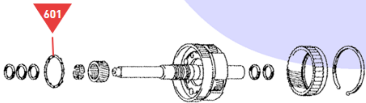
Front Planetary Assembly
