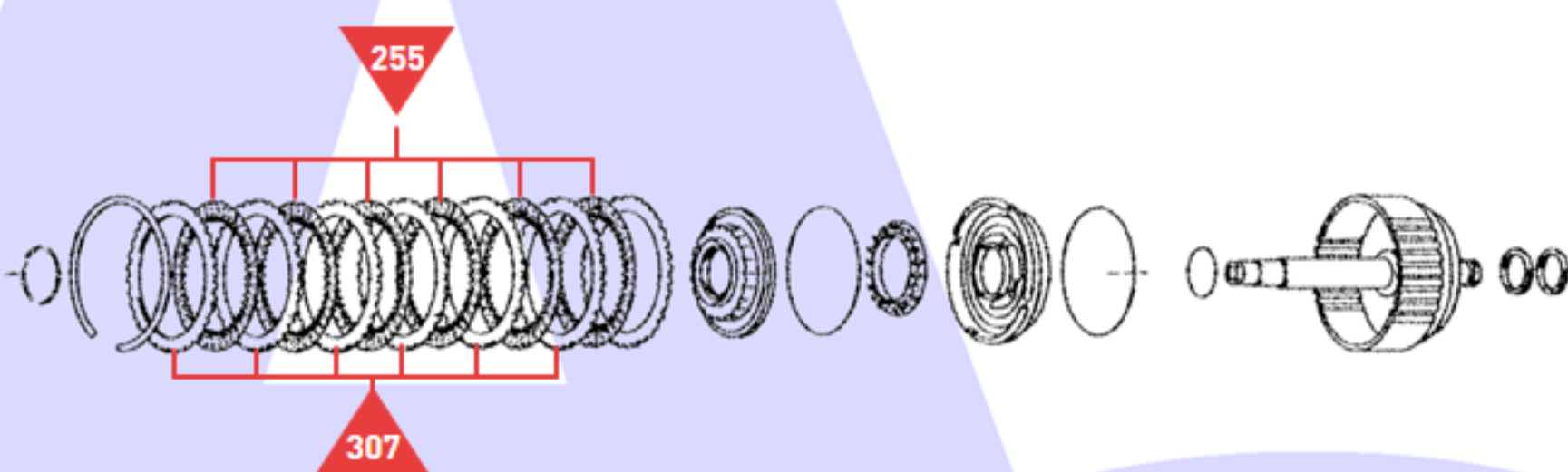
'C2' Clutch (5th, 6th, 7th, & 8th)
