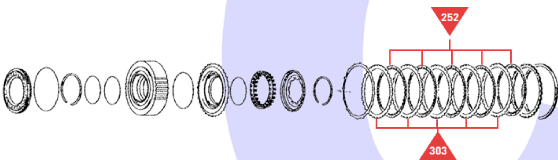
'C4' Clutch (Rev, 4th & 6th)
