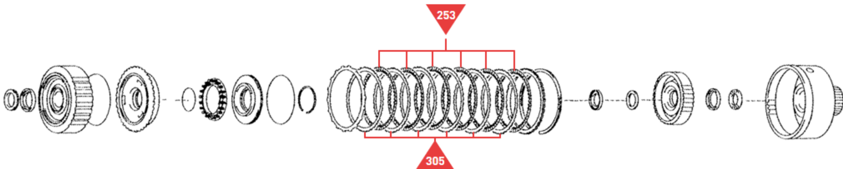
'C1' Clutch (1st, 2nd, 3rd, 4th & 5th)
