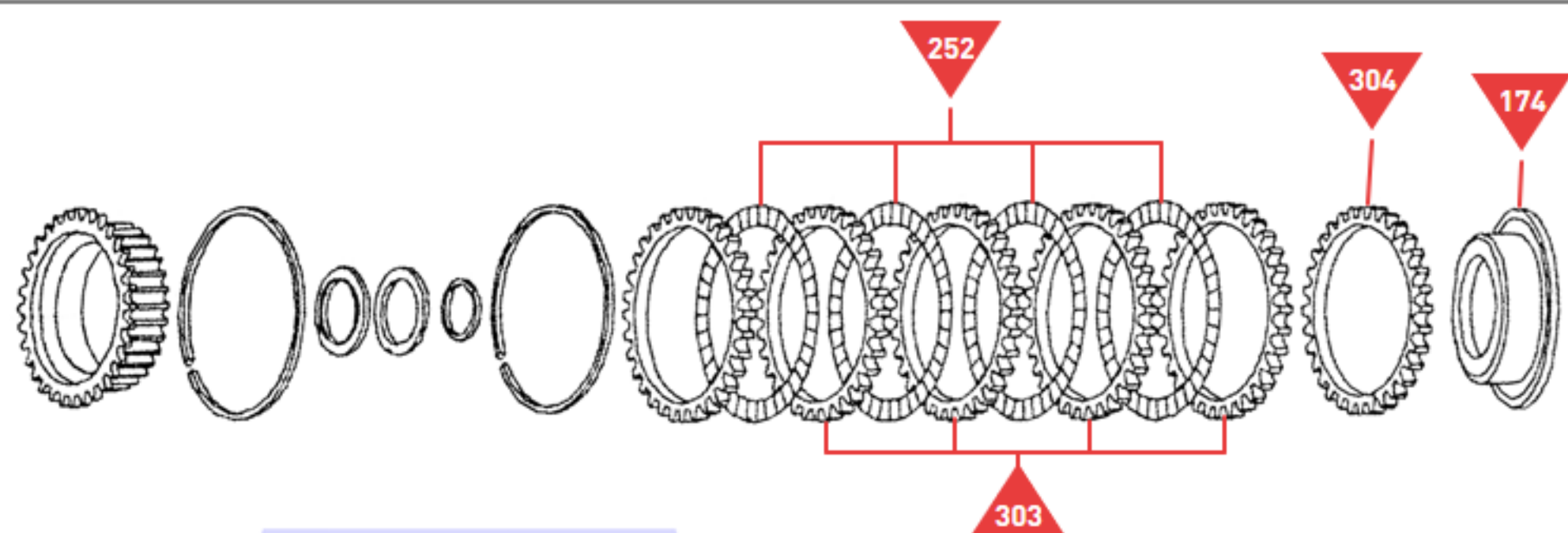
'C3' Clutch
