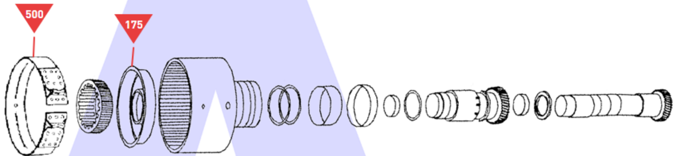
'C3' Clutch
