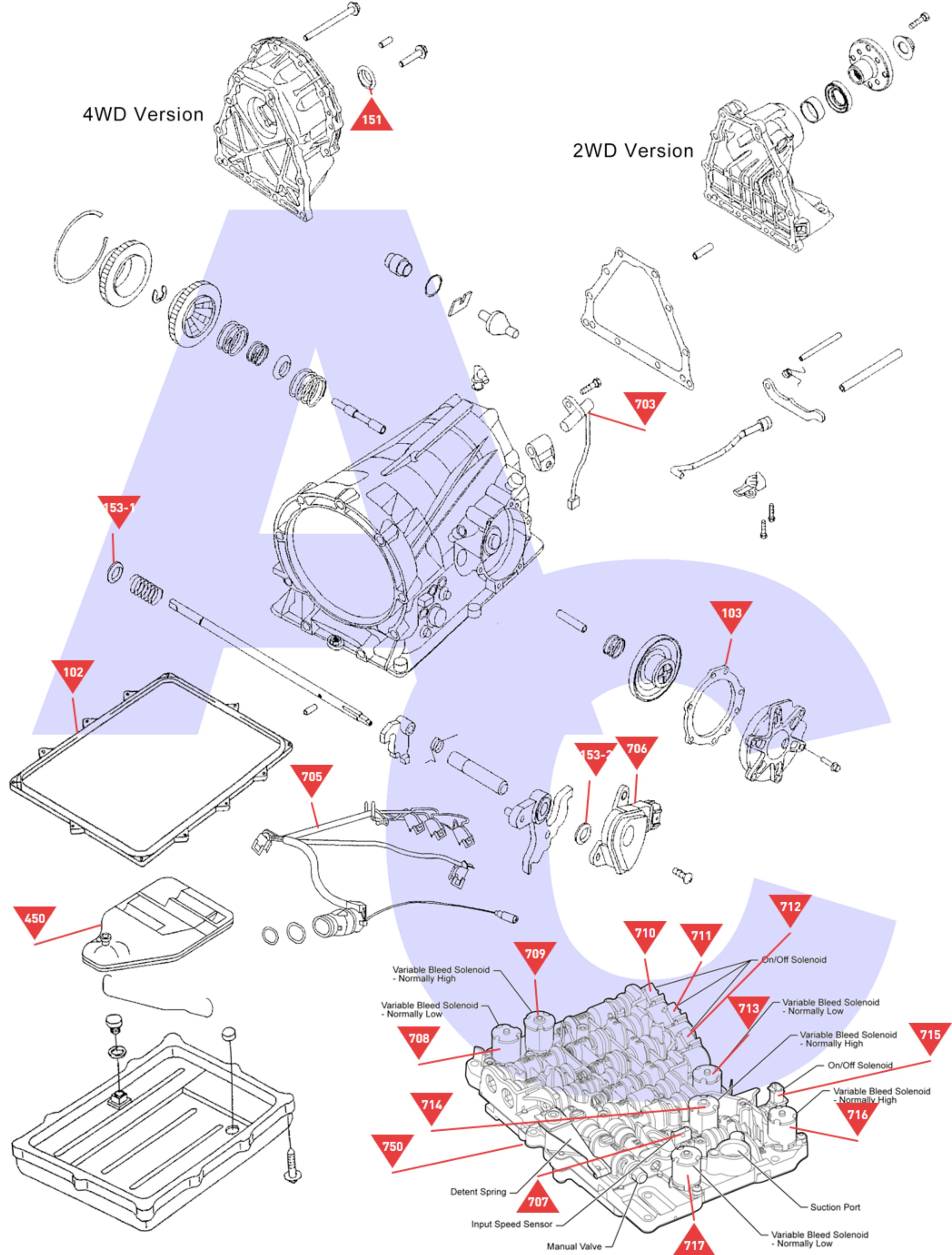
Case, Valve Body, Oil Pan, Filter and Electrical Components
