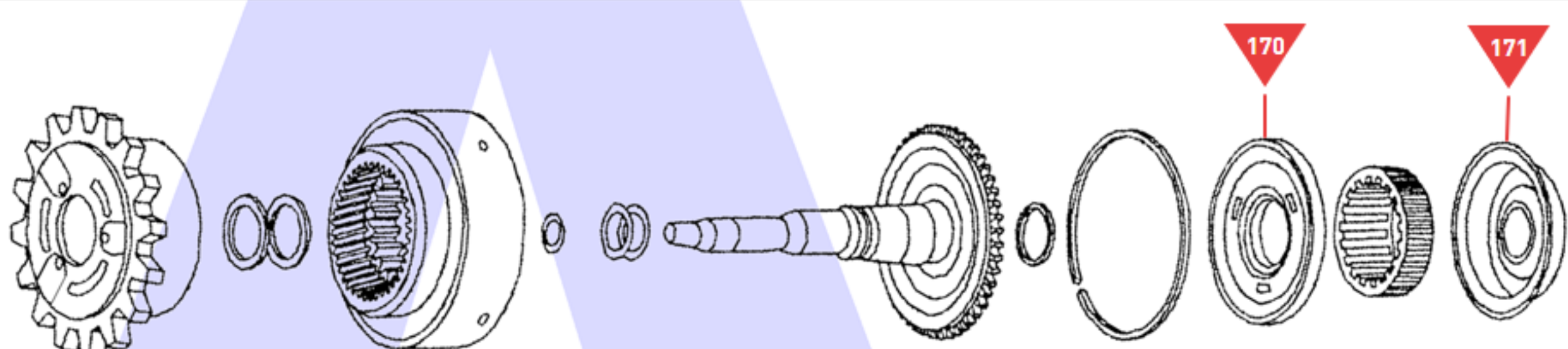
Front Planet, 'C1' Cylinder and Input Shaft
