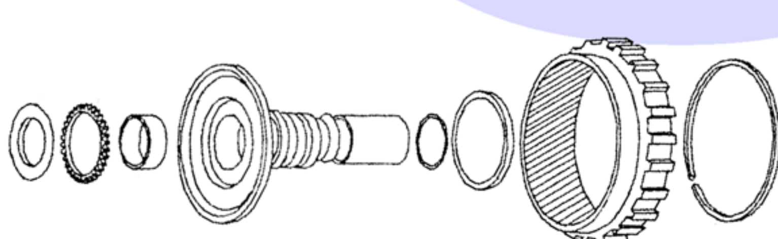
Output Shaft & Rear Anulus
