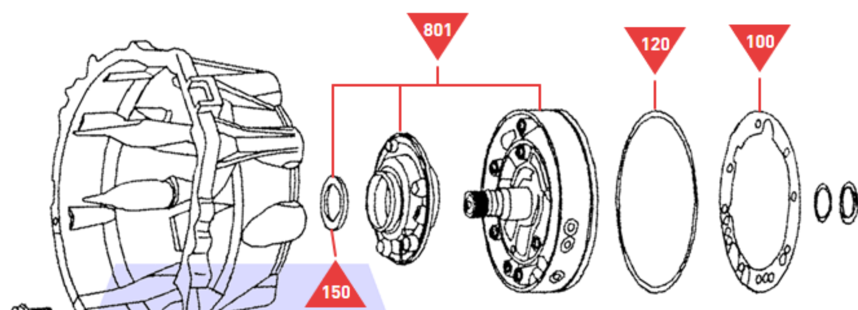
Bell Housing & Oil Pump
