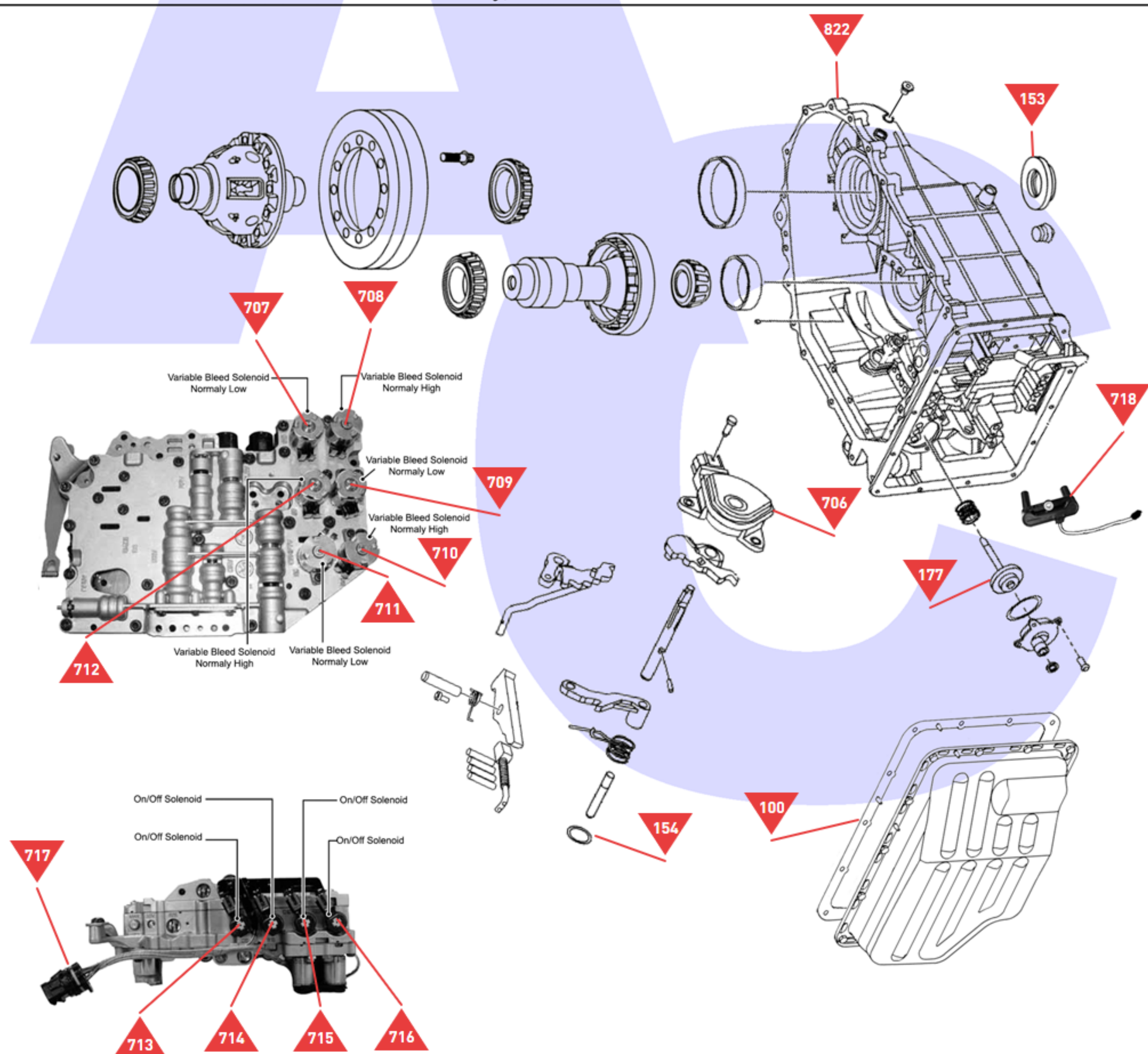
Main Case, Diff, Transfer Gear, Valve Body, Valve Body Cover and Linkages
