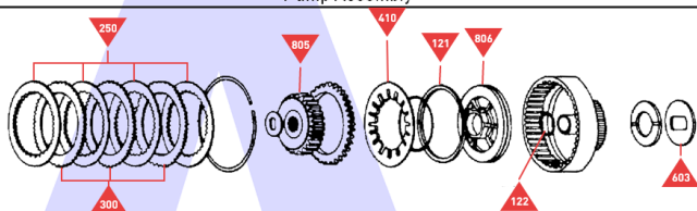
Forward Clutch Assembly
