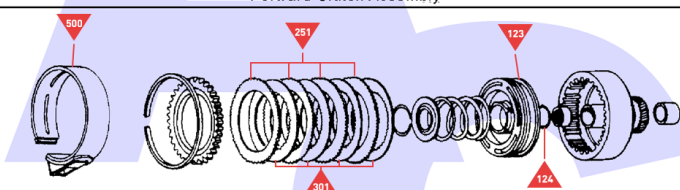
Direct Clutch Assembly
