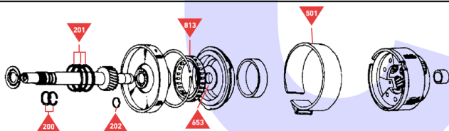
Planetary Assembly
