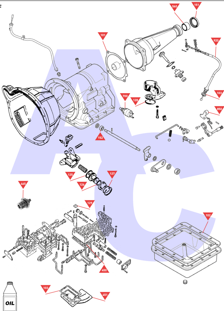
Casing, Servo's, Oil Pan Etc
