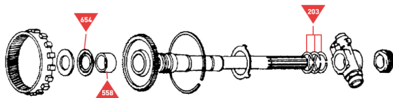
Output Shaft Assembly
