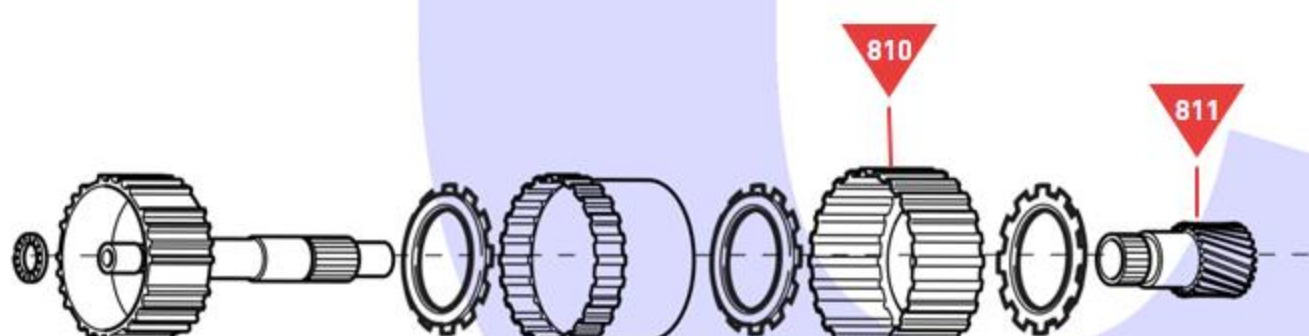
Rear Clutch Drum Assembly
