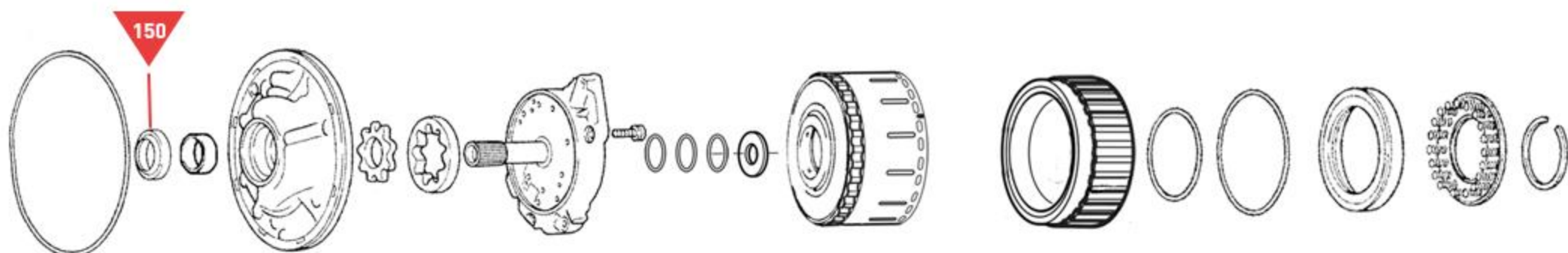
Oil Pump and Front Multi Clutch Drum
