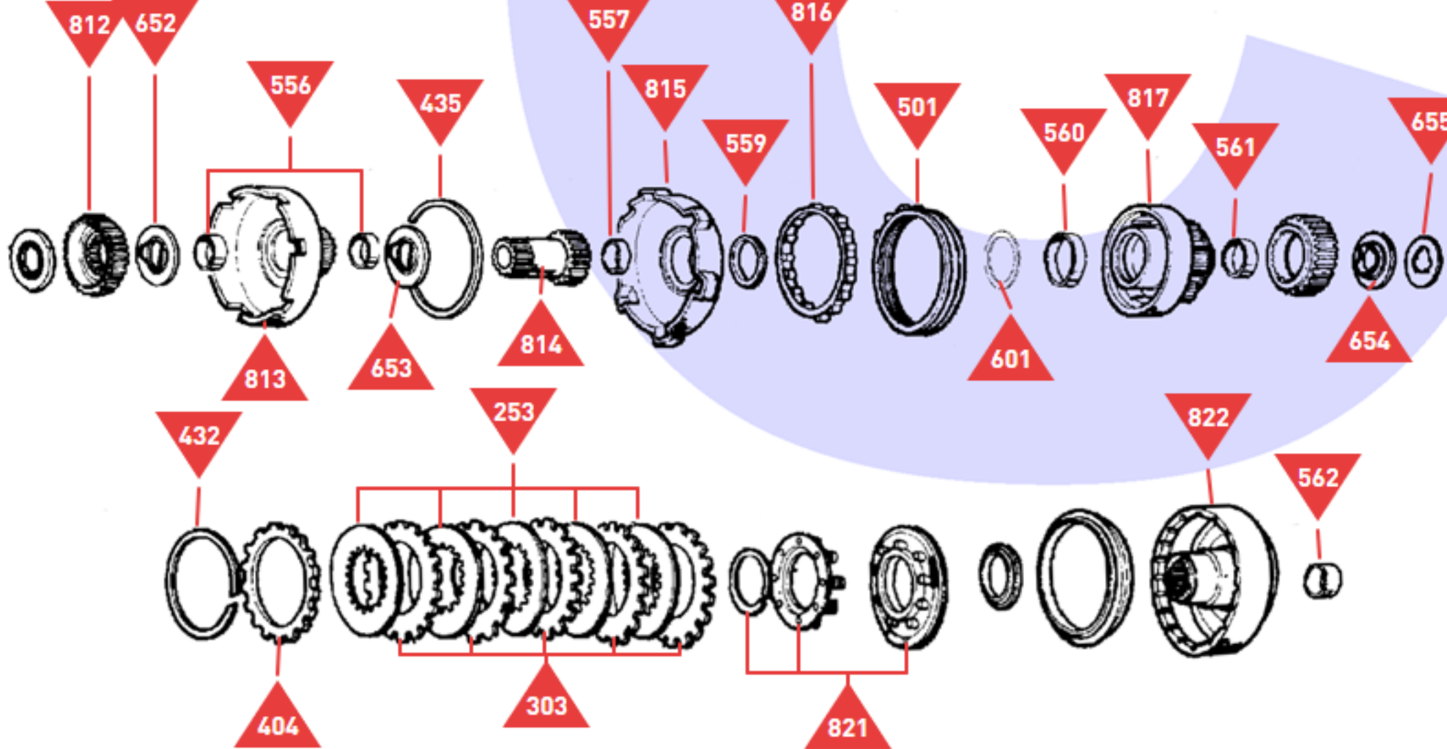
Reverse and Forward Clutches
