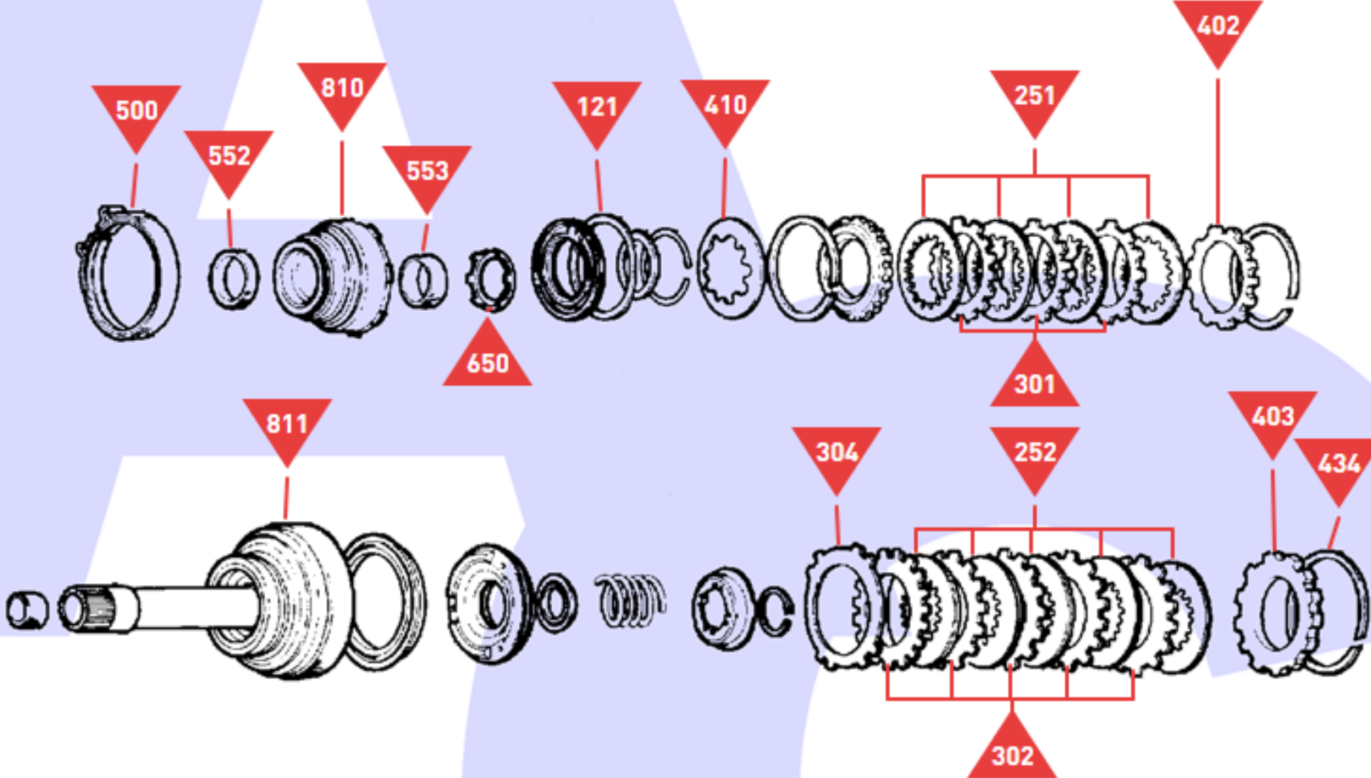
Pump and Intermediate Clutch
