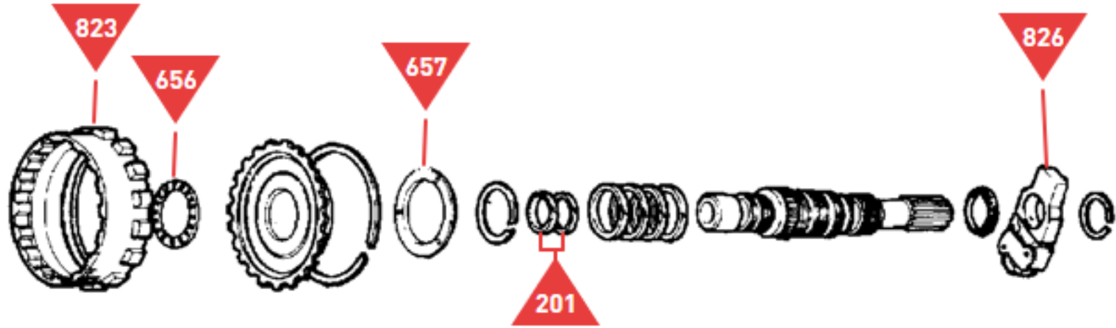
Planetary Set and Direct Clutch
