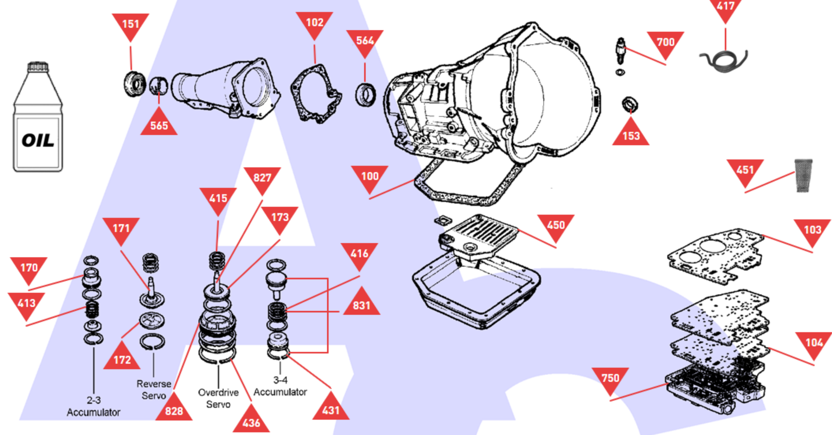
Case, Valve Body, Servo's and Accumulators
