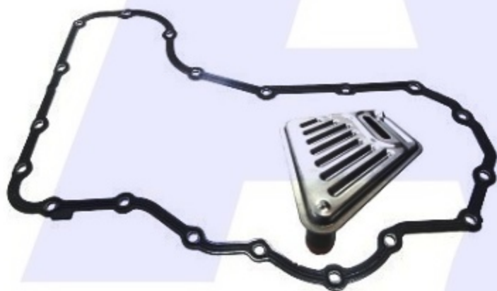
FORD AX4N Pan Gasket AX4N.GAS11 Filter AXODE.FIL02 Filter has Orange Seal
