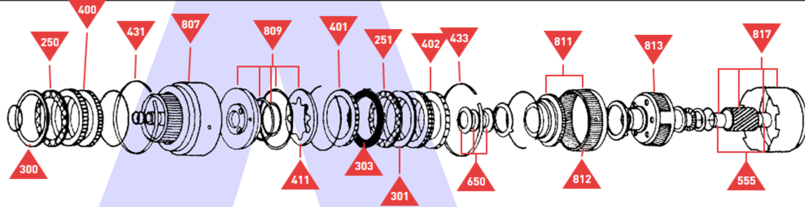
Forward Clutch and Front Planetary
