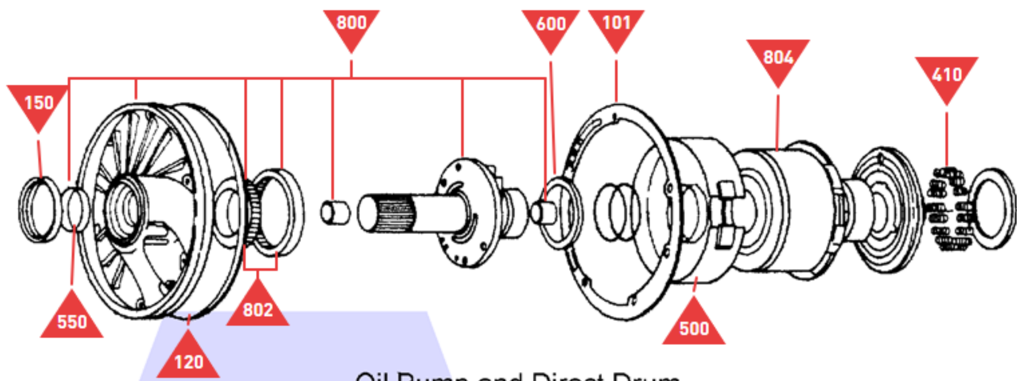
Oil Pump and Direct Drum
