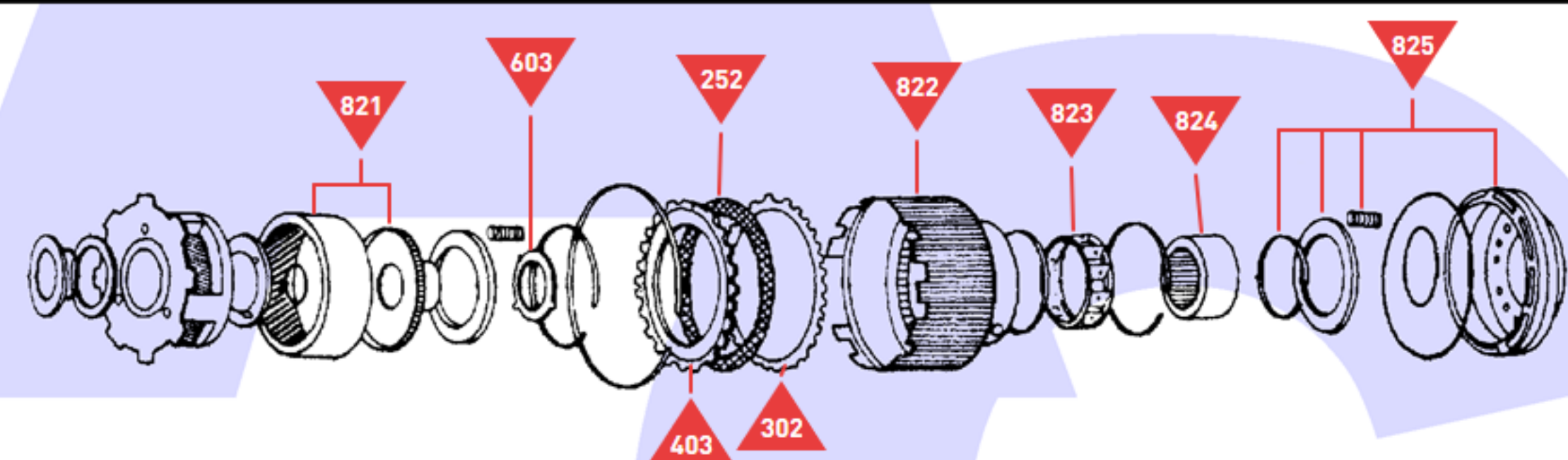
Forward Clutch and Front Planetary
