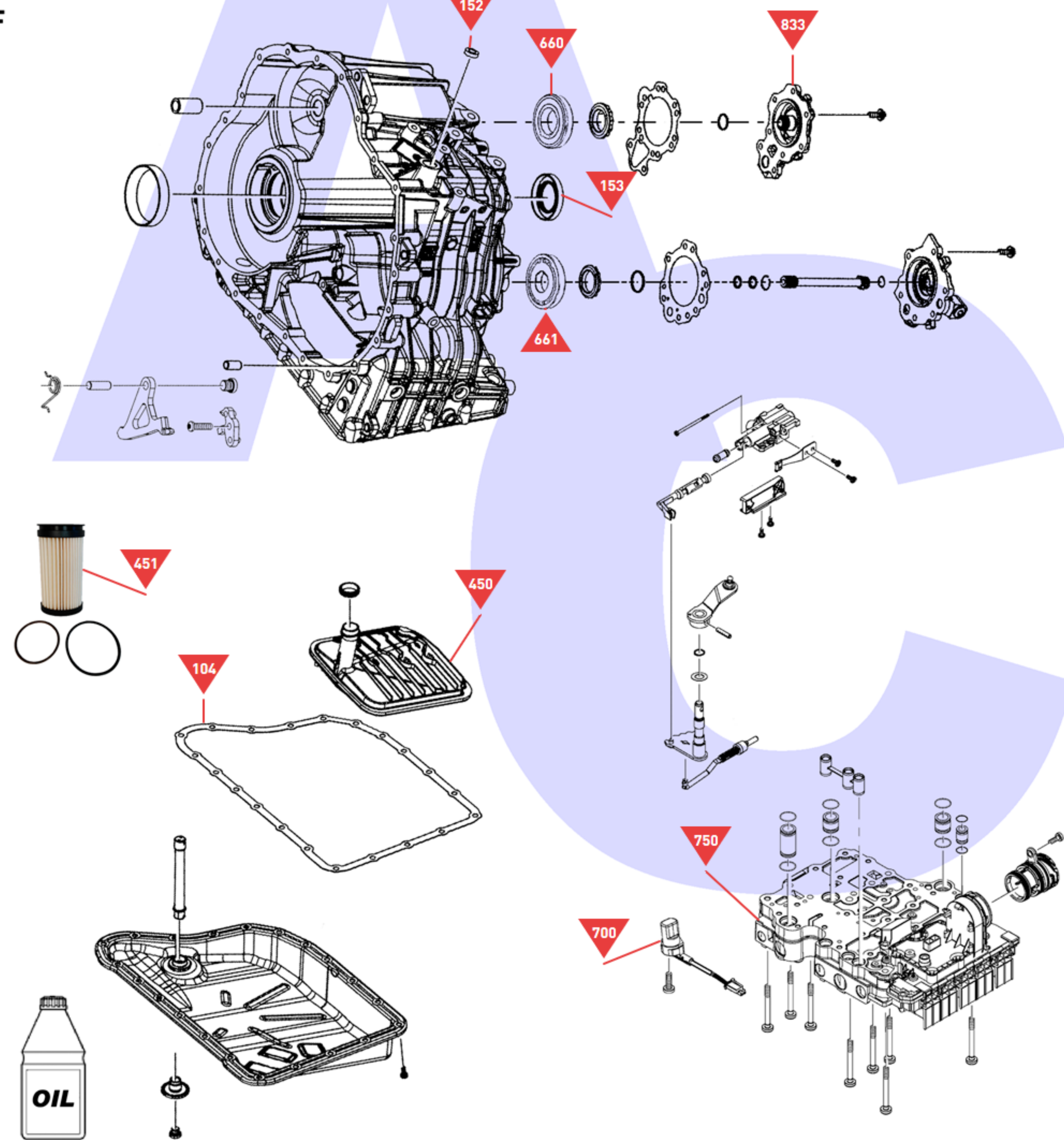
Main Case, Oil Pan, Filter, Mechatronic Etc
