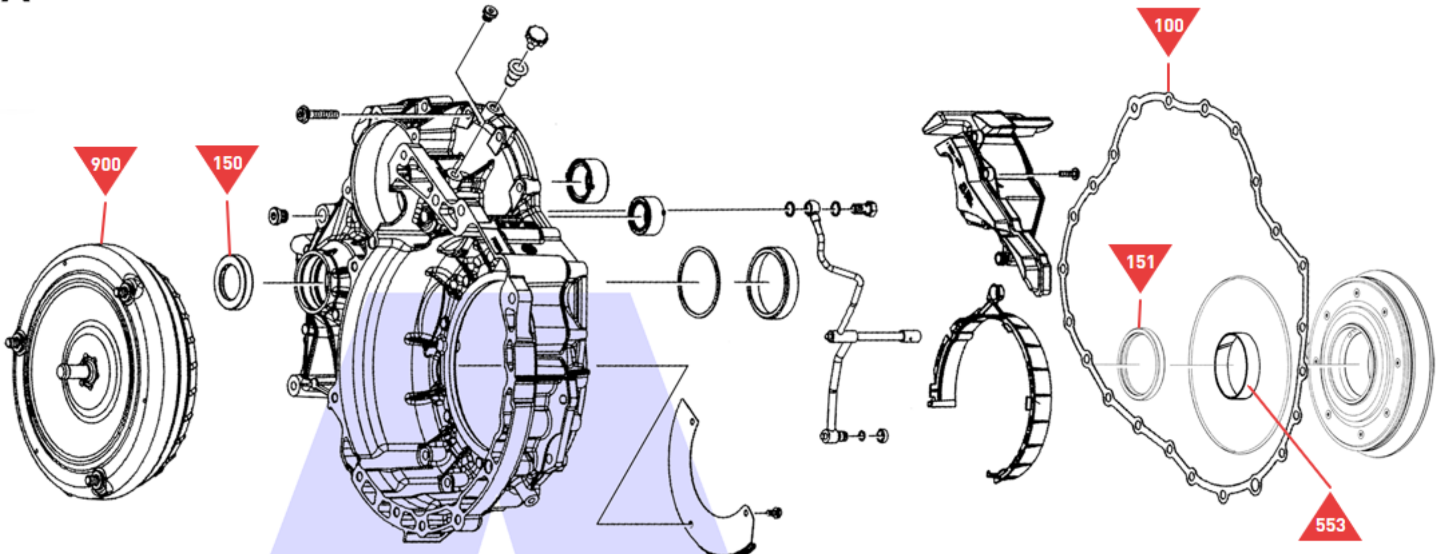
Torque Converter, Bell Housing & Pump
