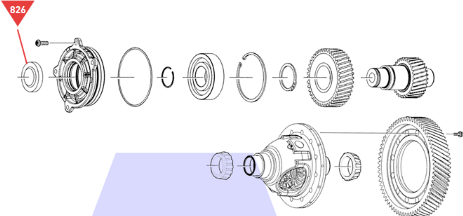
Output Gears & Differential Assembly
