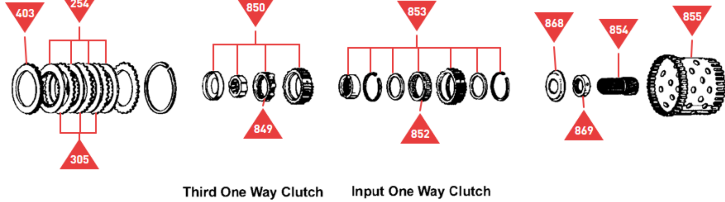
Input and Third Drum
