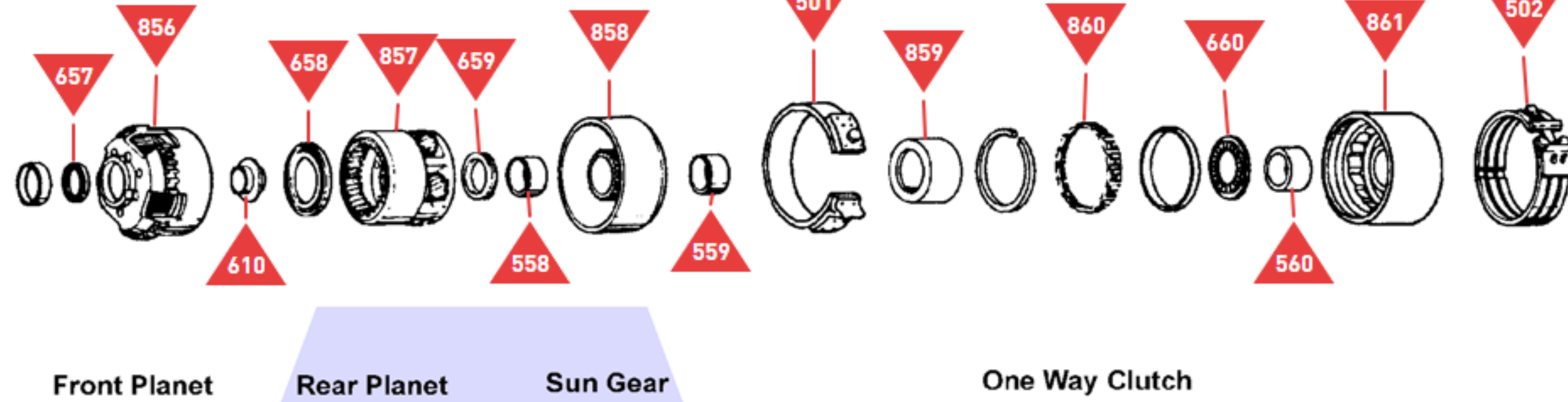
Third One Way Clutch
