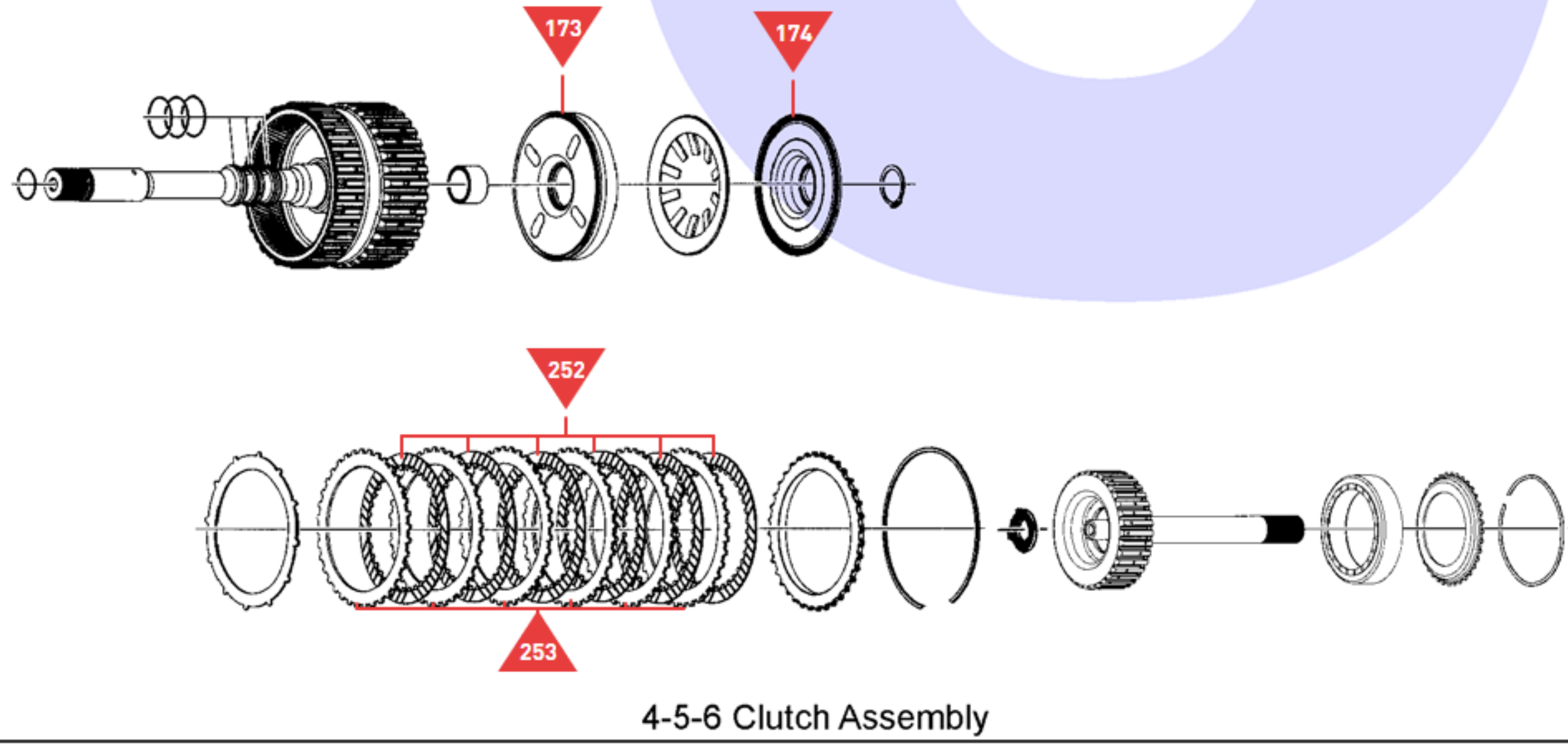
4-5-6 Clutch Assembly
