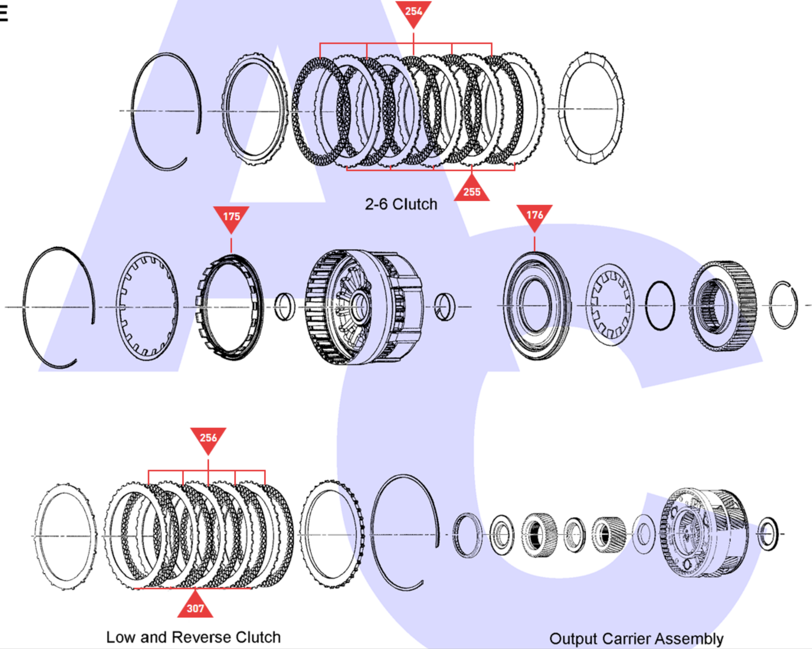
Low and Reverse Clutch
