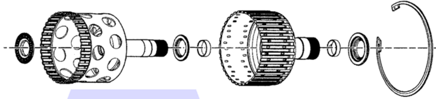
1-2-3-4 Clutch Hub, 2-6 & 3-5-Reverse Clutch Hub
