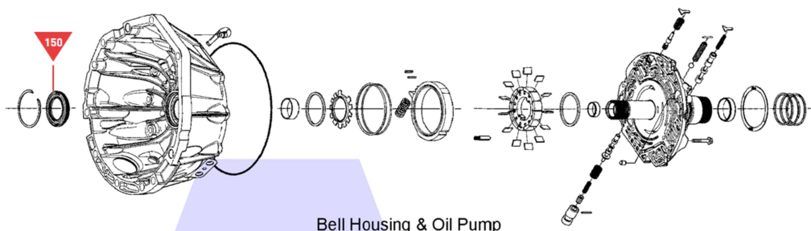
Bell Housing & Oil Pump
