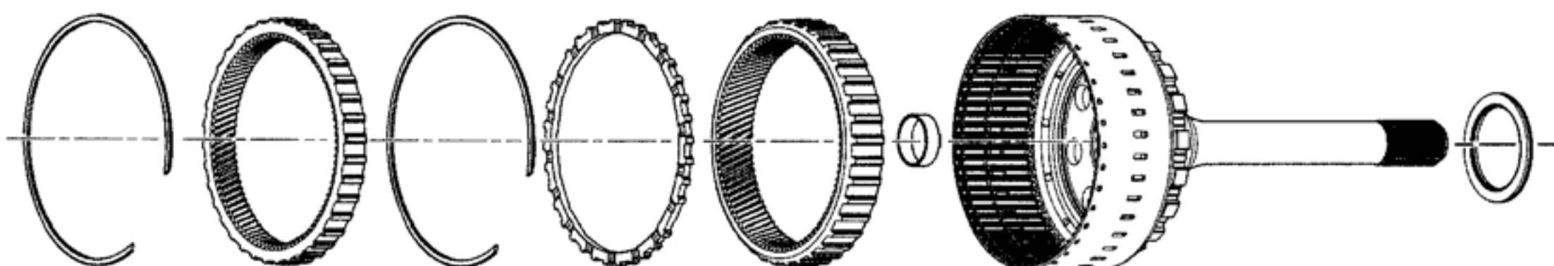
Output Shaft Assembly
