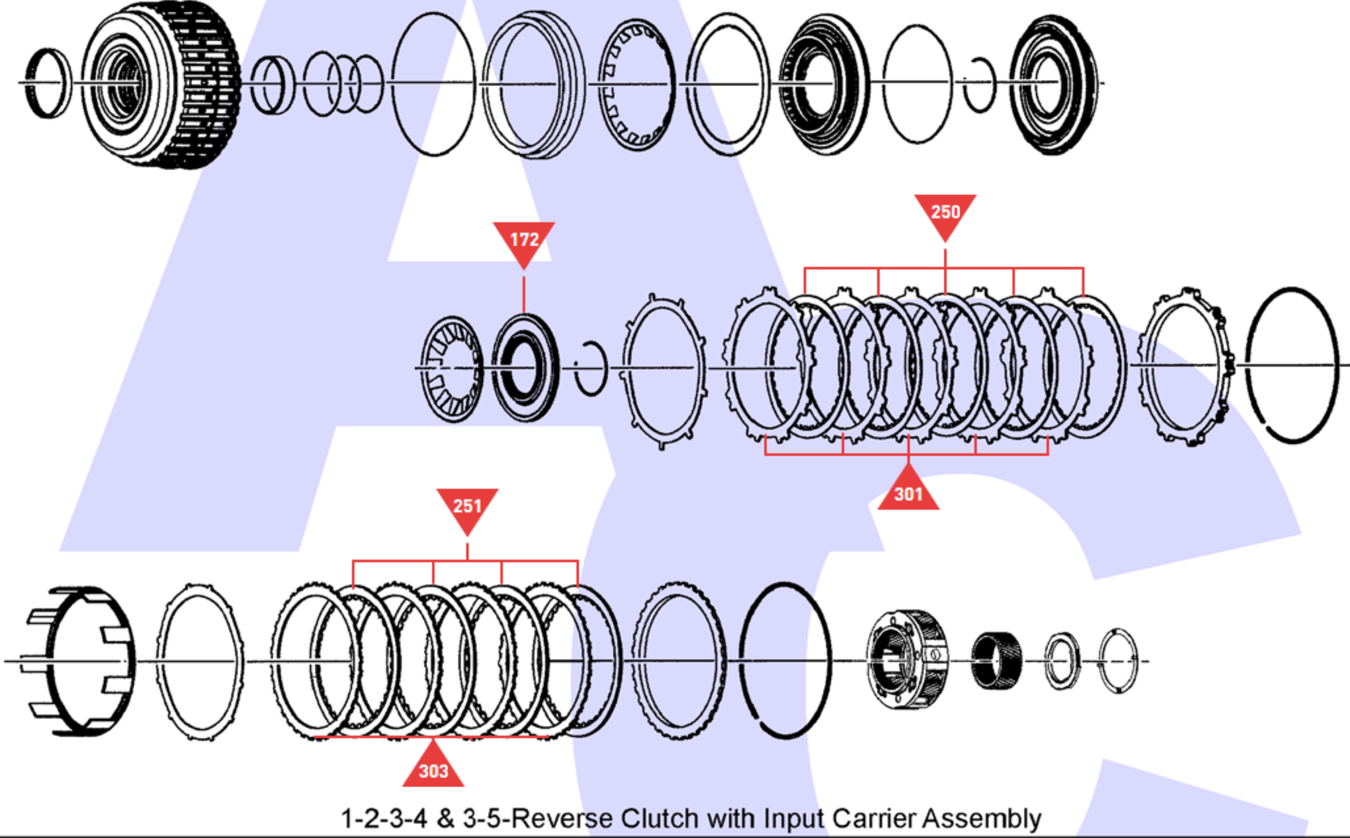
1-2-3-4 & 3-5-Reverse Clutch with Input Carrier Assembly
