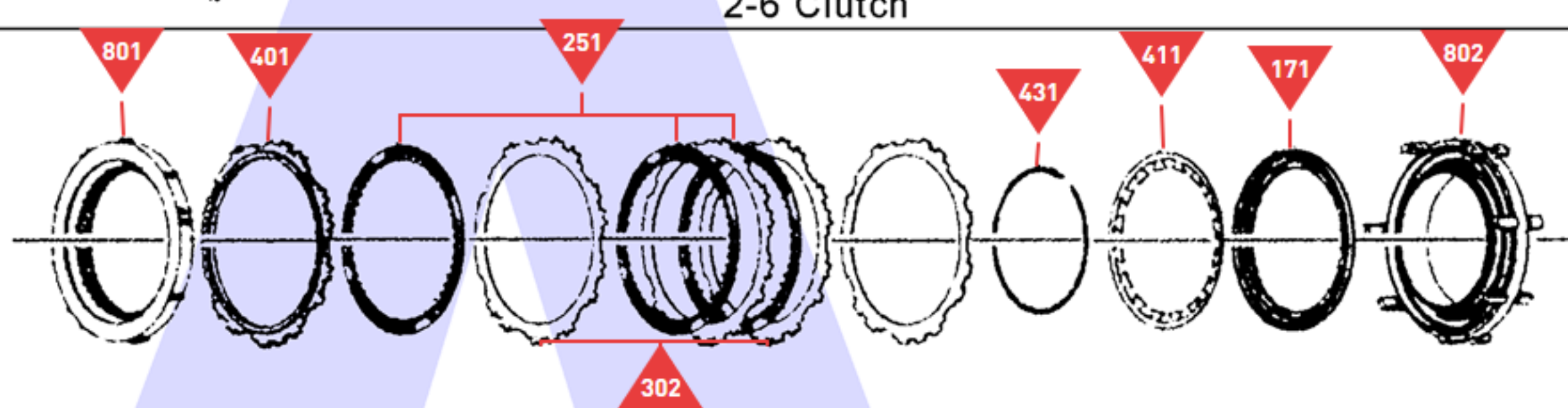
Low & Reverse Clutch
