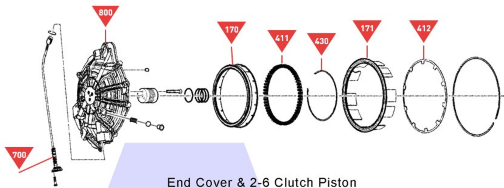
End Cover & 2-6 Clutch Piston
