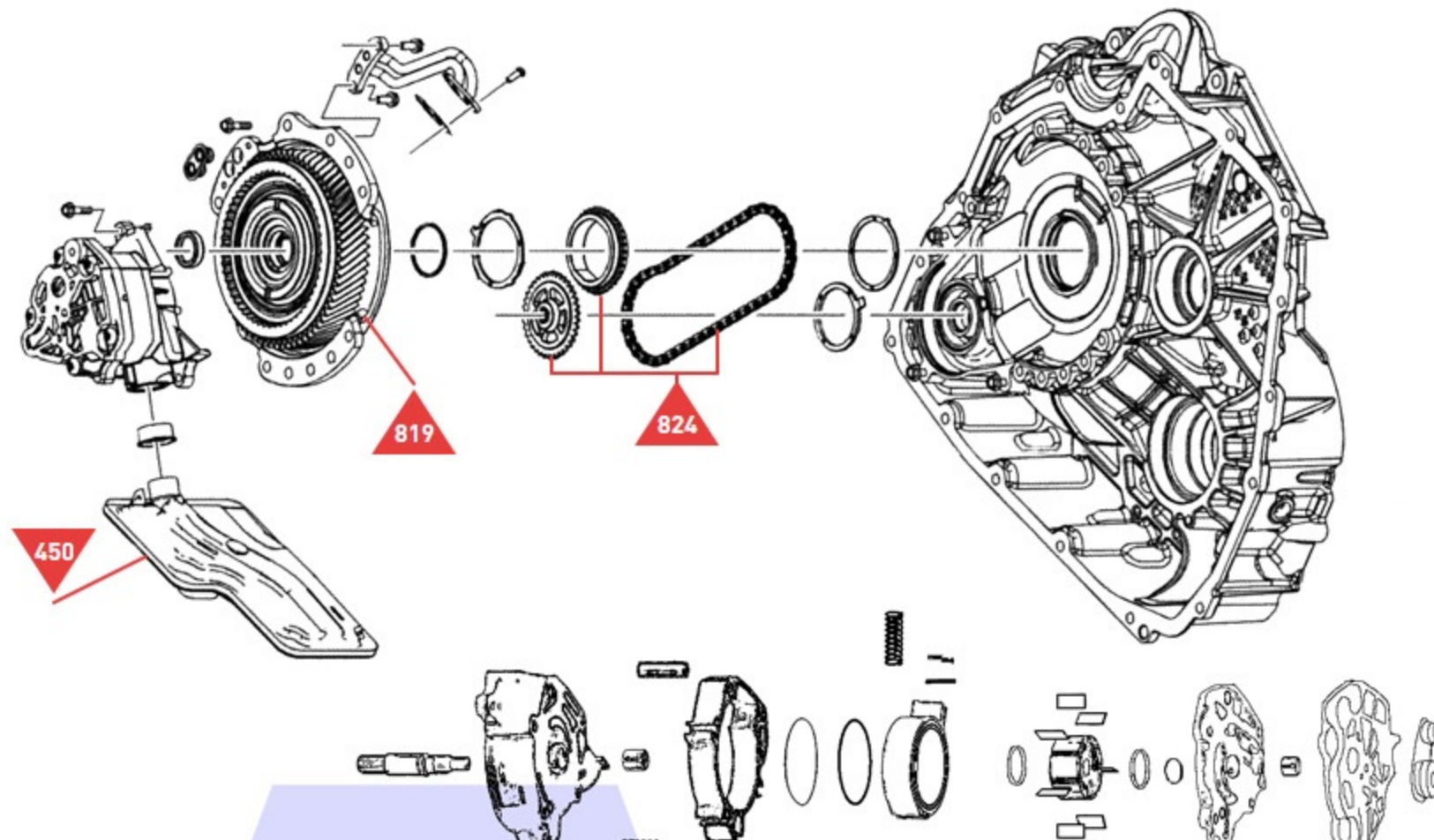
Filter, Oil Pump & Ancillary Items
