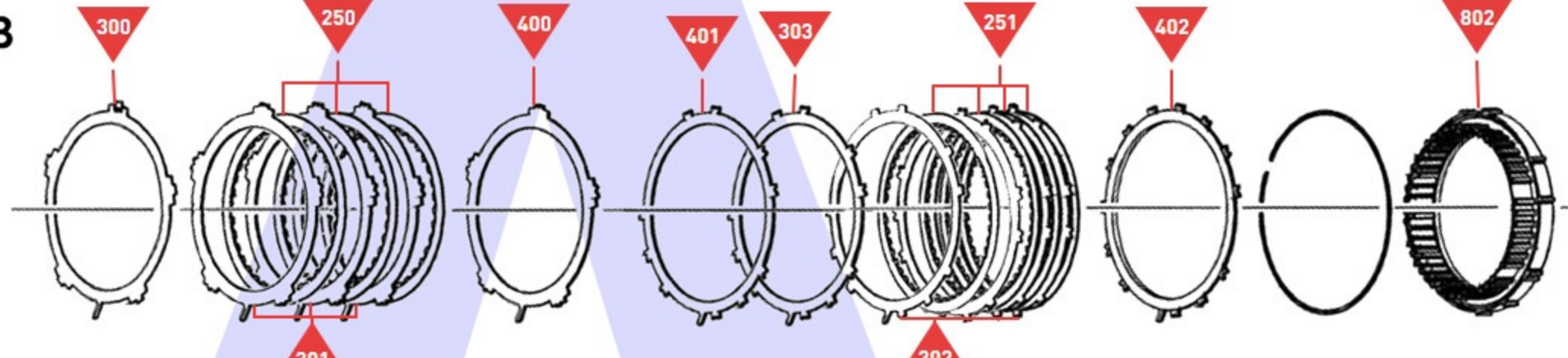
2-6 Clutch Assembly
