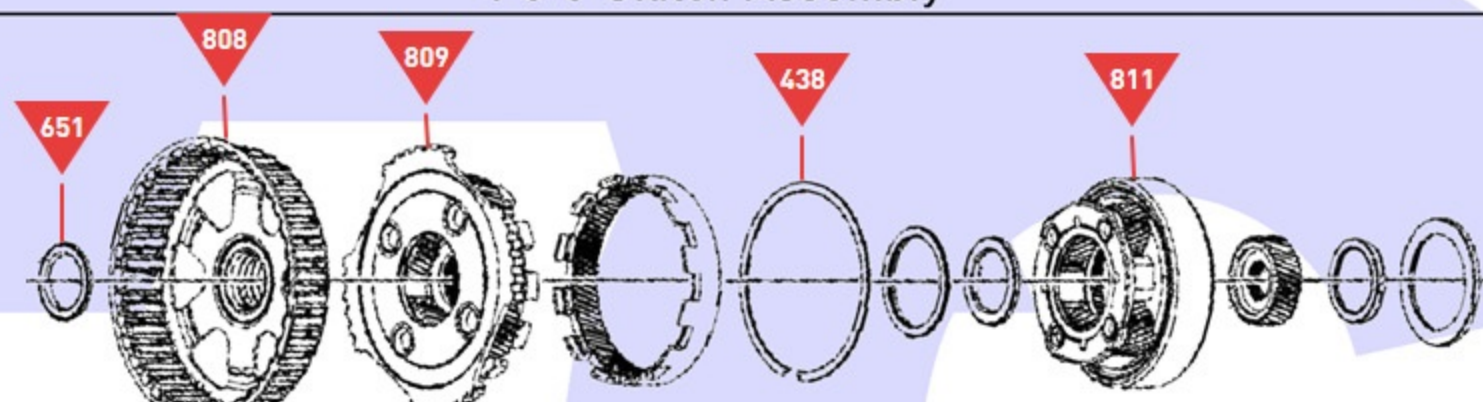
4-5-6 Clutch Assembly
