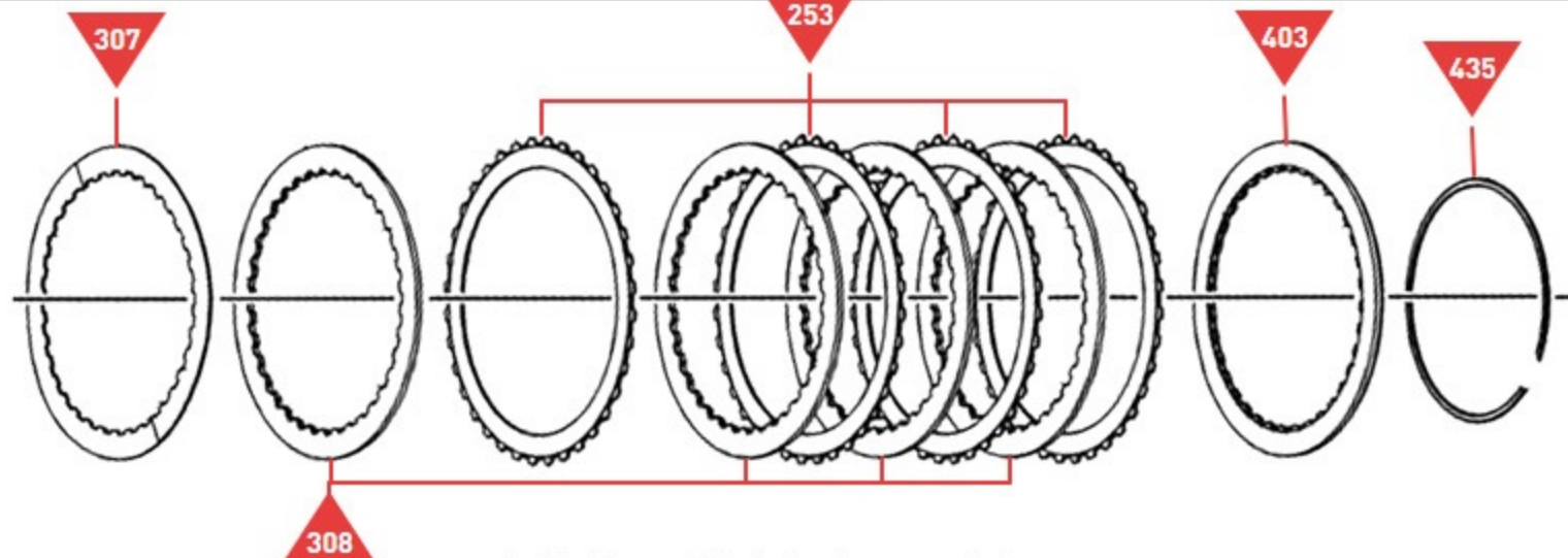
3-5-Rev Clutch Assembly
