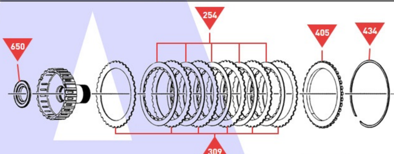
4-5-6 Clutch Assembly
