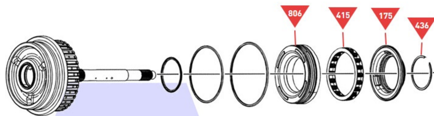
4-5-6 Clutch Piston Etc.
