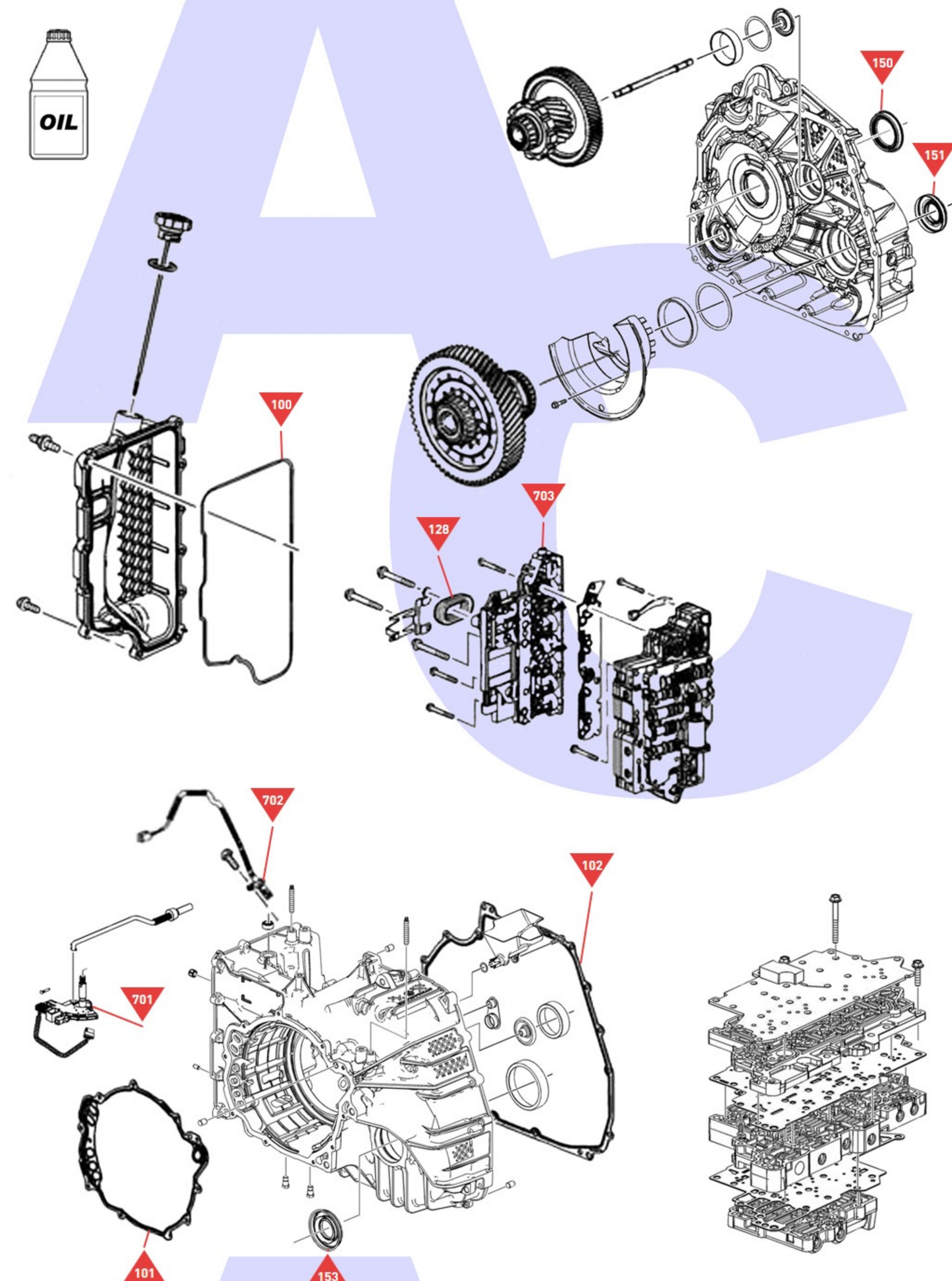
Case Components, Valve Body, Differential Etc.
