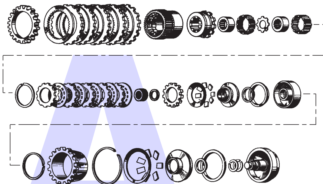
Forward and Coast Clutch Assemblies
