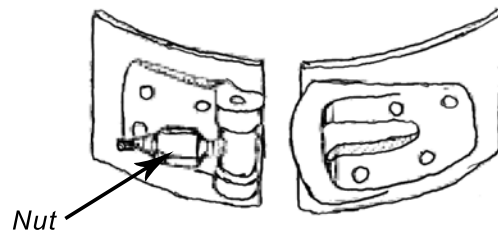
Rear Band 1954-1957 GMC 350 & 650 truck Rigid 55.80mm wide With adjusting nut
