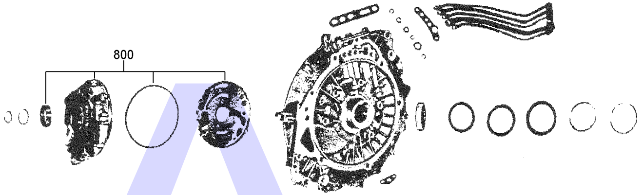
Pump Assembly & Case Cover
