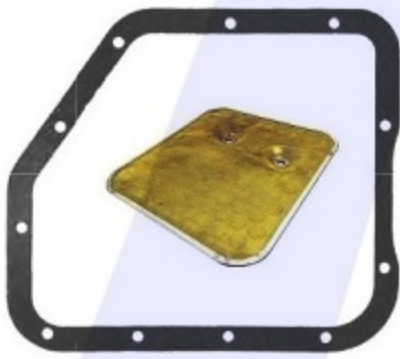
TH200 1976-1978 Pan Gasket in Kit Only Filter TH200.FIL01 Brass
