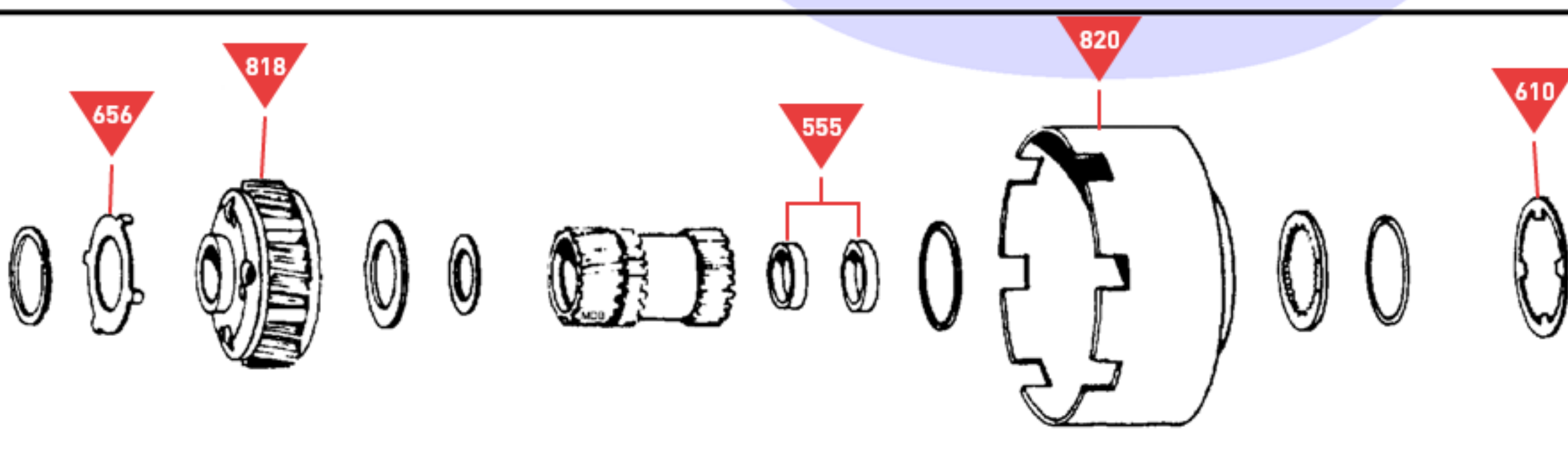
Front Planetary and Sun Gear
