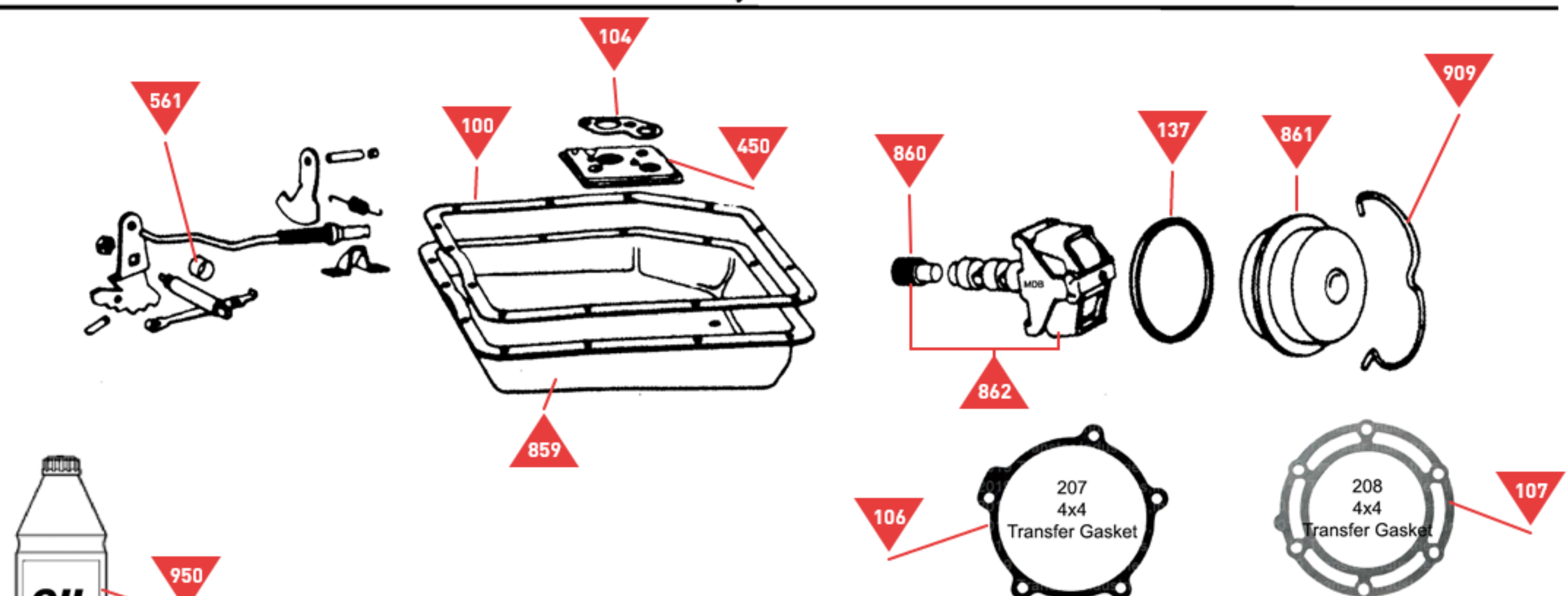
Valve Body and Servo
