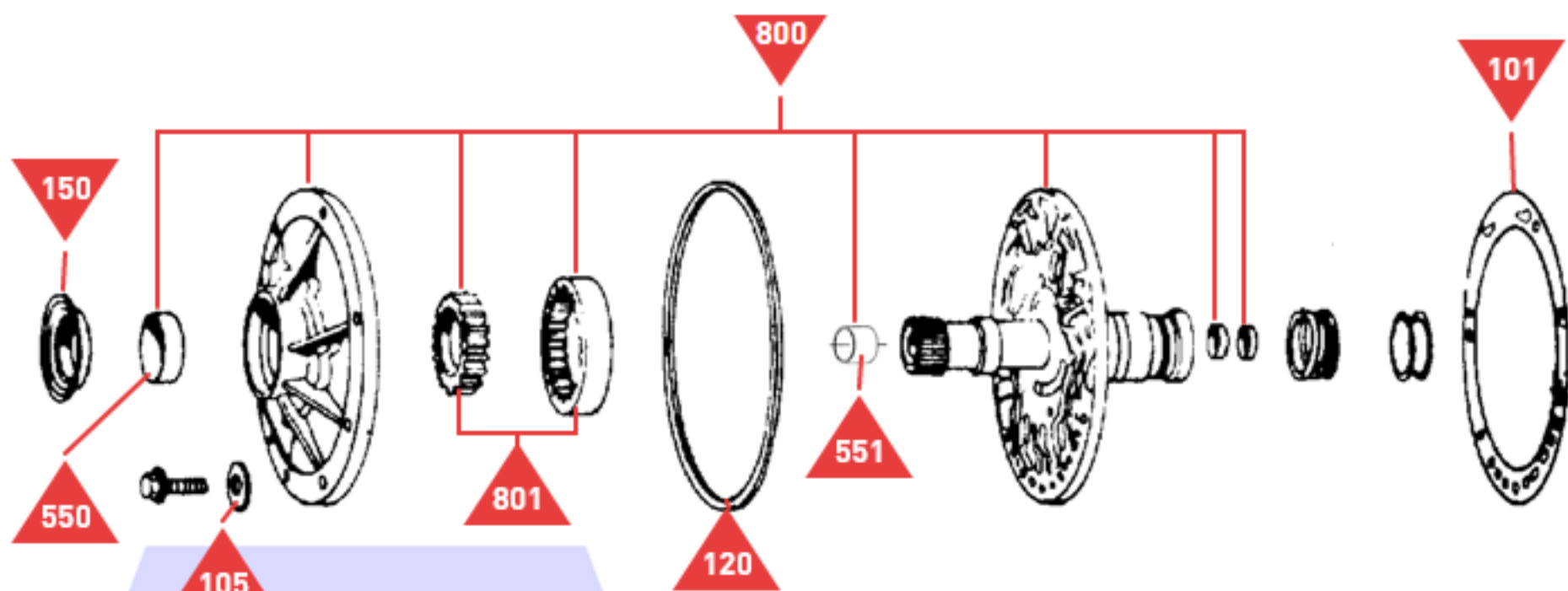
Pump Assembly
