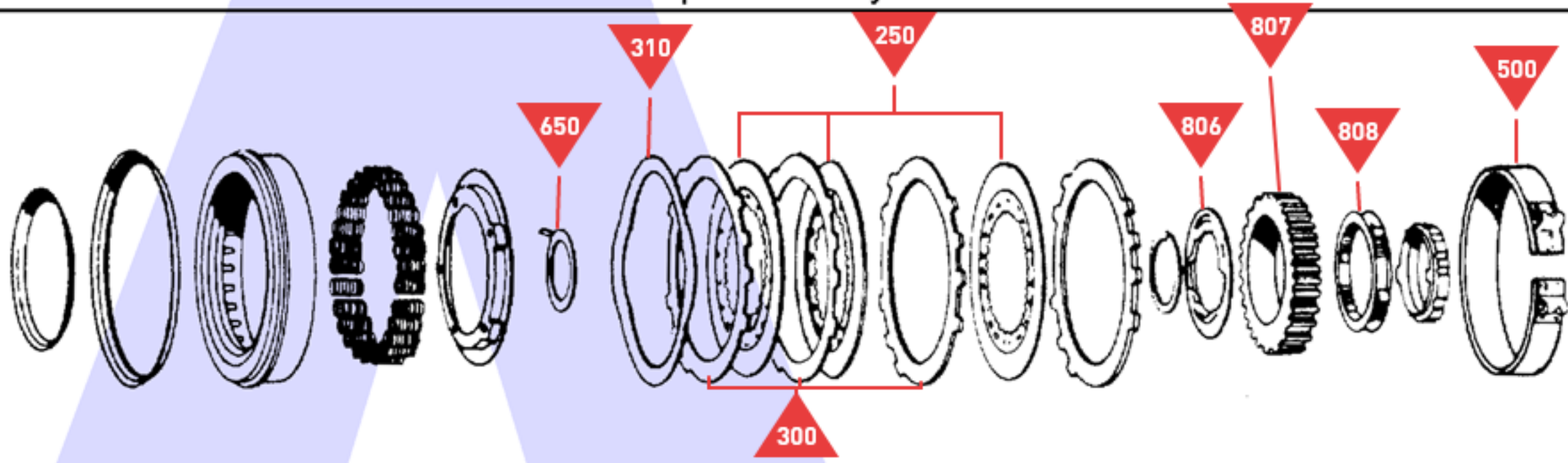
Intermediate Clutch
