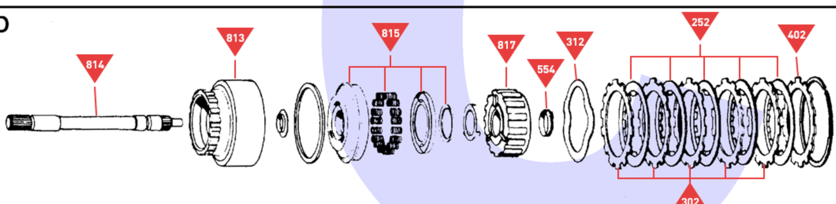
Forward Clutch
