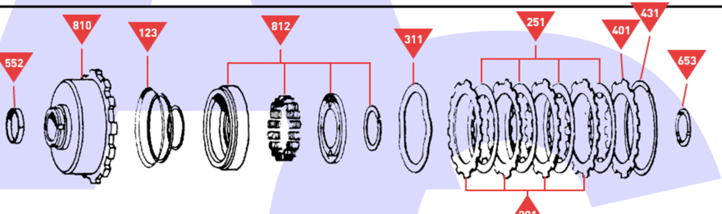
Direct Clutch
