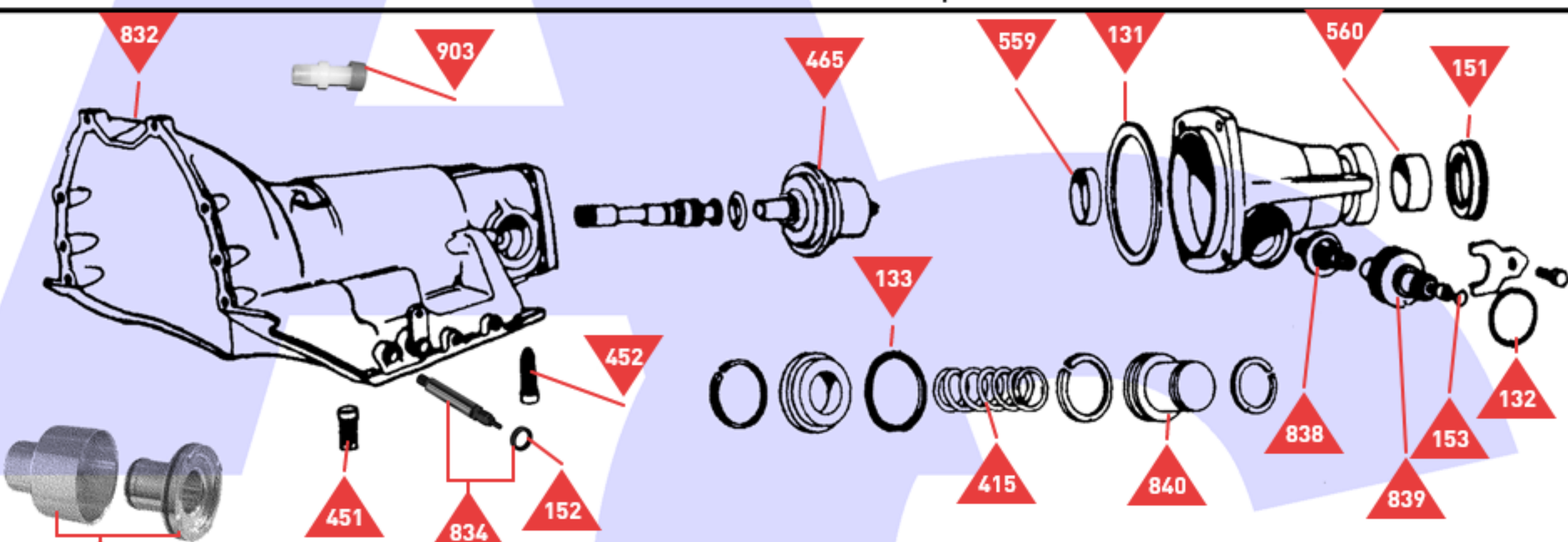
Case and Accumulator
