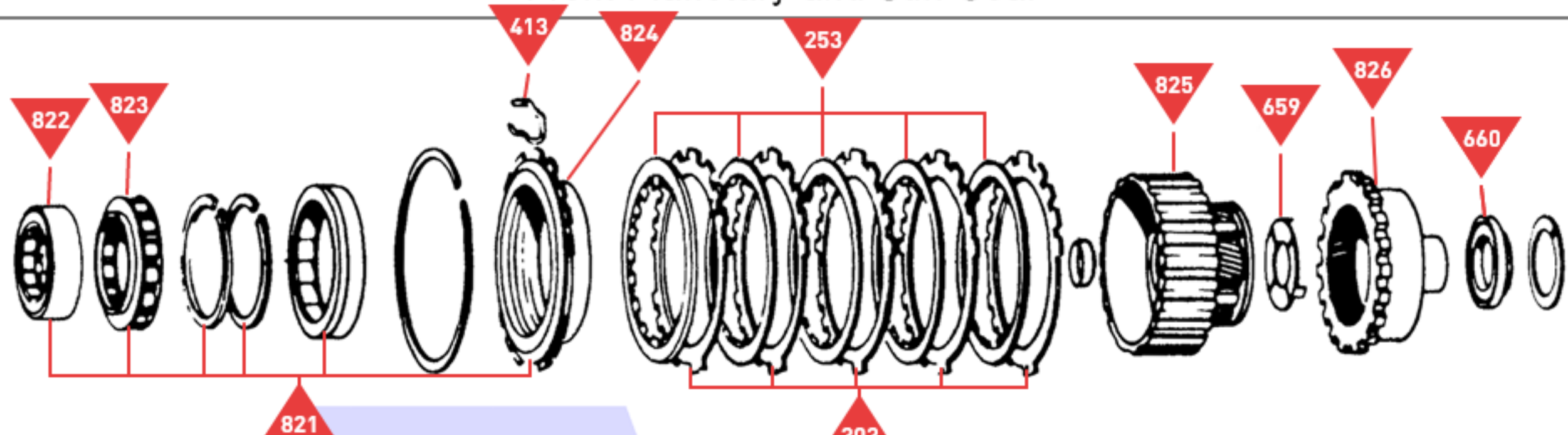
Front Planetary and Sun Gear
