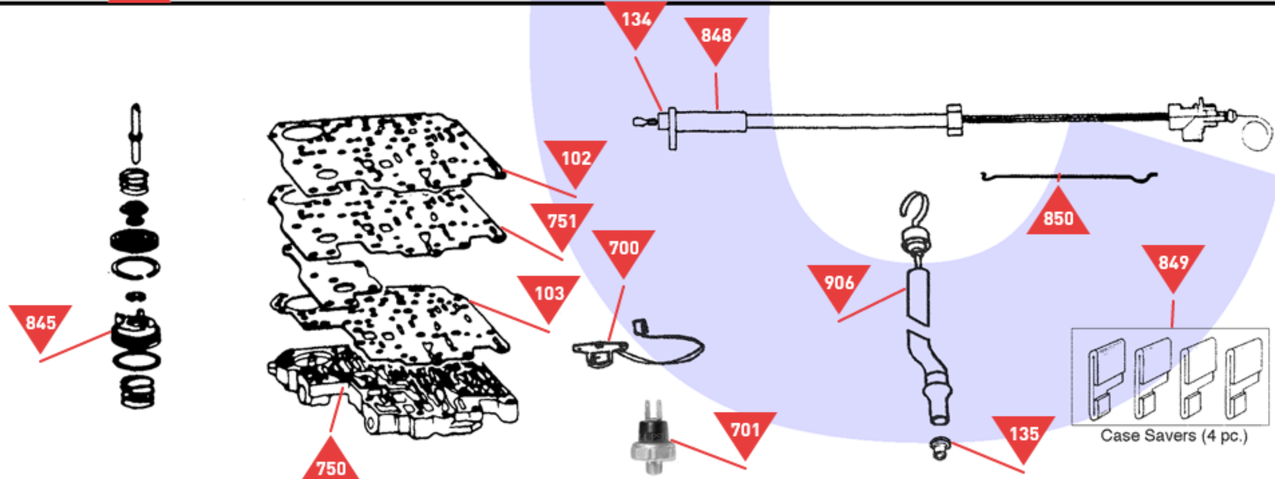
Case and Accumulator
