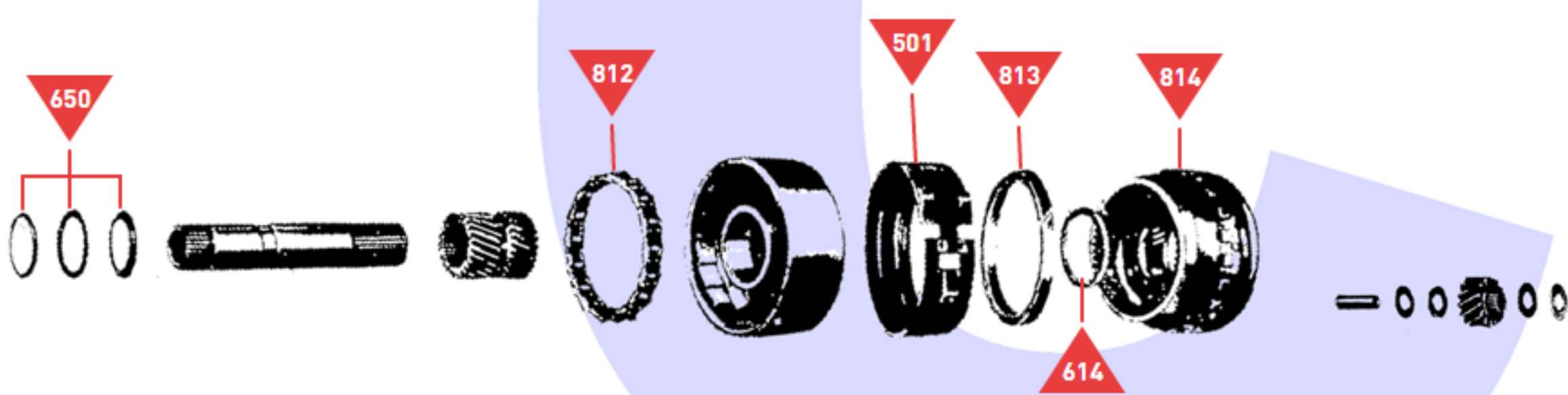
Sun Gear, Low/Reverse Band & Planetary
