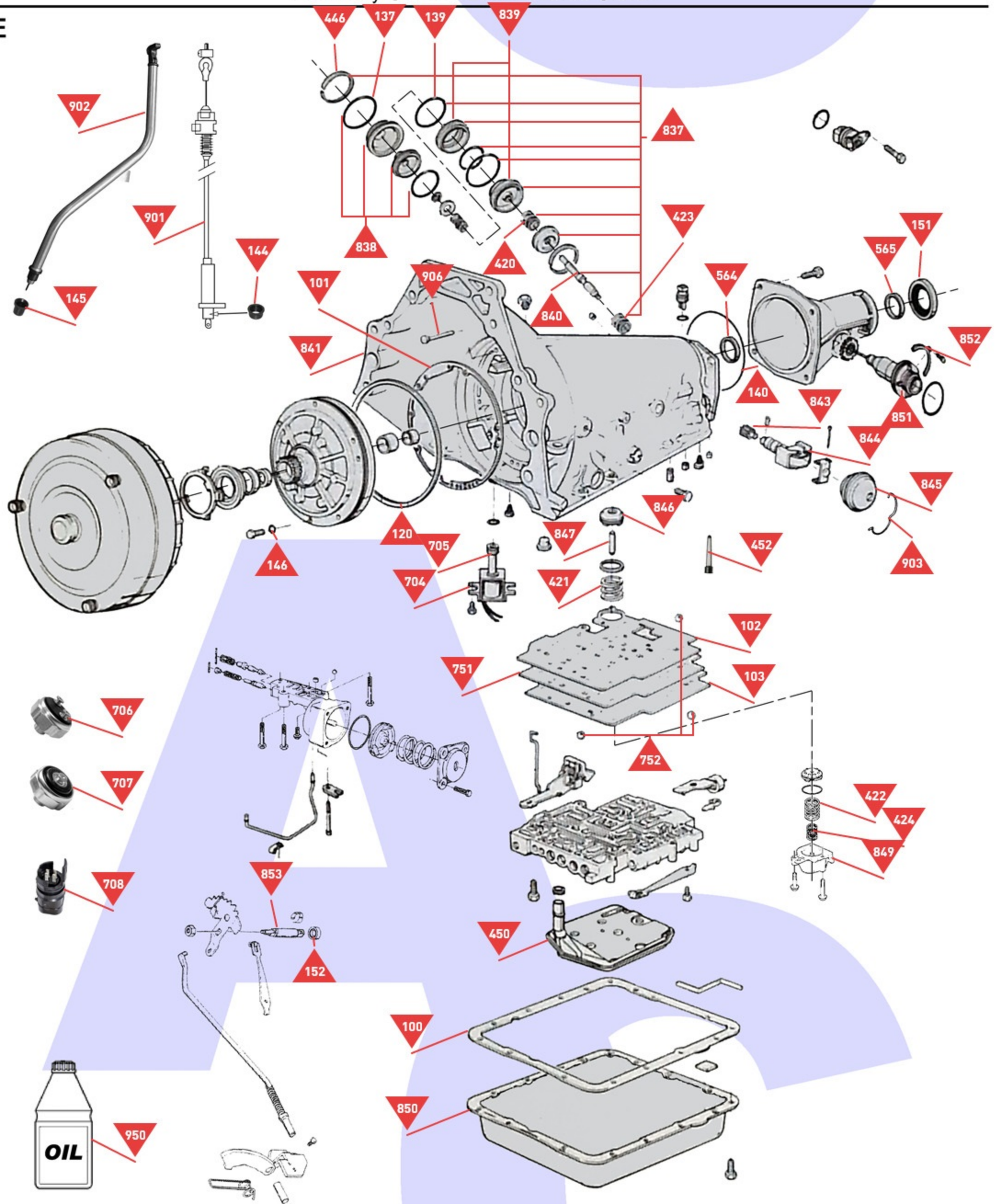
Casings, Valve Body & External Components
