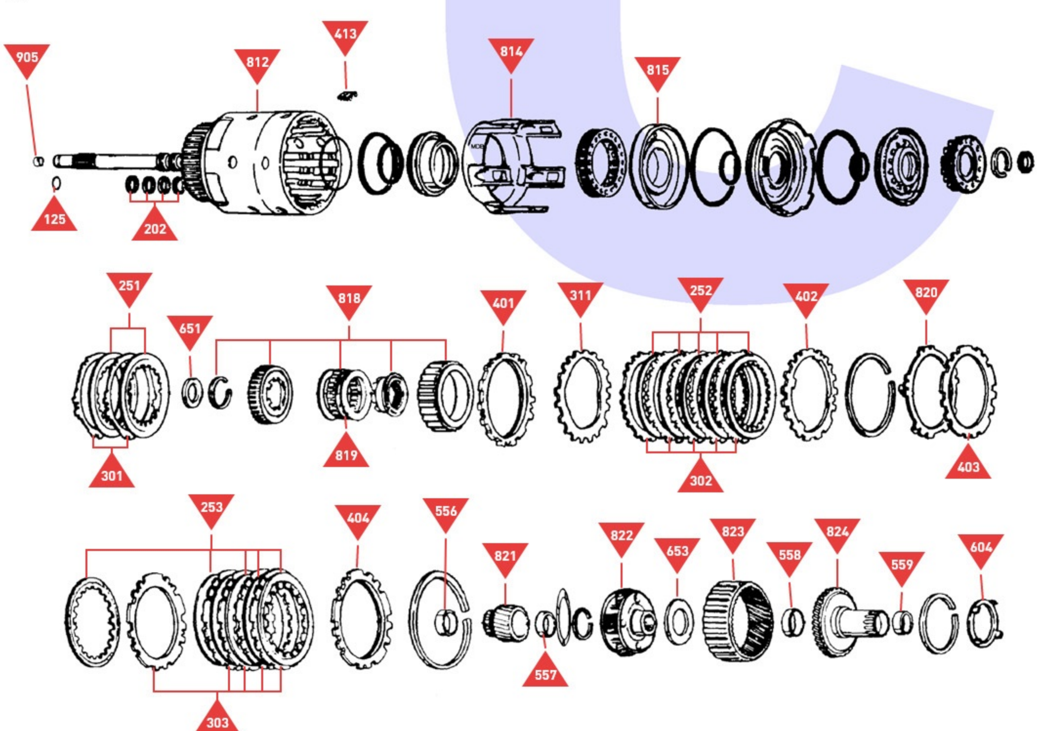
Coast, Forward and 3-4 Clutch
