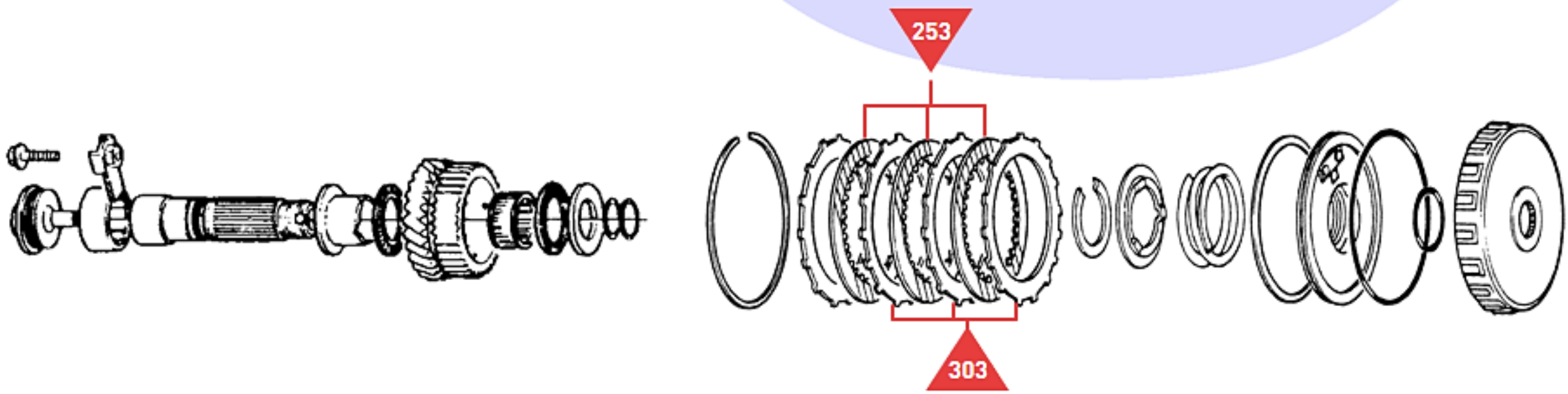
Sub Shaft & First Hold Clutch
