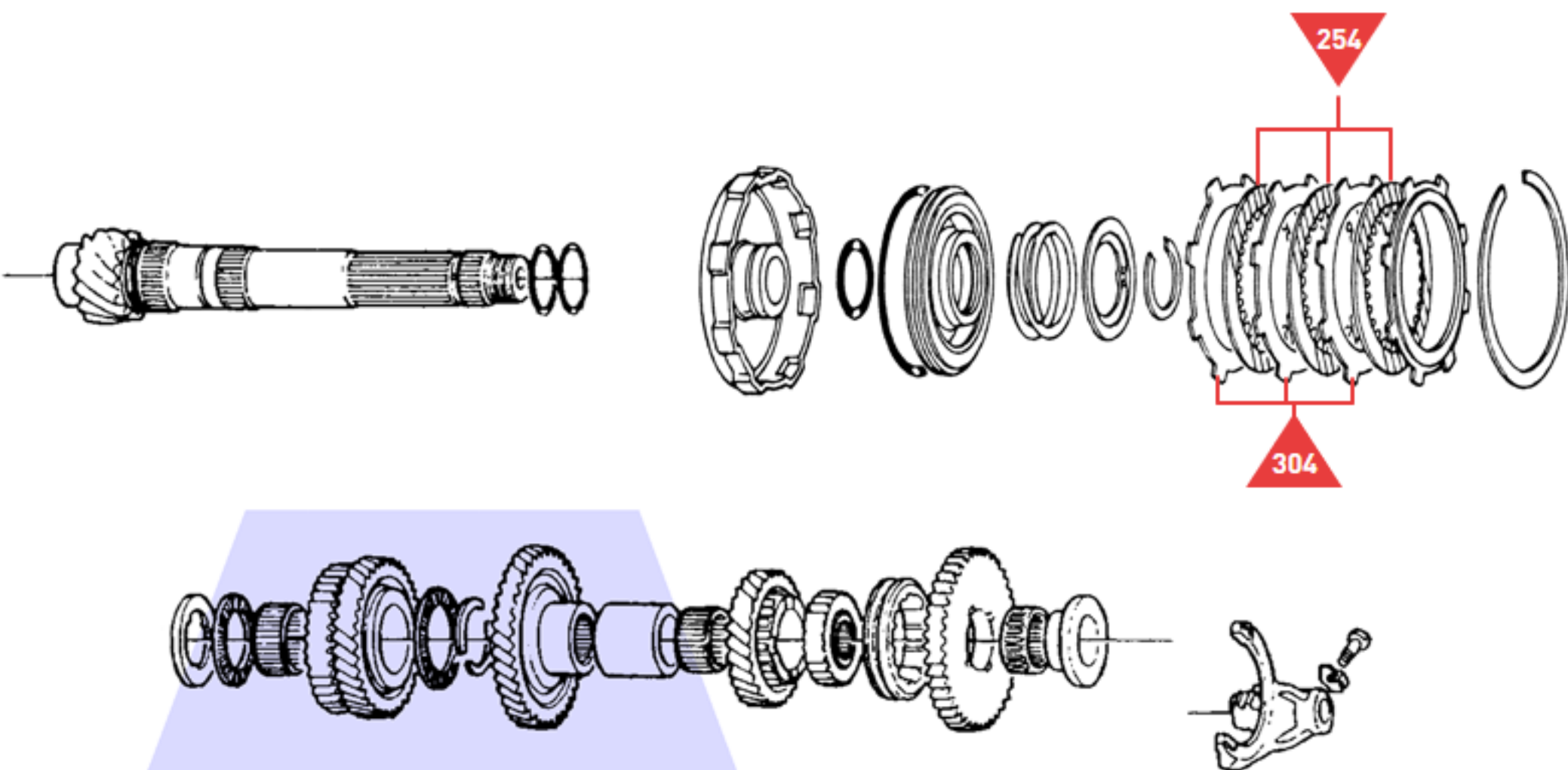
Sub Shaft & First Hold Clutch
