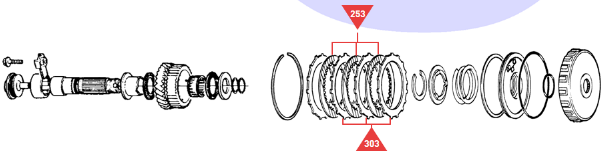
Sub Shaft & First Hold Clutch
