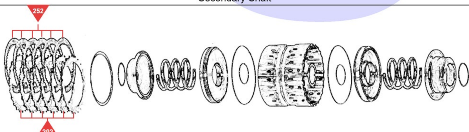
1st & 2nd Clutch
