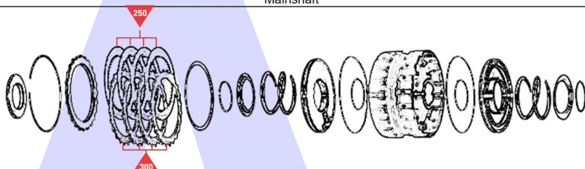
3rd & 4th Clutch
