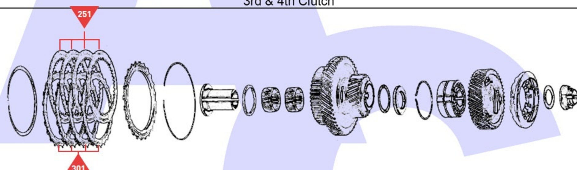
3rd & 4th Clutch
