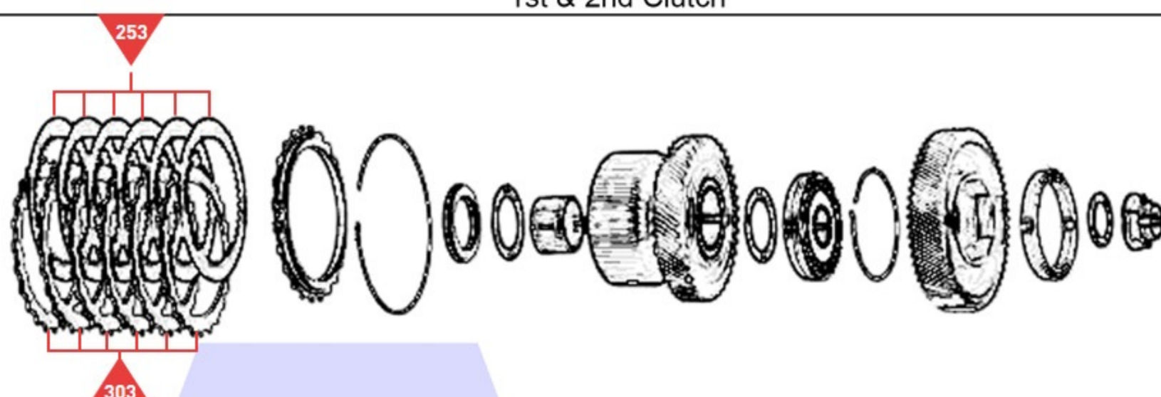
1st & 2nd Clutch
