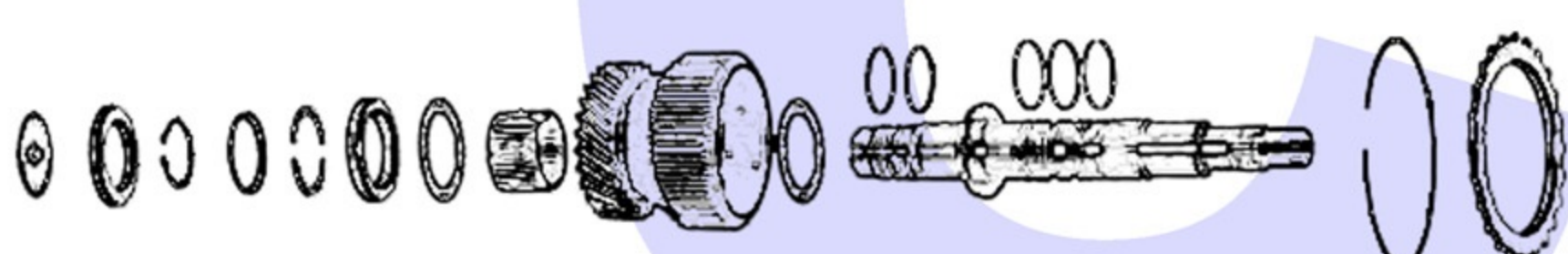
Secondary Shaft
