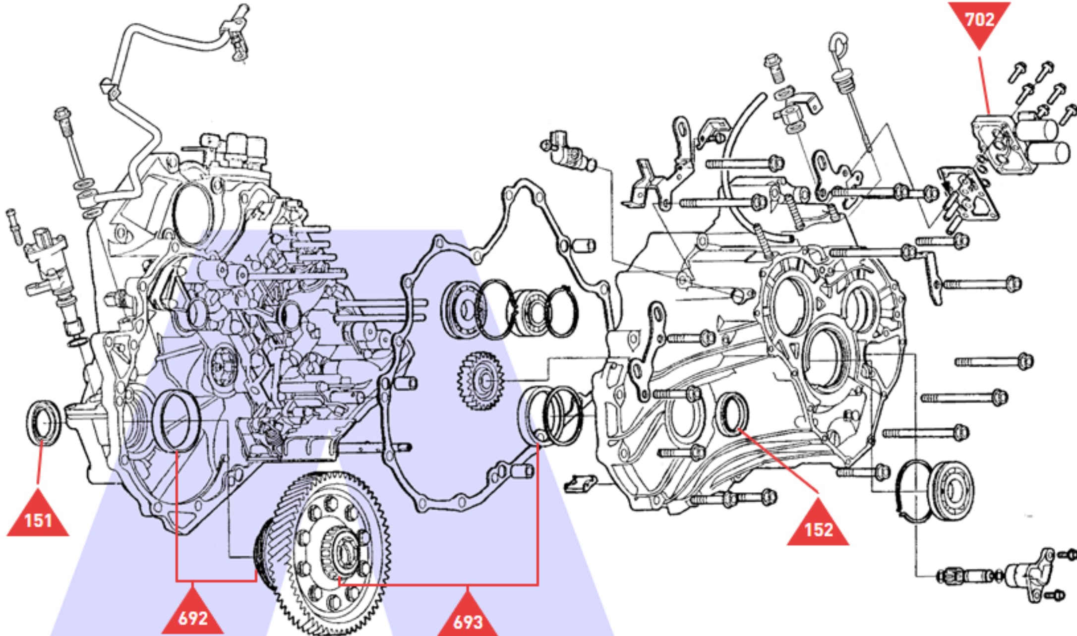
Main Casings, External Components & Diff Assy
