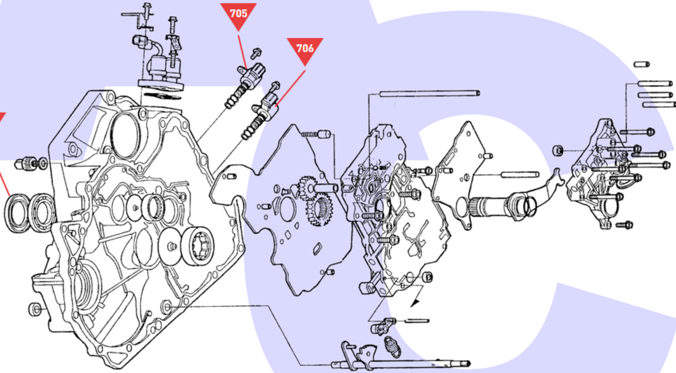
Front Housing & Main Valve Body Assembly
