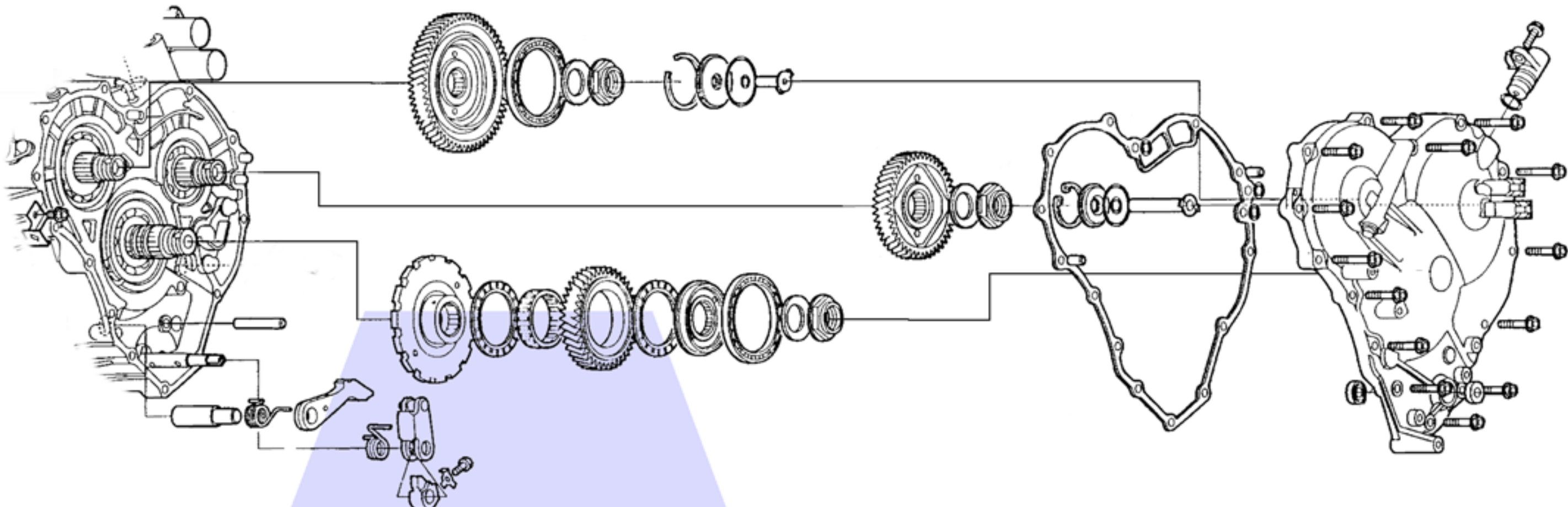
End Cover & Idler Gears
