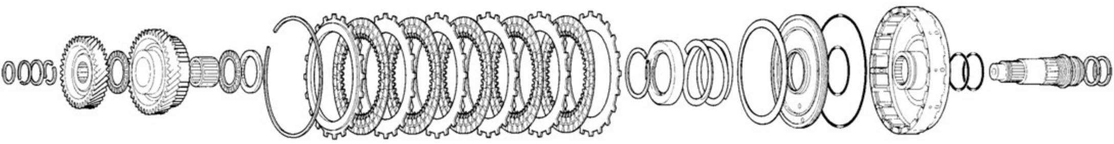
Intermediary Shaft & Third Clutch
