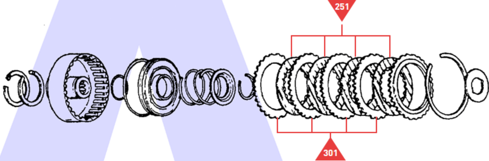
High Clutch
