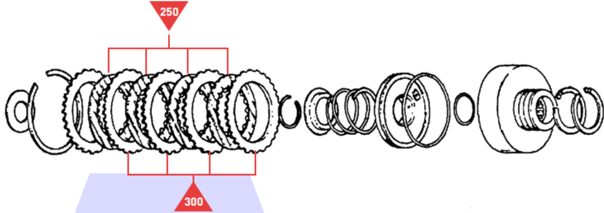
Low Clutch
