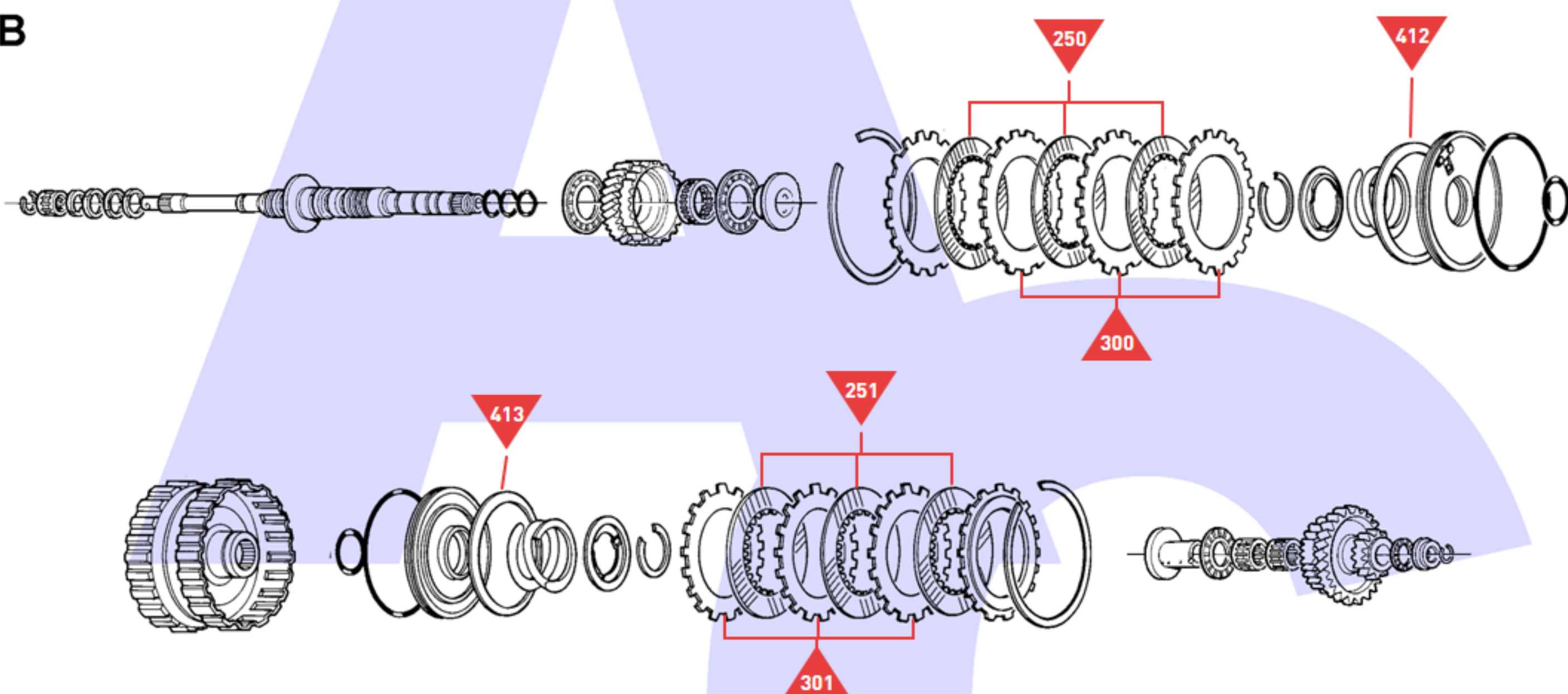
Third & Fourth Clutches
