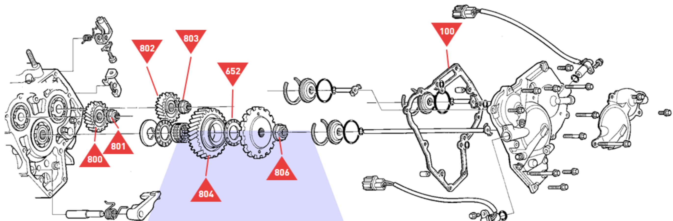
End Cover & Output Gears
