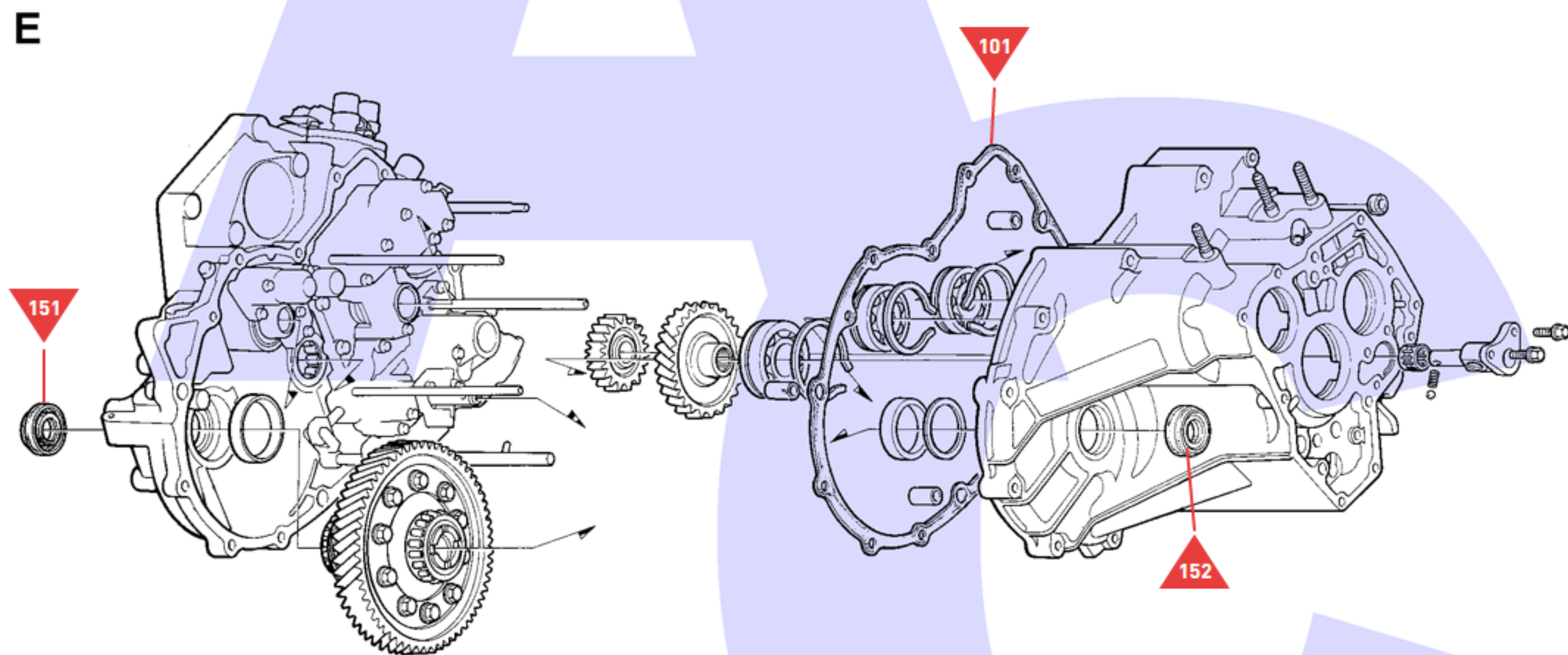
Main Casings & Differential
