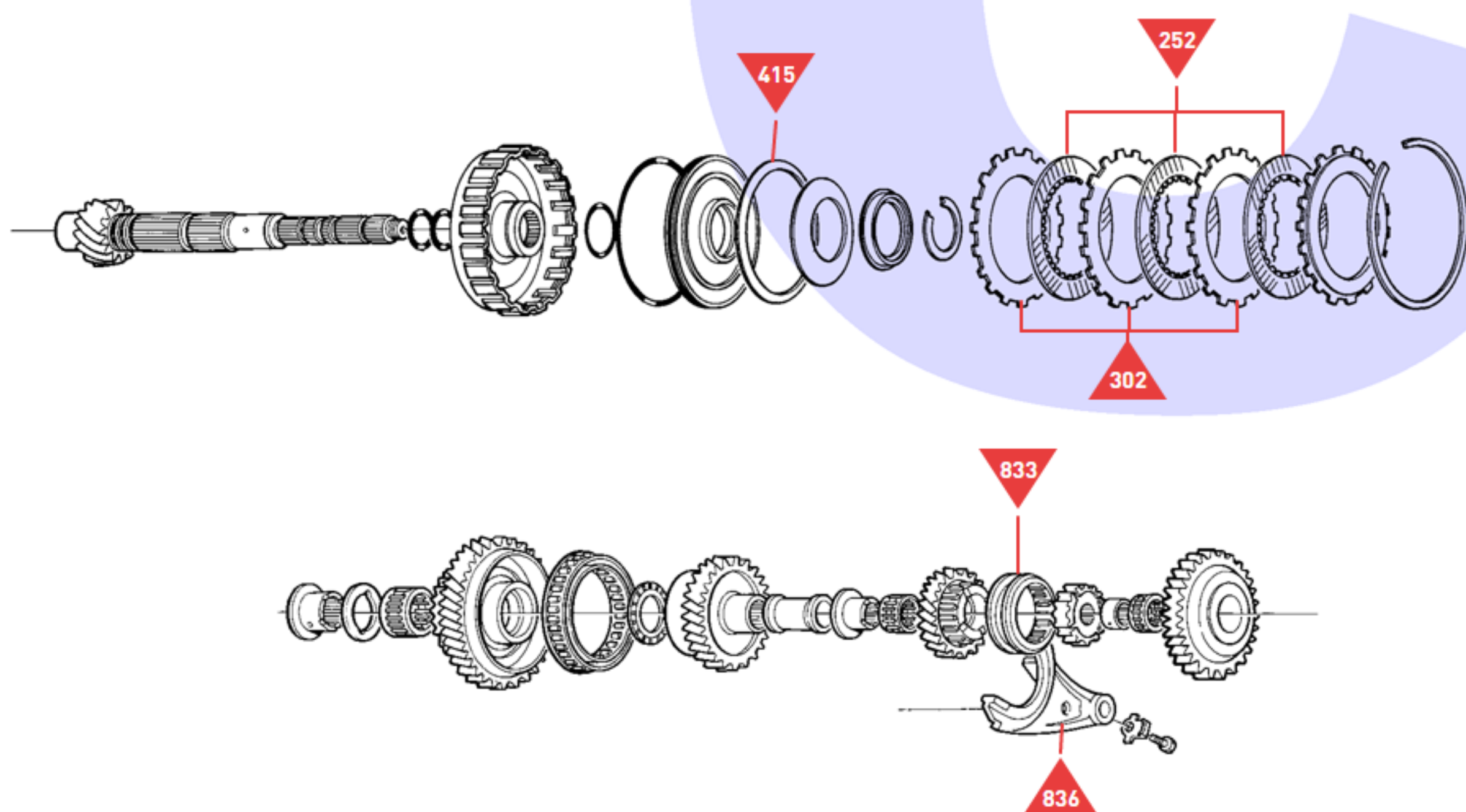
First Hold Clutch
