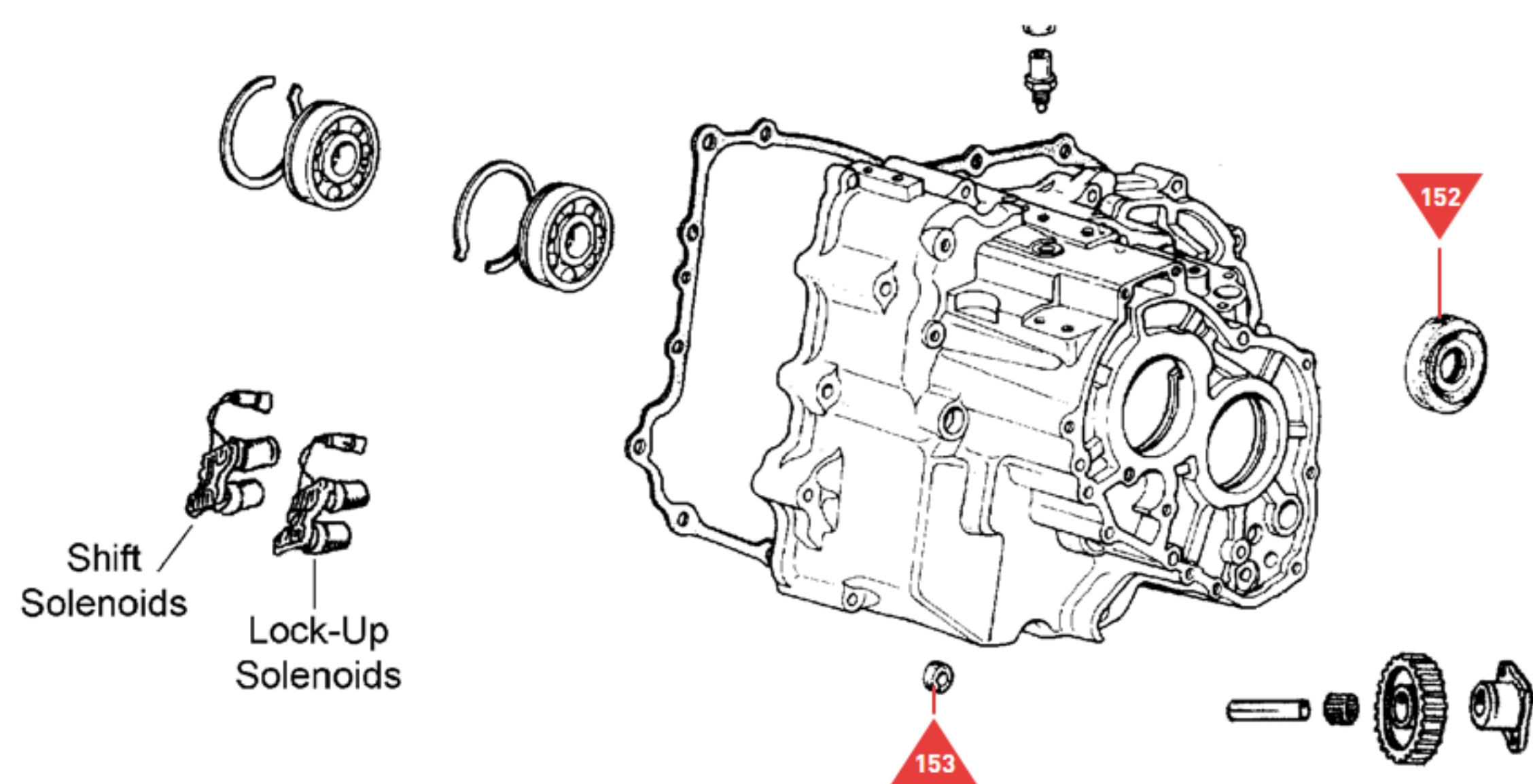
Transmission Housing
