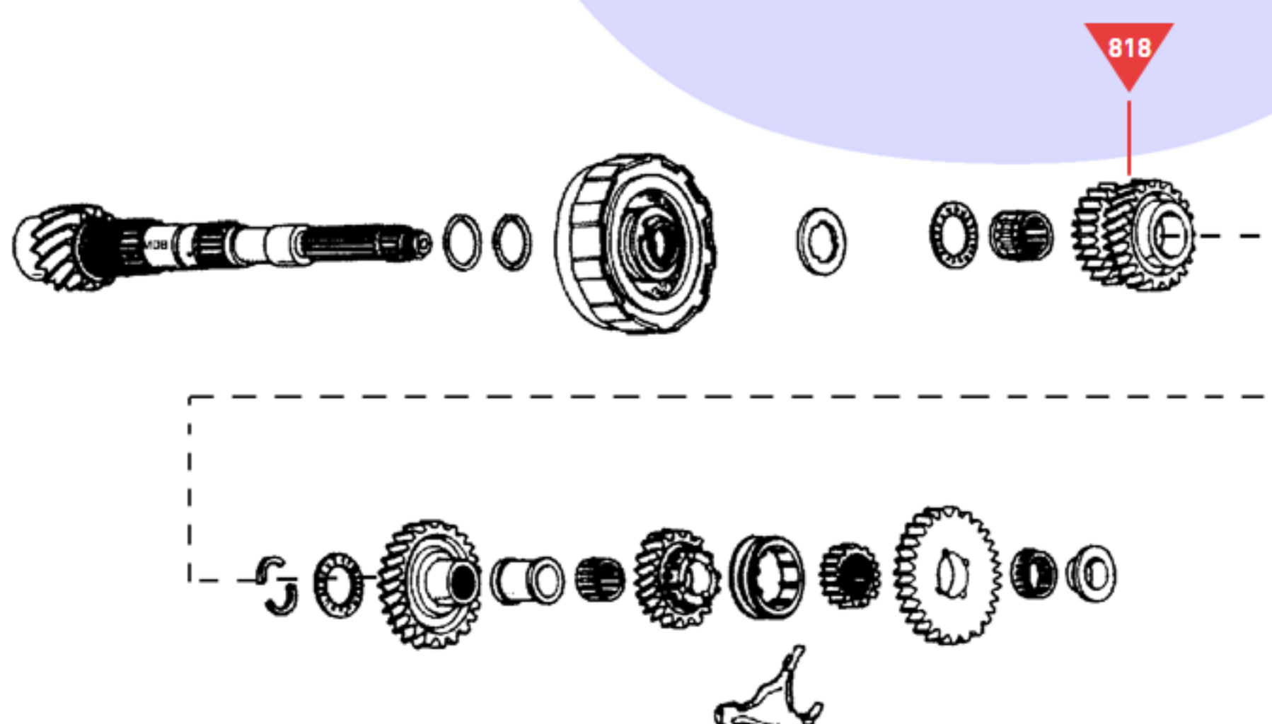
Countershaft
