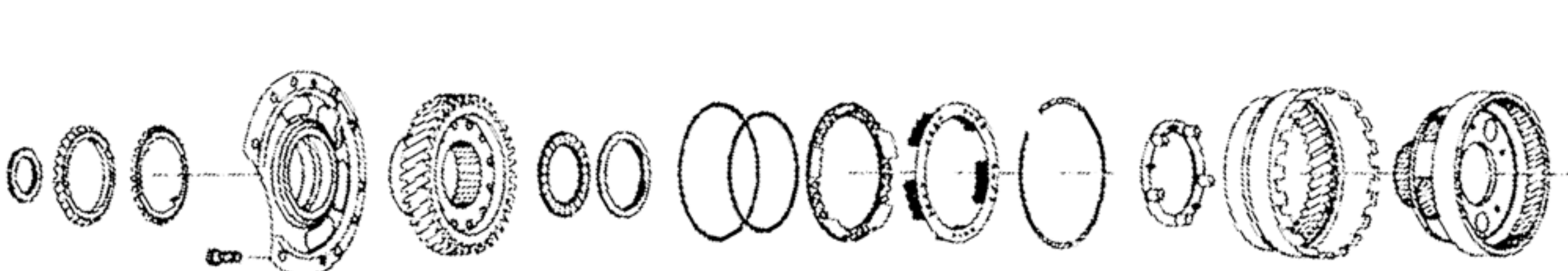
Output Drive Gear
