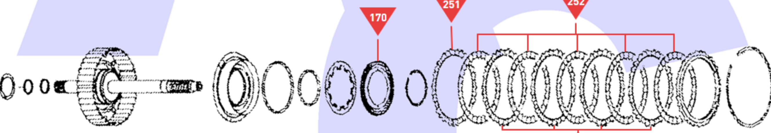
3-5-R Clutch Assembly
