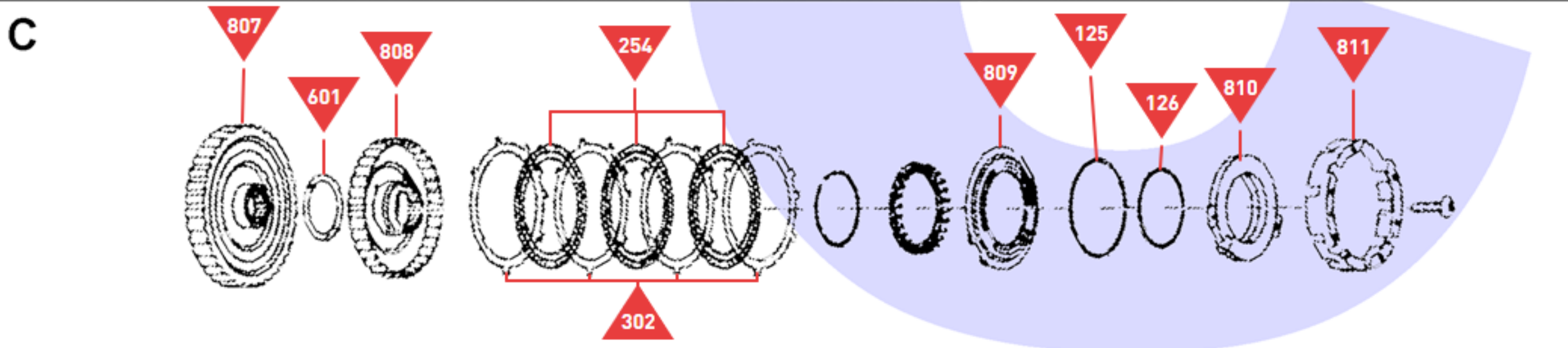
Underdrive Brake Assembly
