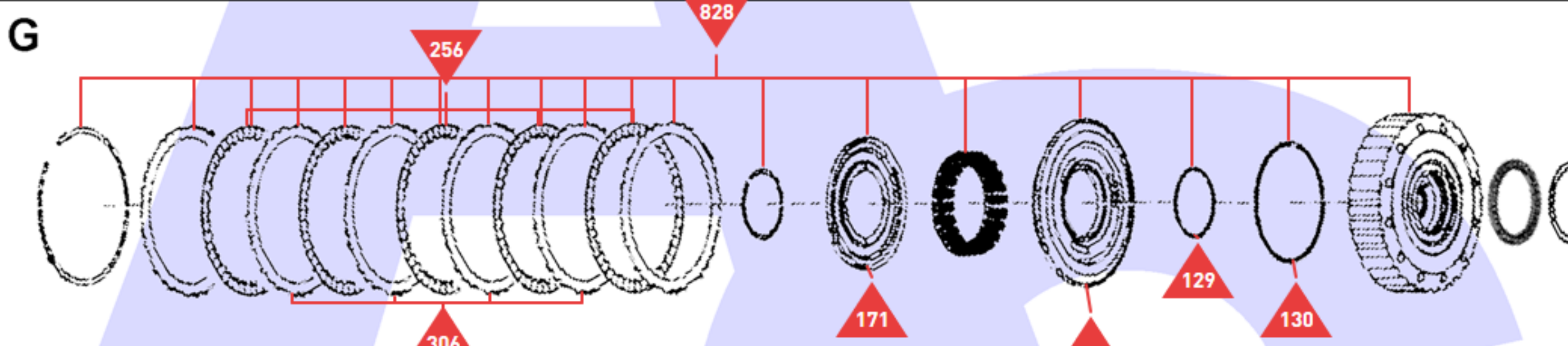
Overdrive Clutch Assembly
