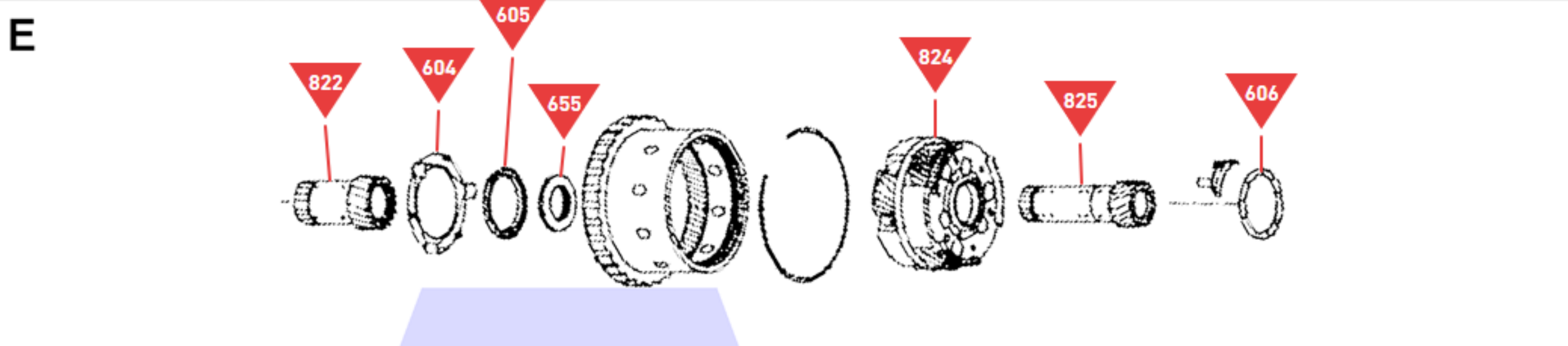
Front Sun Gear, Mid & Rear Planet, Sun Gear
