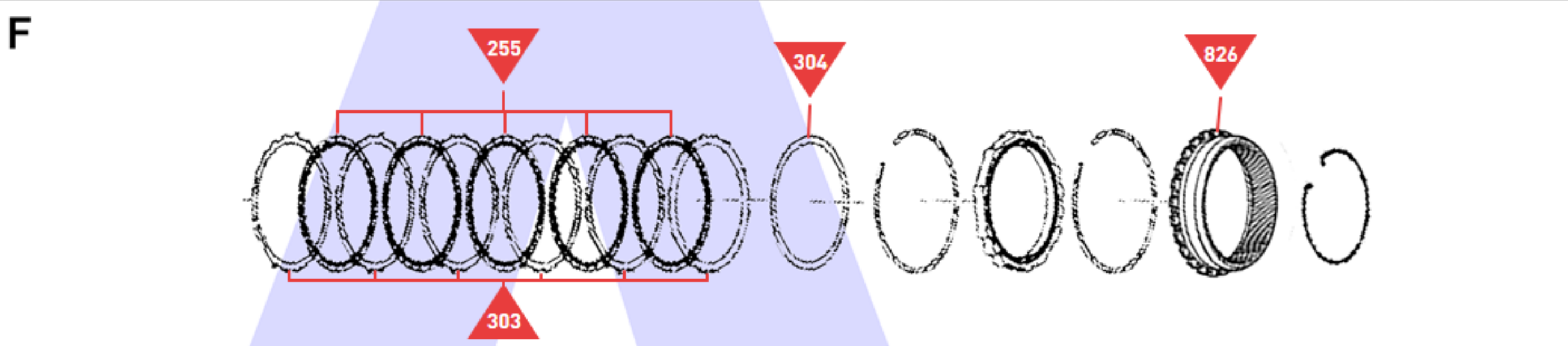
Low & Reverse Brake, One Way Clutch & Inner Race
