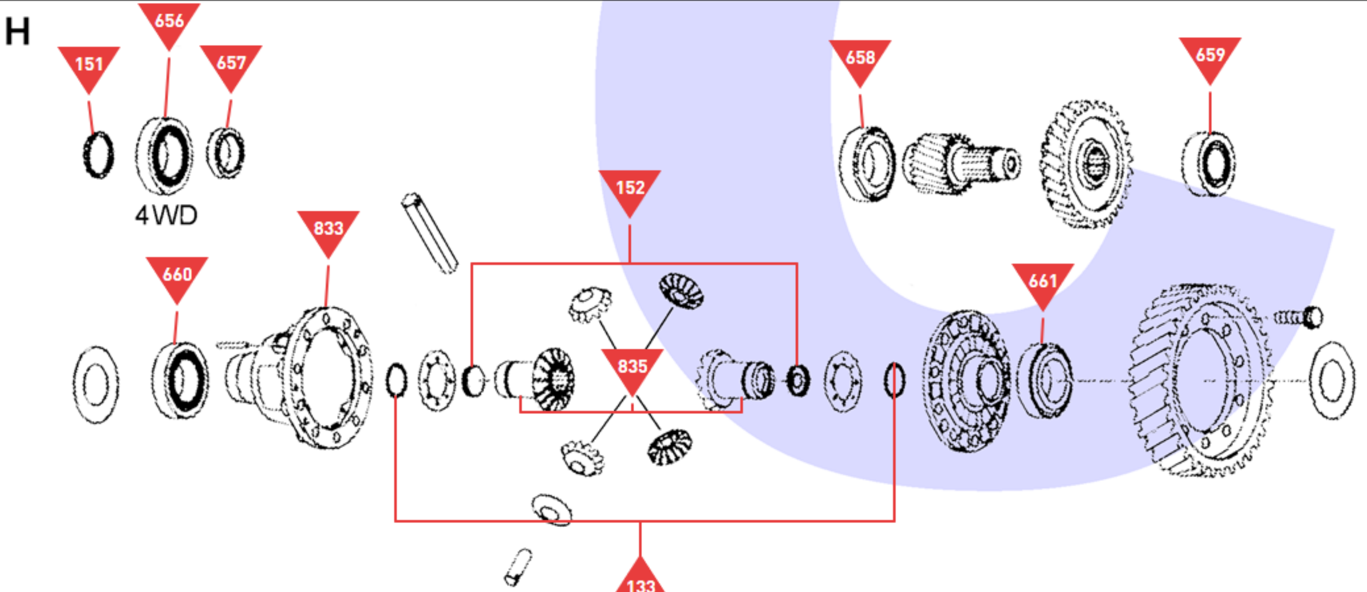
Transfer Gear & Differential Assembly
