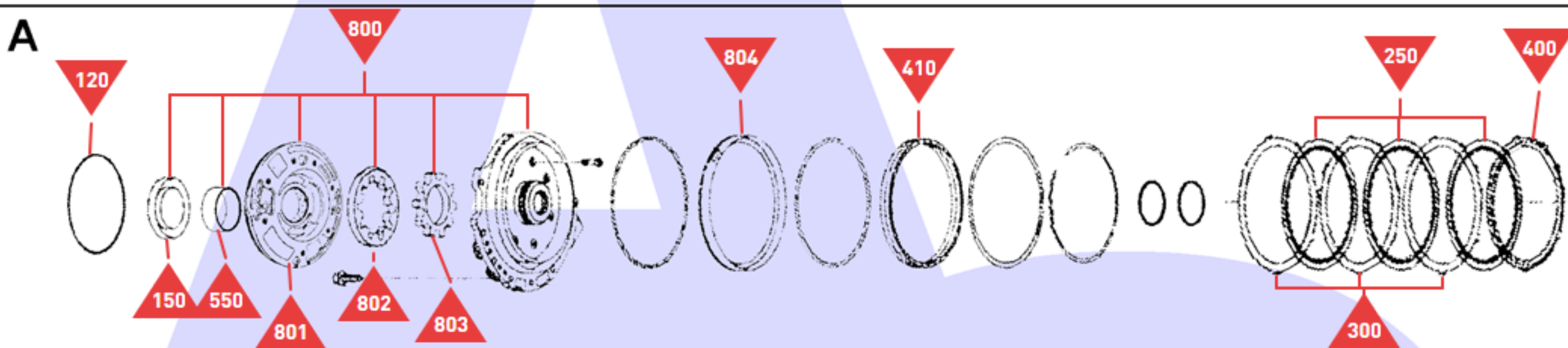
Pump Assembly
