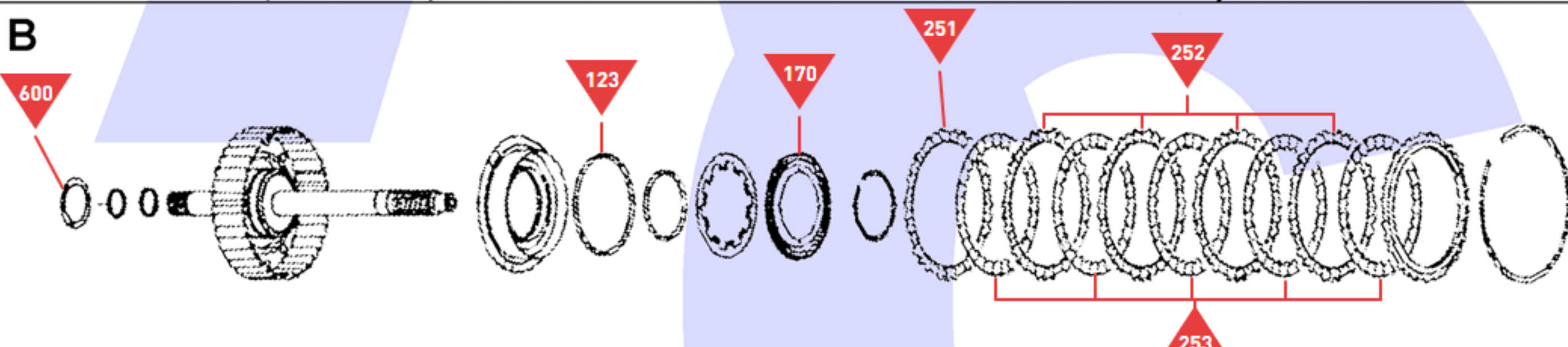
3-5-R Clutch Assembly
