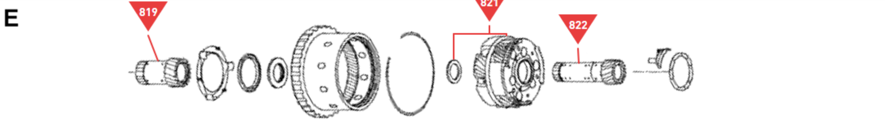
Front Sun Gear, Mid & Rear Planet, Sun Gear
