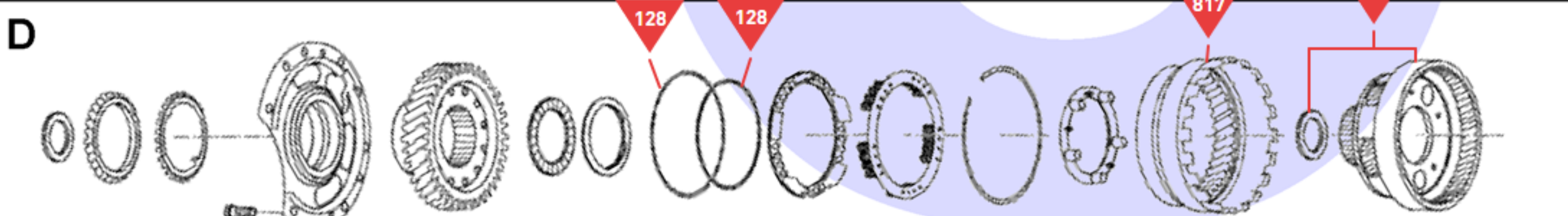
Output Drive Gear
