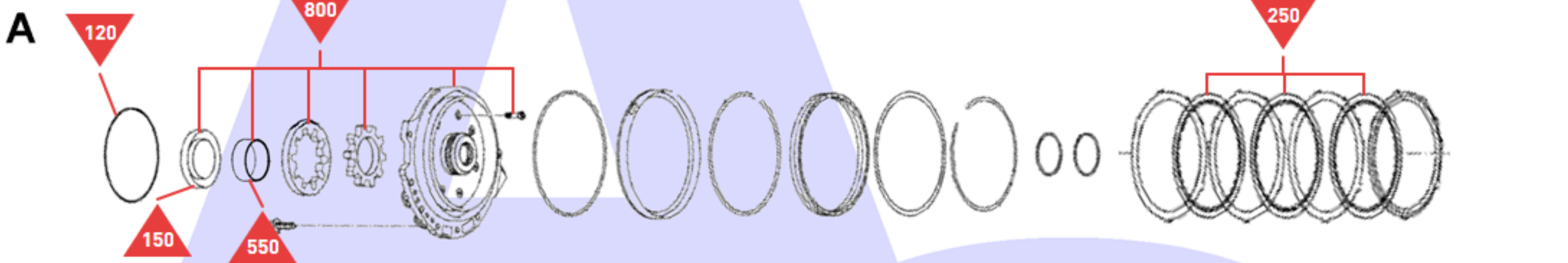
Pump Assembly
