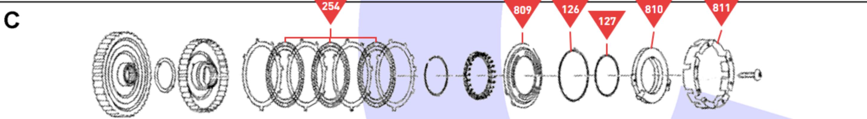
Underdrive Brake Assembly
