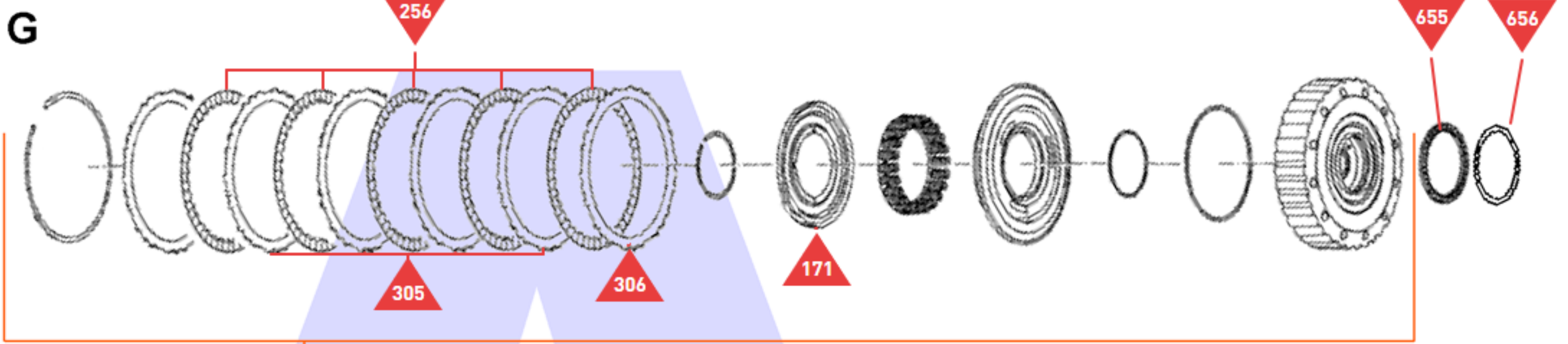
Overdrive Clutch Assembly
