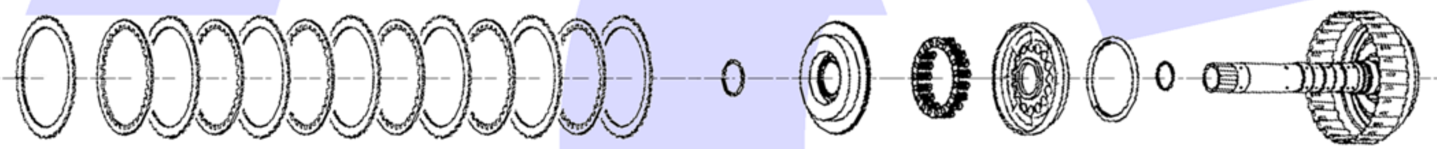
3-5/Reverse Shell, 3-5/Reverse Planet & Underdrive Clutch Assembly
