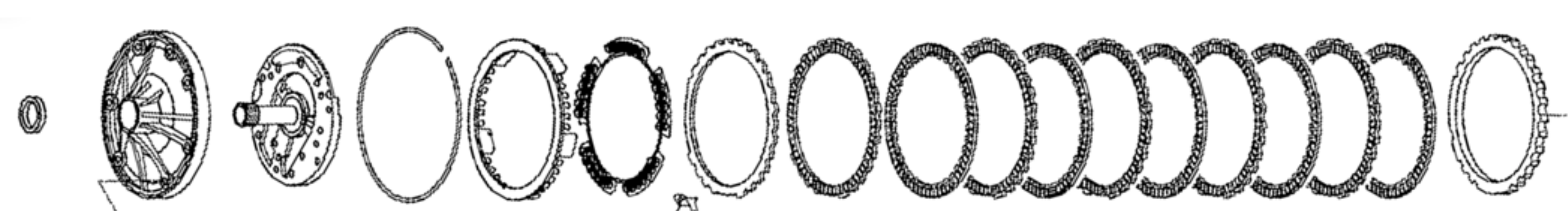
Oil Pump & 8th - Low - Reverse Brake
