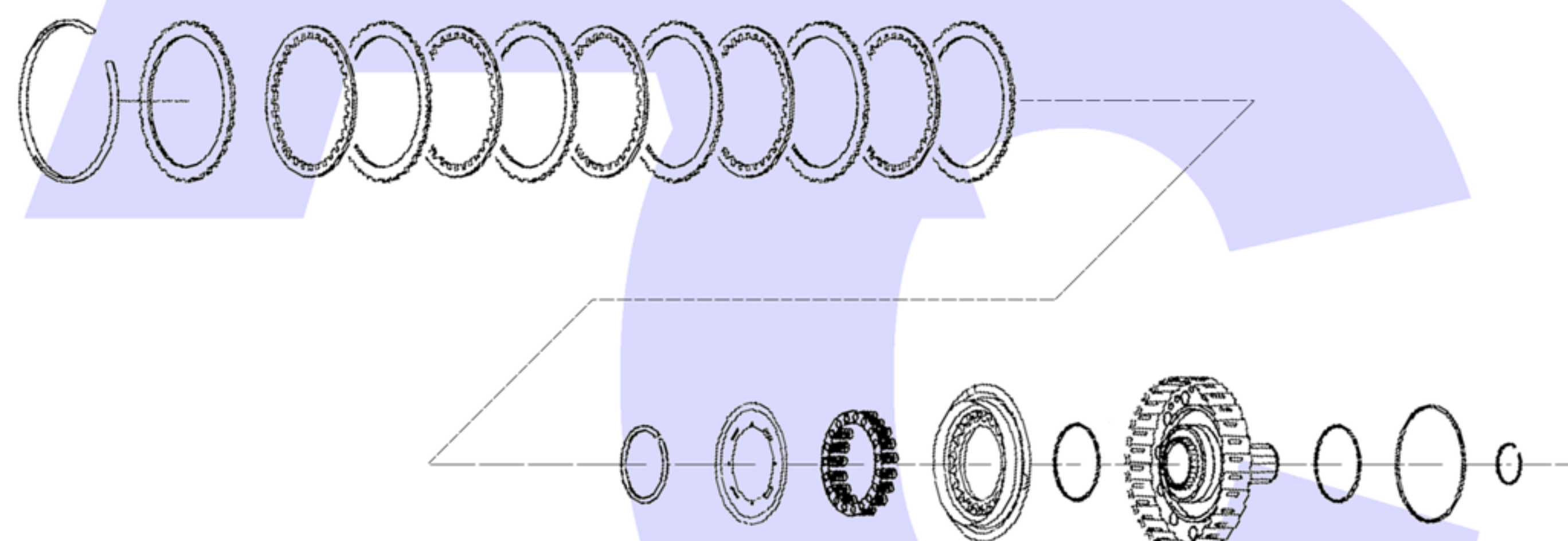
6th Clutch Assenbly
