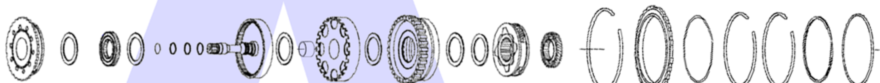
Overdrive Planet, Overdrive Ring Gear, 6th Sun Gear & Low Reverse Ring Gear
