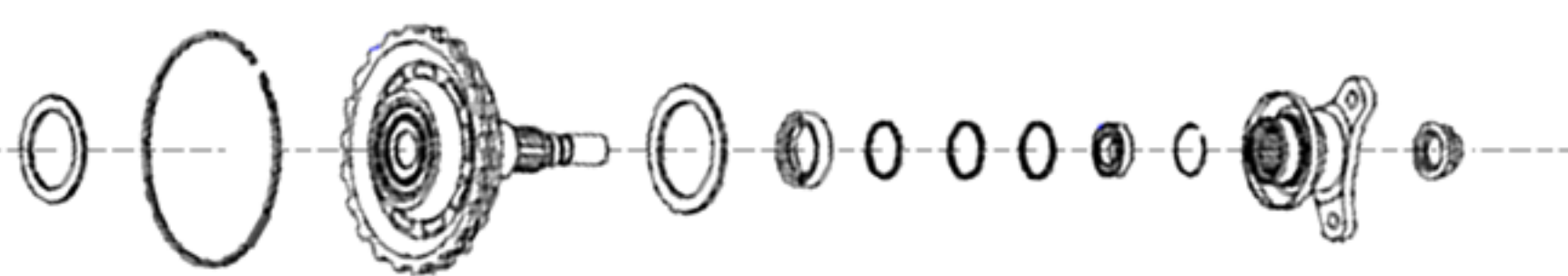
4th Clutch Hub, 4th Clutch Assembly & Output Shaft
