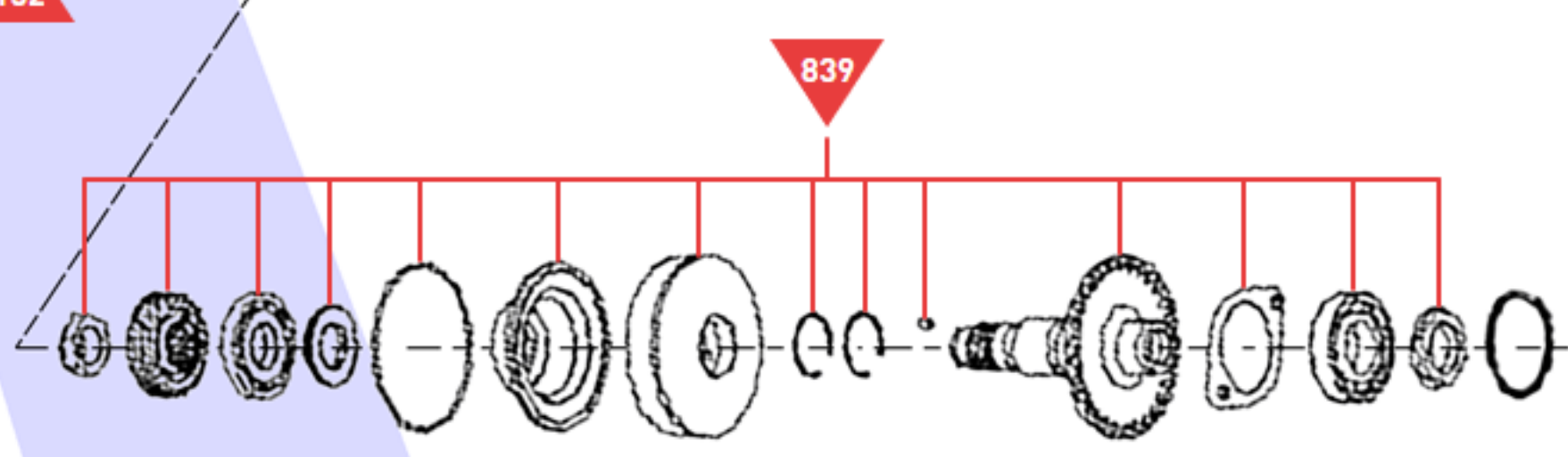
Primary Pulley
