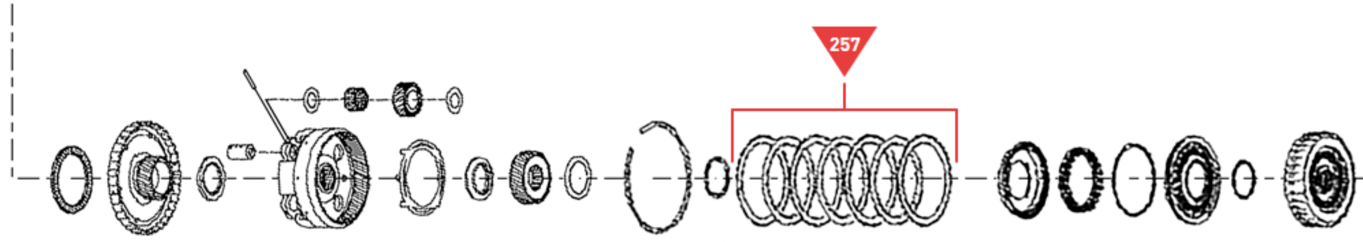
Forward Clutch
