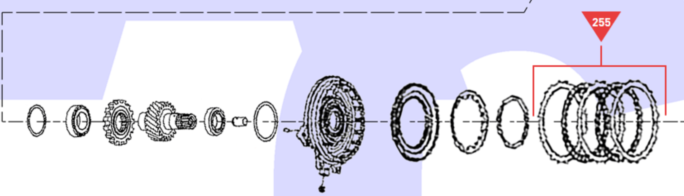
Underdrive Brake
