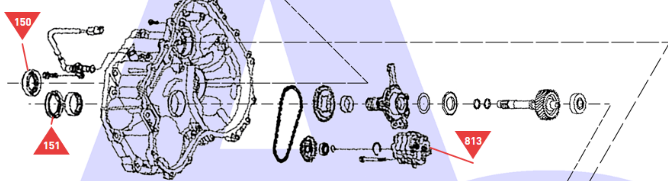
Oil Pump, Drive Chain Stator & Input Shaft
