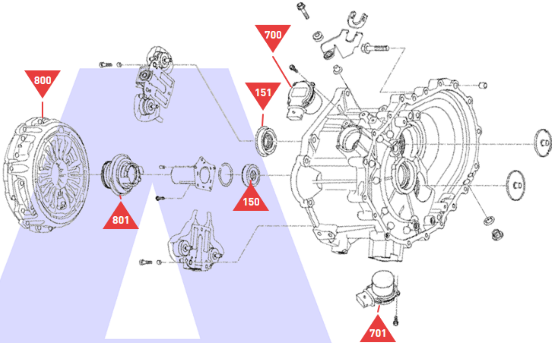
Clutch, Clutch Control and Bell Housing
