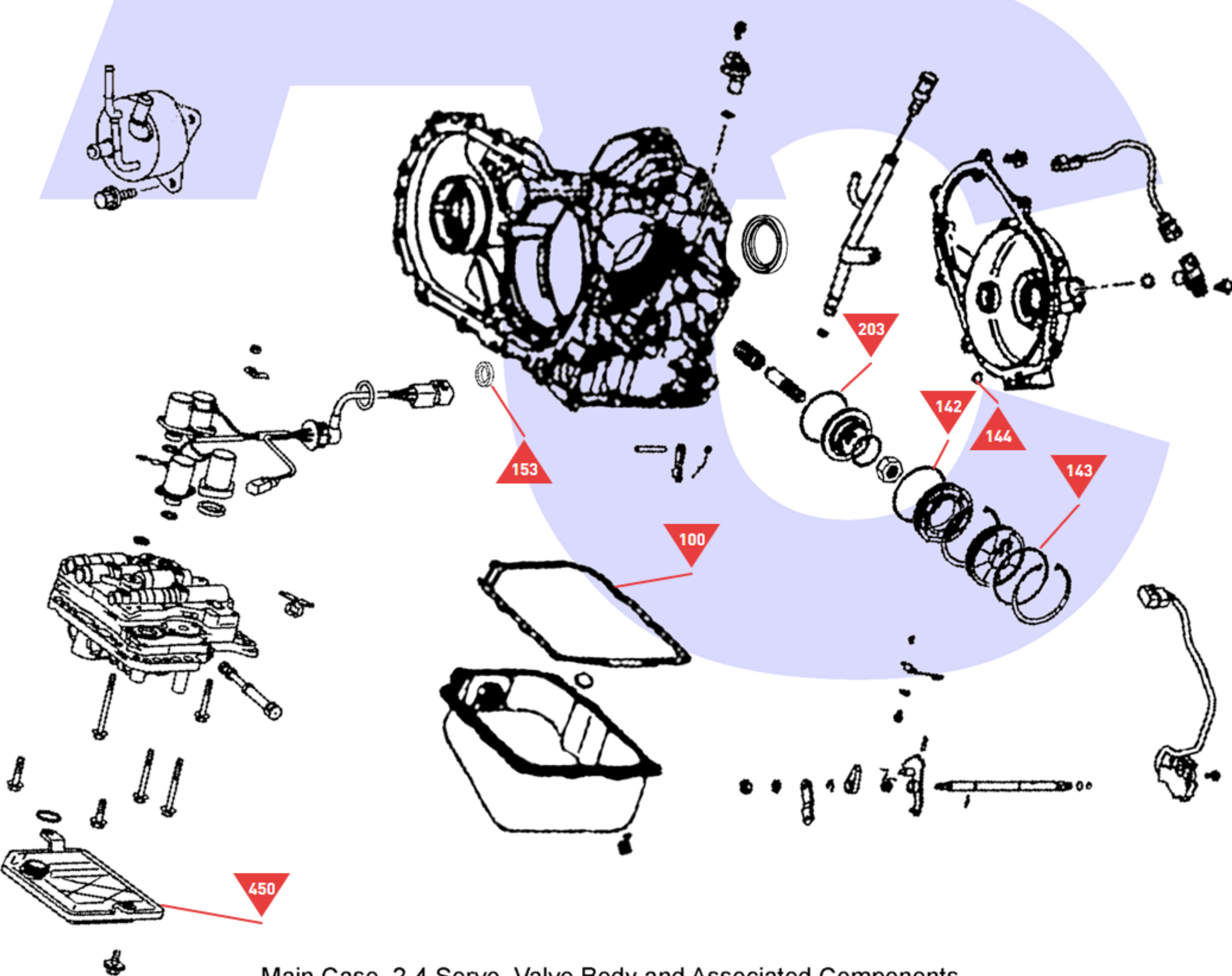
Main Case, 2-4 Servo, Valve Body and Associated Components
