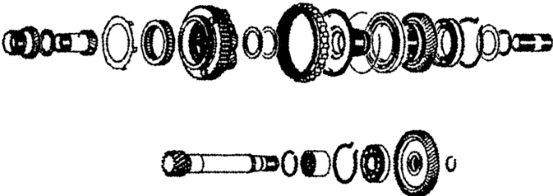
Sun Gears, One-Way-Clutch, Planetary, Transfer Gears and Pinion Shaft
