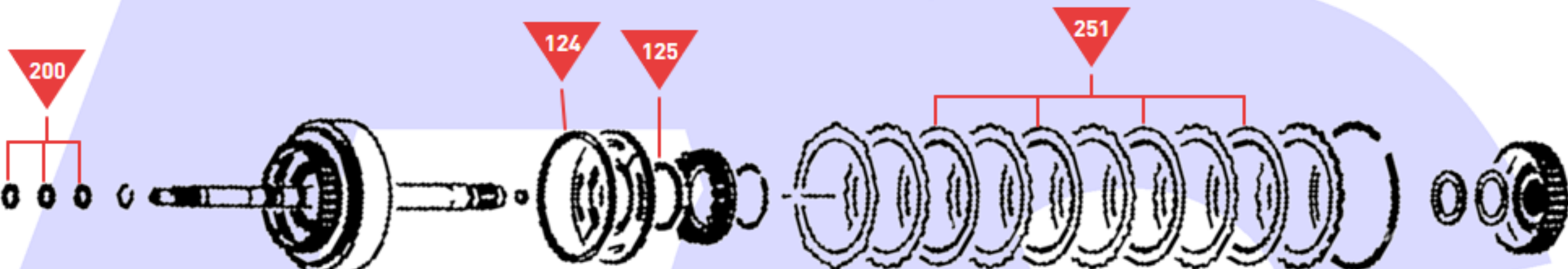
Front (Direct) Clutch
