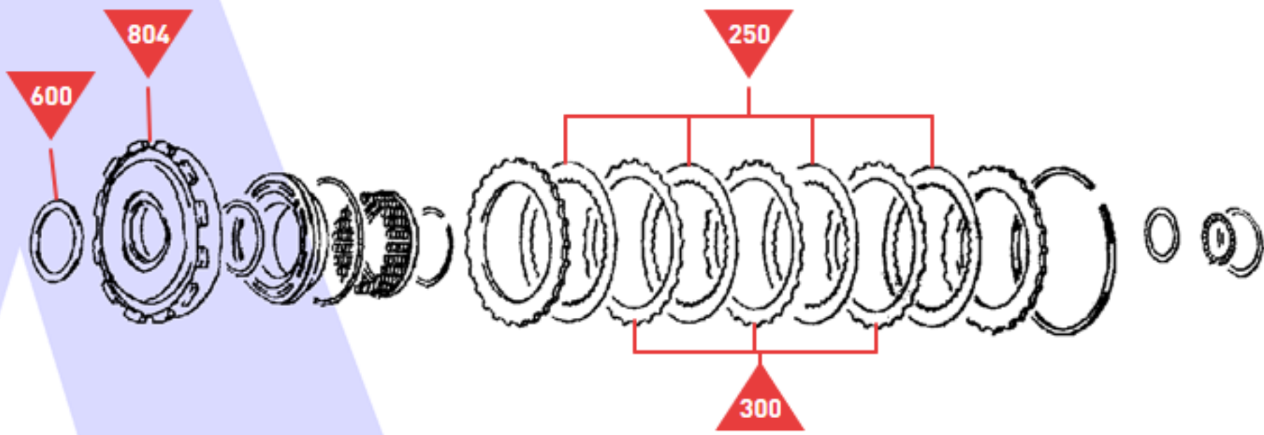
Oil Pump & Direct Clutch
