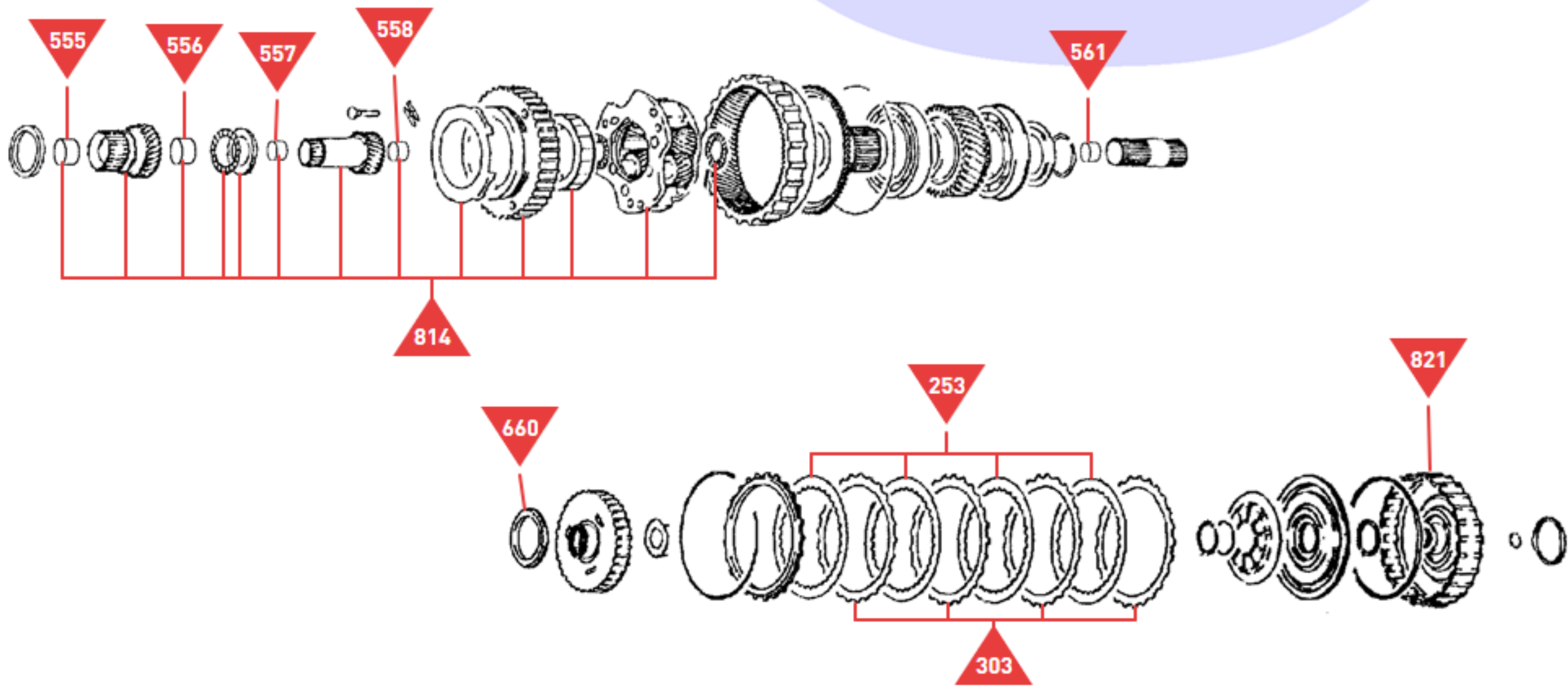
Planetary Set & Overdrive Clutch
