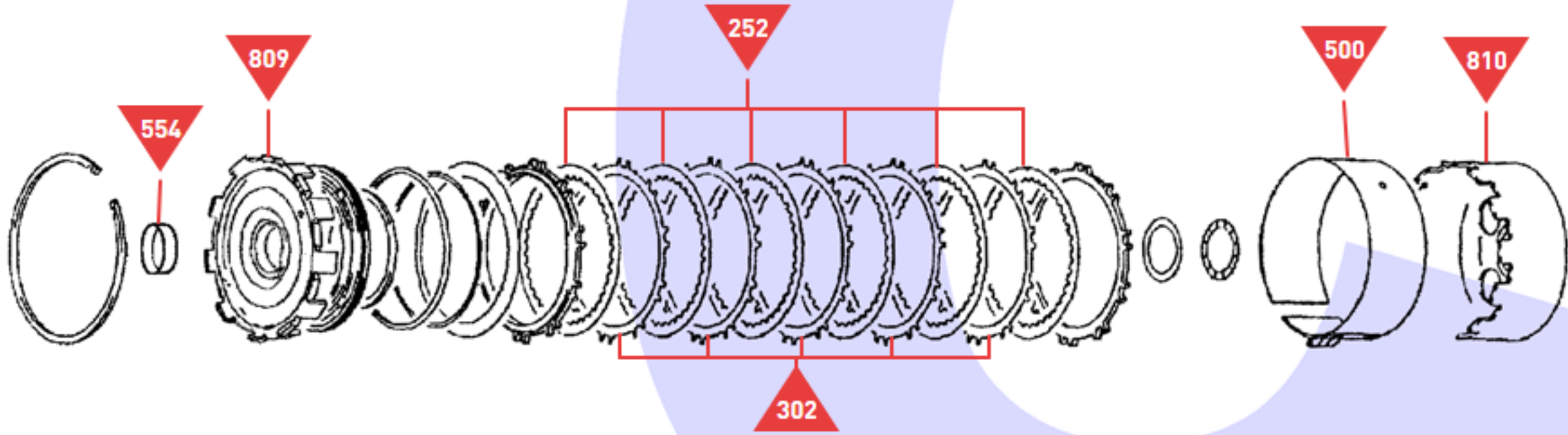
Low Reverse Brake
