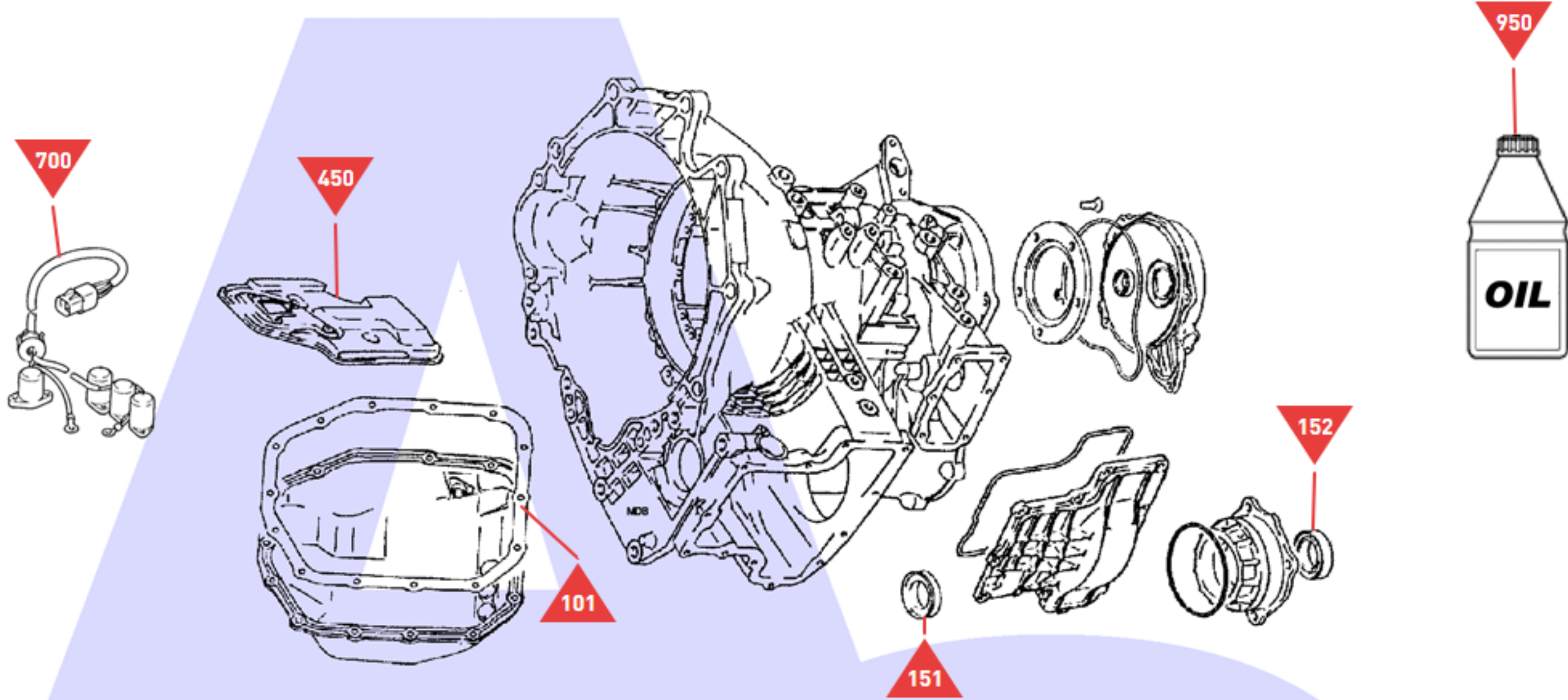
Casings, Oil Pan Etc.
