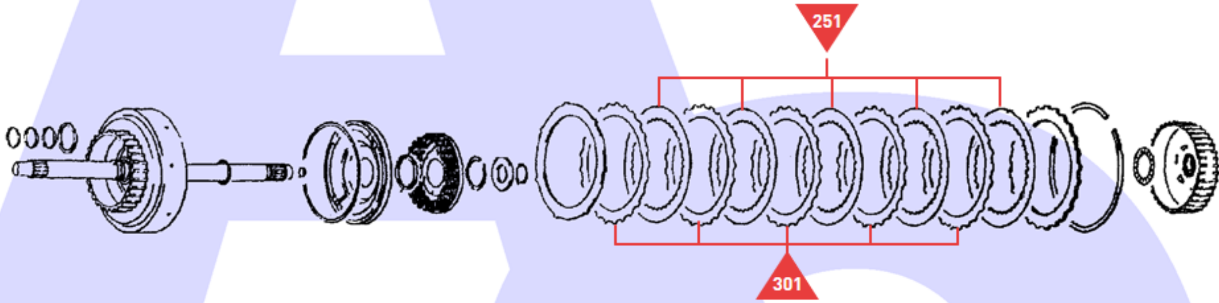
Forward Clutch
