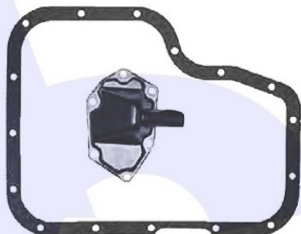
JATCO F3A Pan Gasket F3A.GAS01 Filter F3A.FIL03 40mm Pipe
