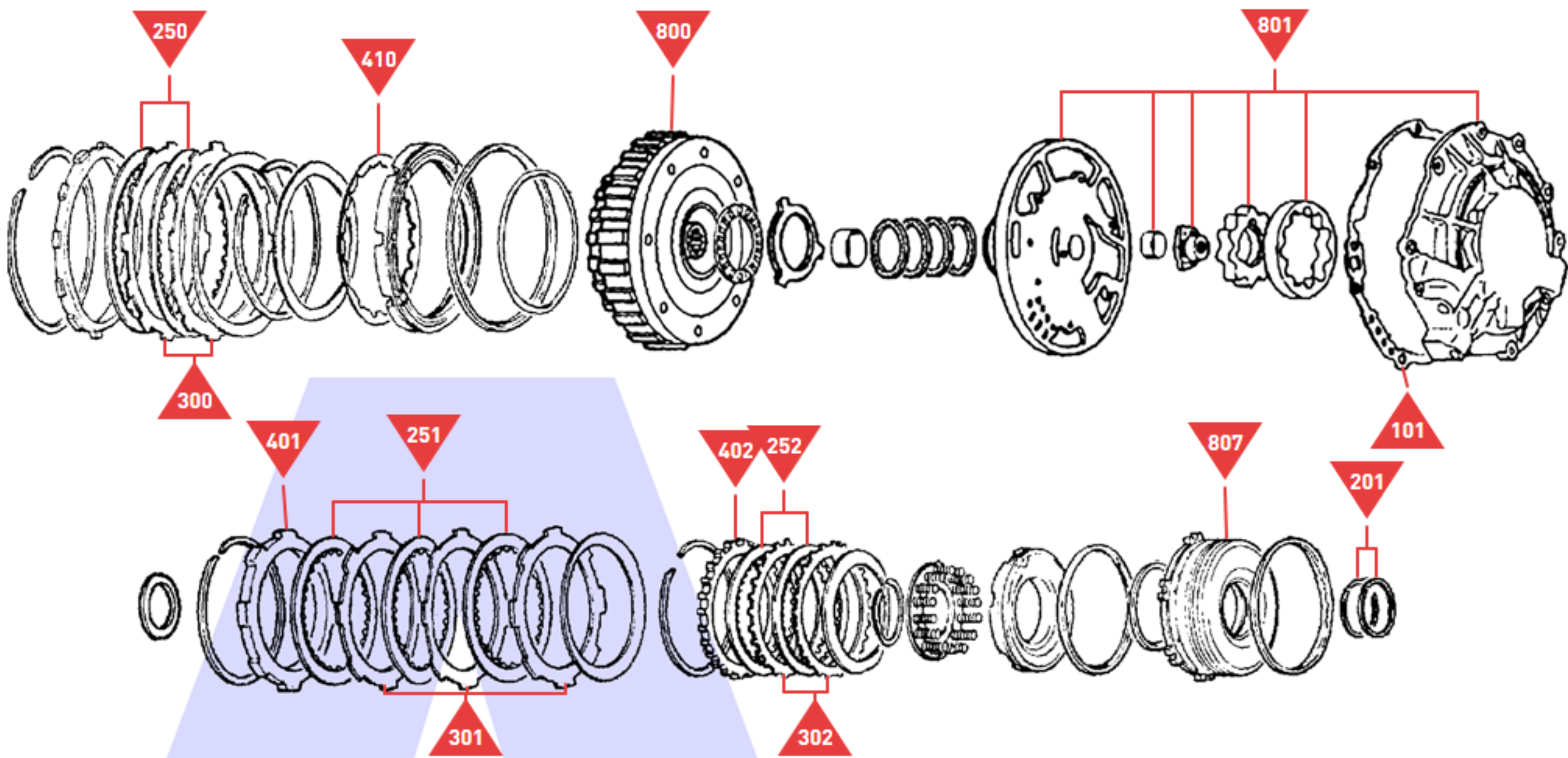
Reverse, Forward and Coast Clutches
