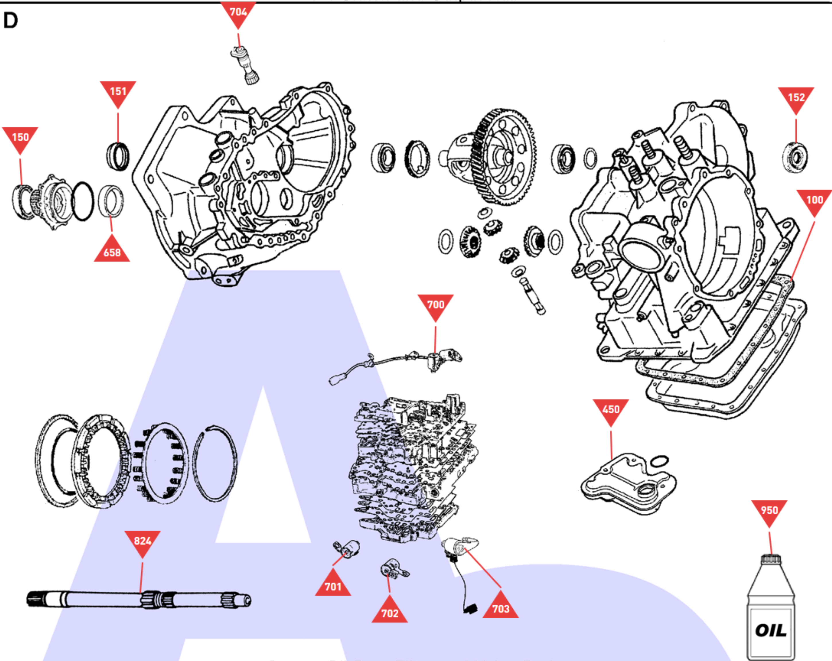
Cases, Oil Pan, Filter and Valve Body
