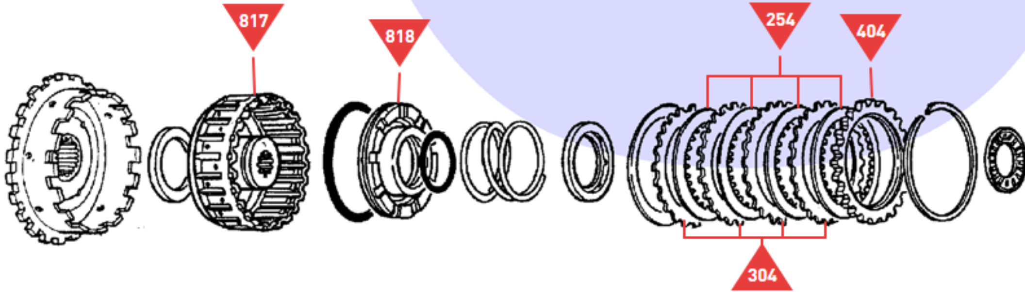
3-4 Clutch and Output Hub
