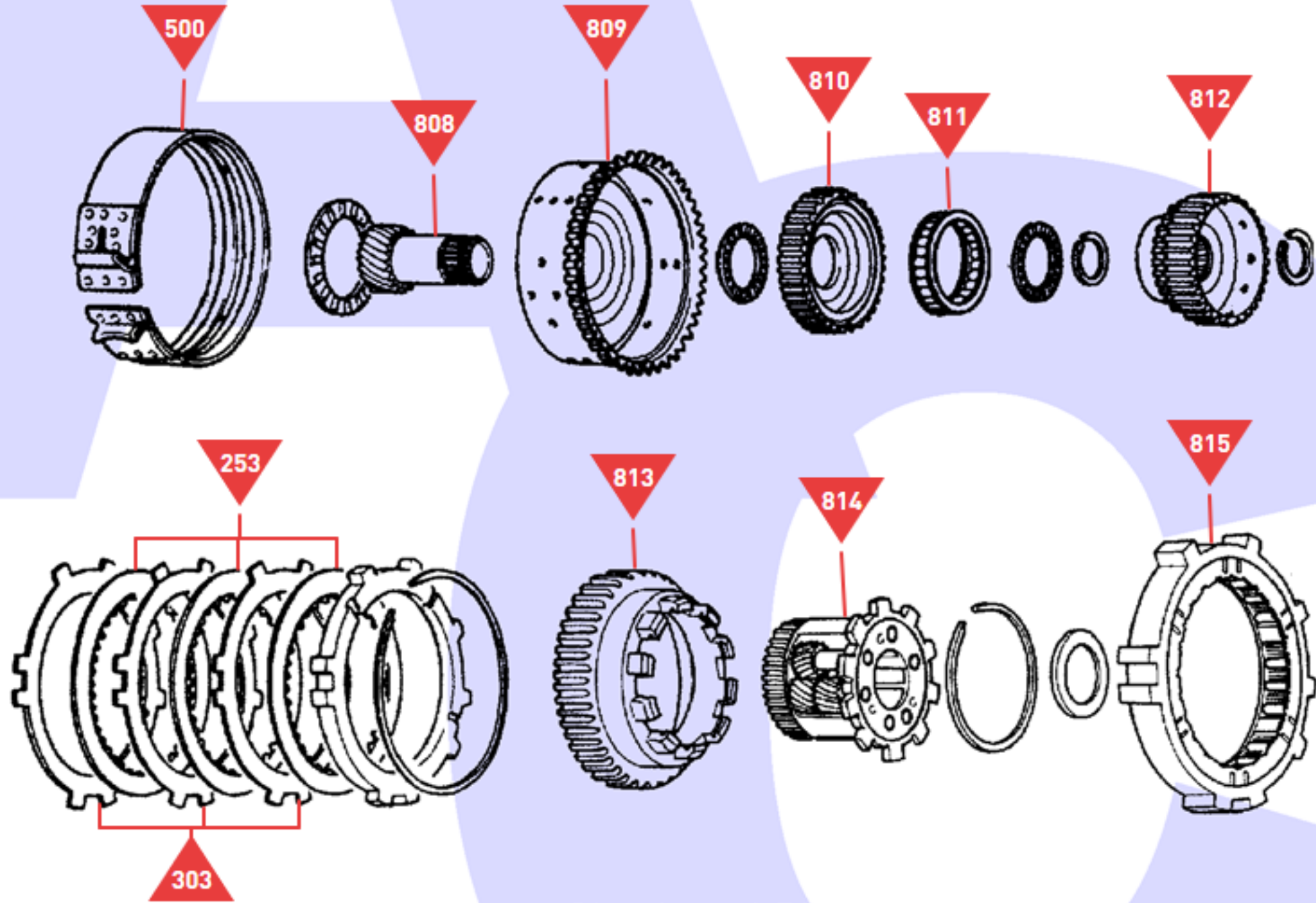
Low Reverse Clutch and Planetary Set
