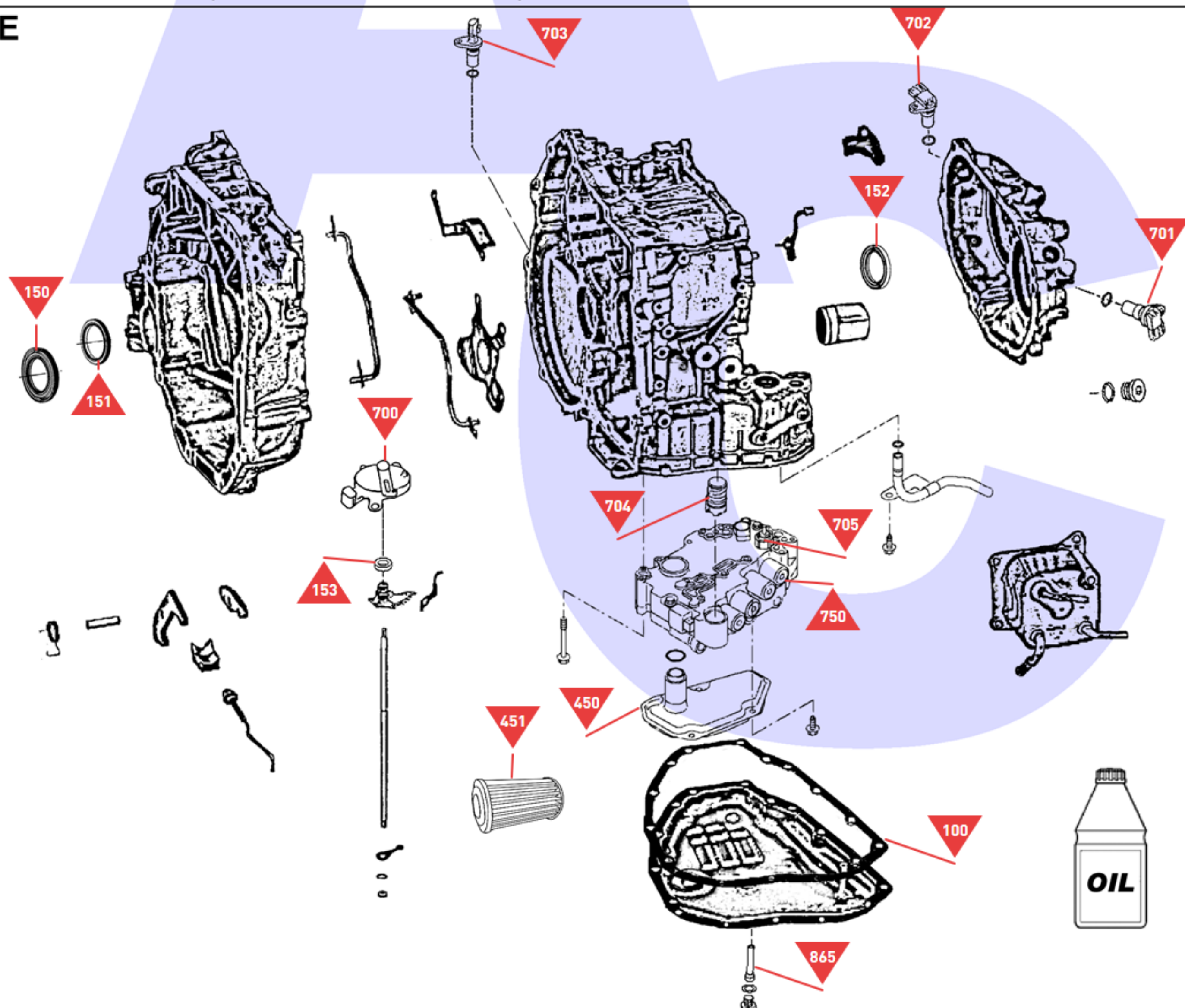
Casings, Valve Body, Filters and External Items Etc.
