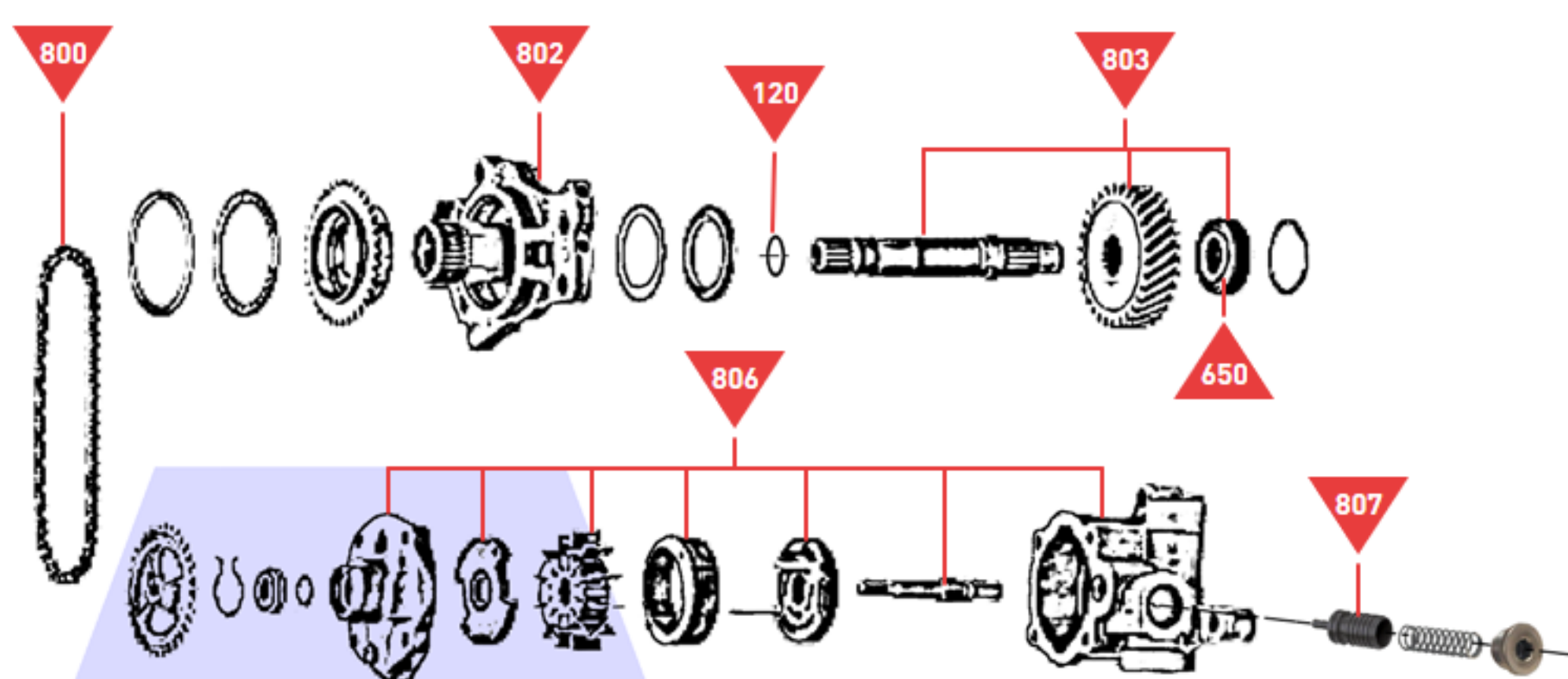
Input Shaft and Oil Pump Assy
