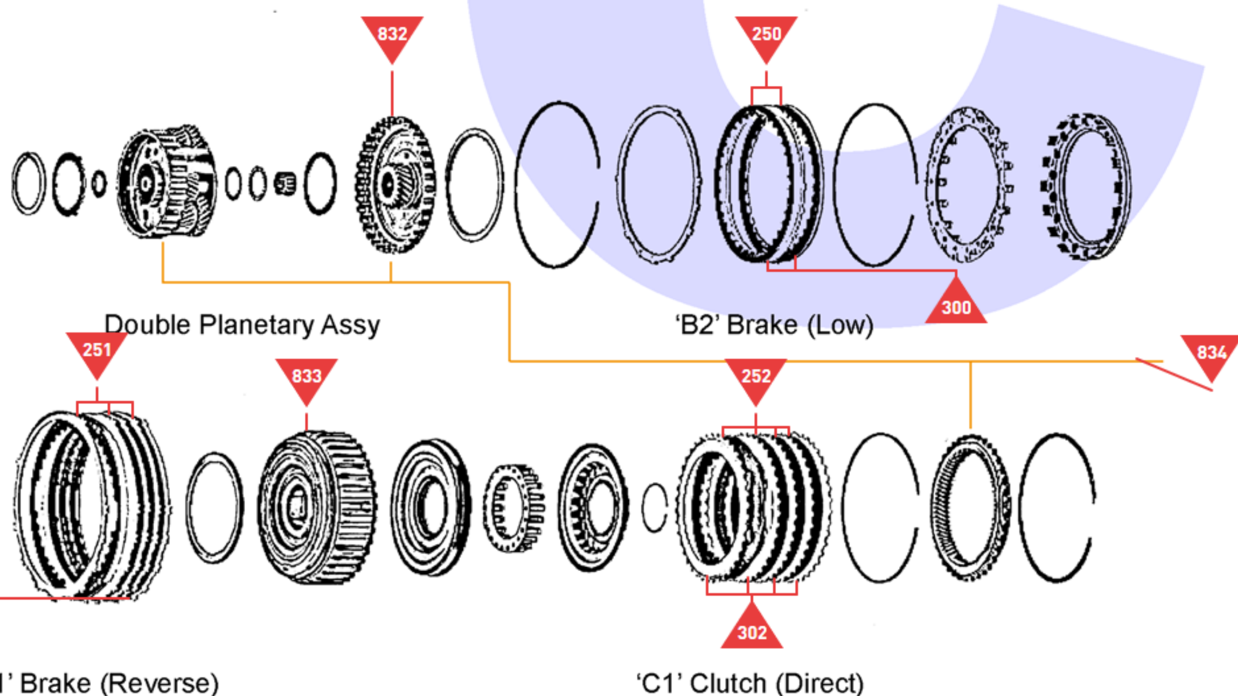
Primary and Secondary Drums
