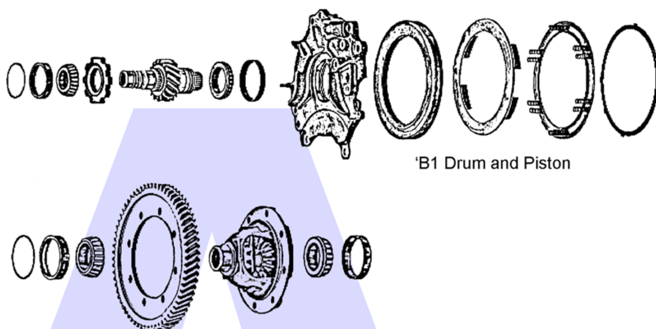
Output Gear and Differential Assy
