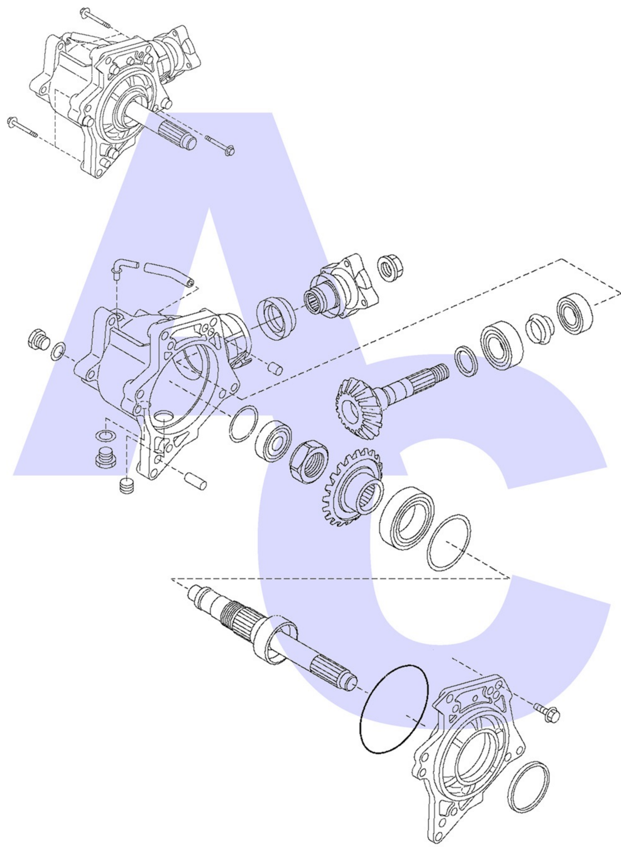
Angle Drive PTU
