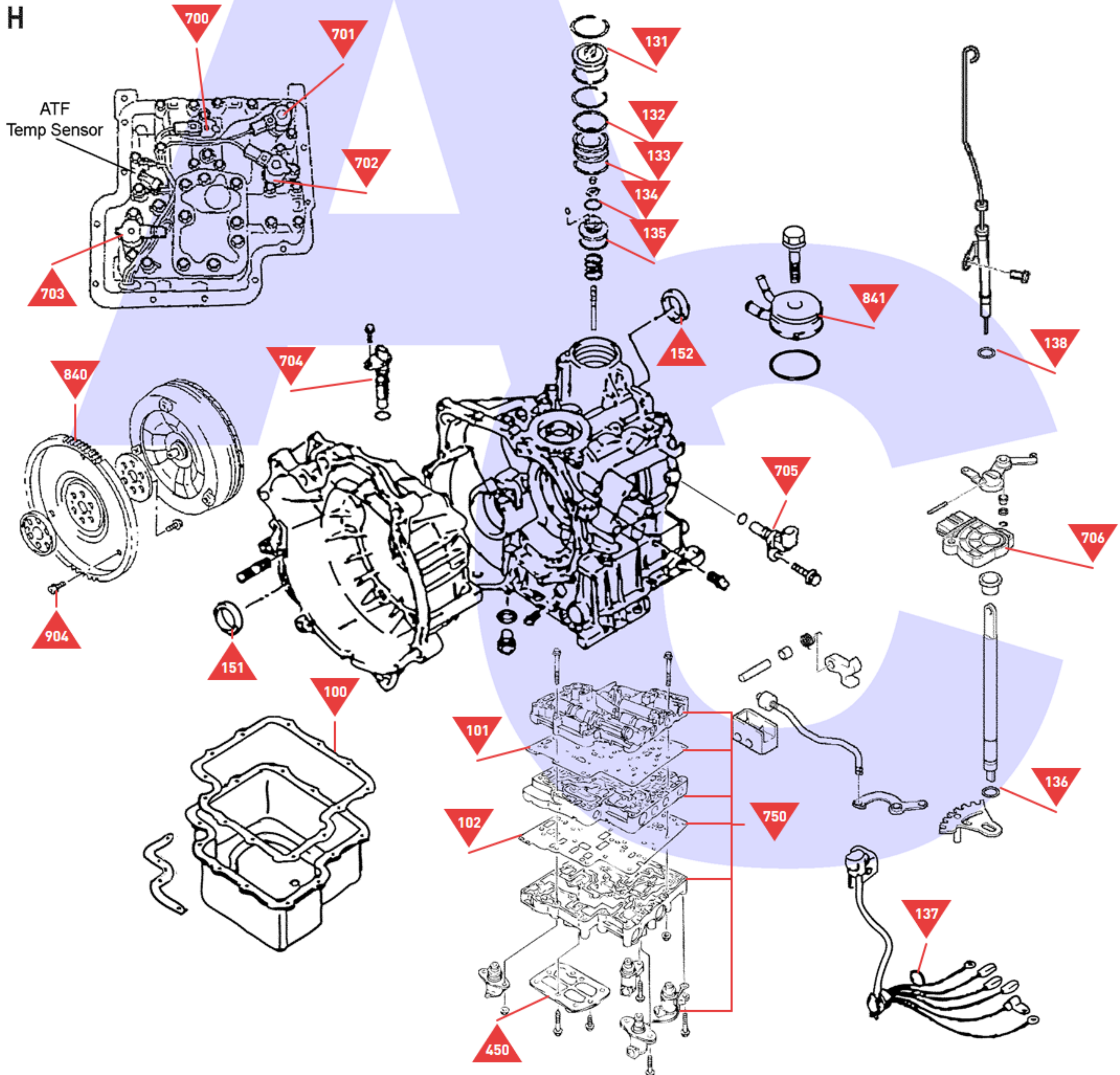
Casing, Bell Housing, Valve Body & Associated Parts
